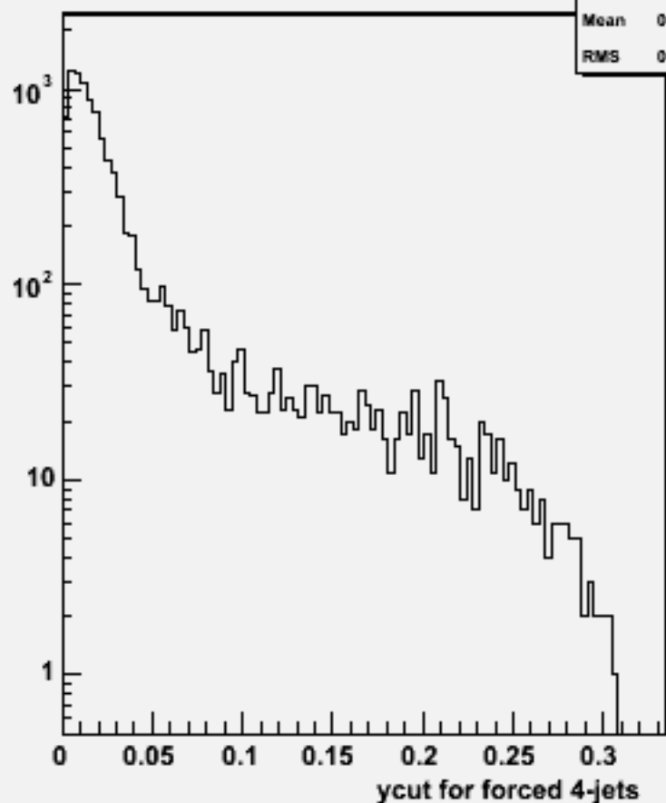
Ycut for 4-jets :w101156 ssude1n1_o
