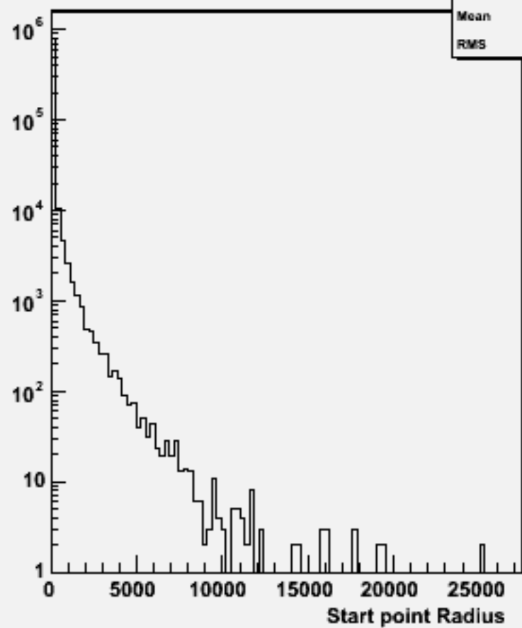
Start point R : w101156 ssude1n1_o
