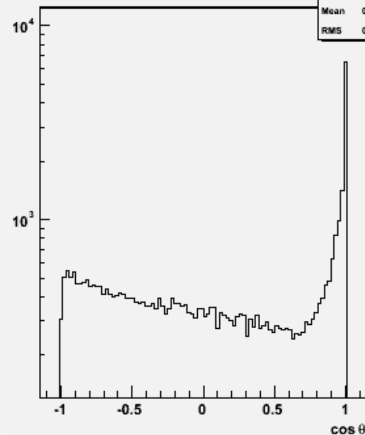
Jet cosθ (All jets)w101156 ssude1n1_o
