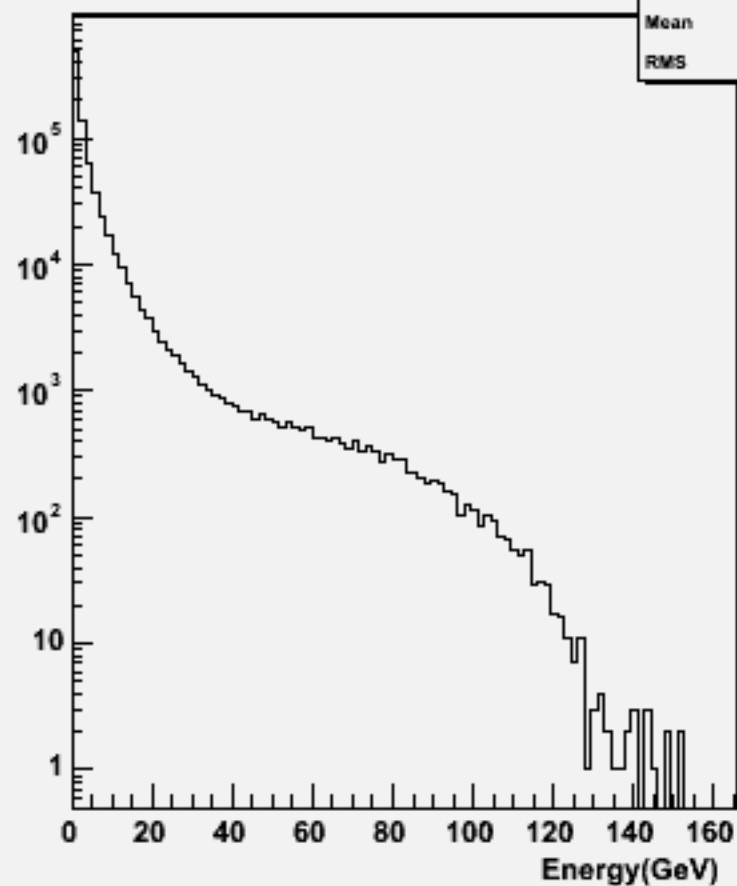
Particle Energy : w101156 ssude1n1_o
