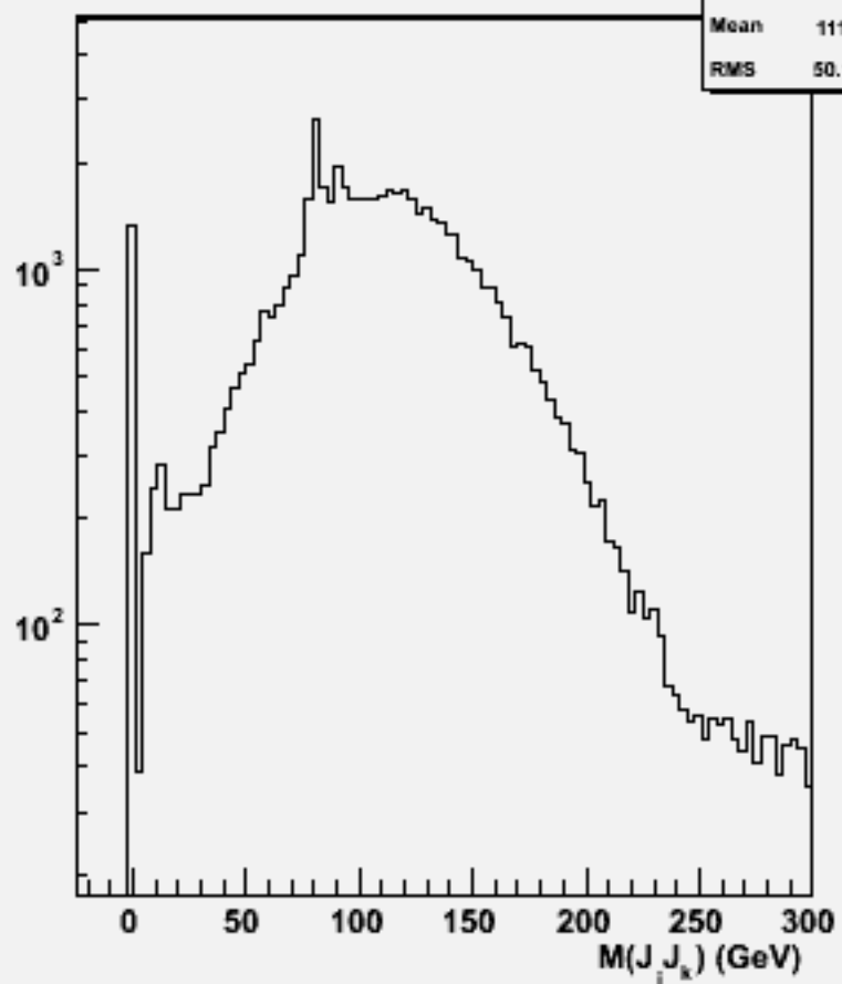
2jets mass(All comb)w101156 ssude1n1_o
