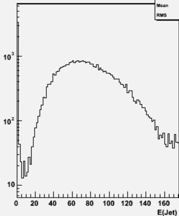
Jet energies(All jets)w101156 ssude1n1_o
