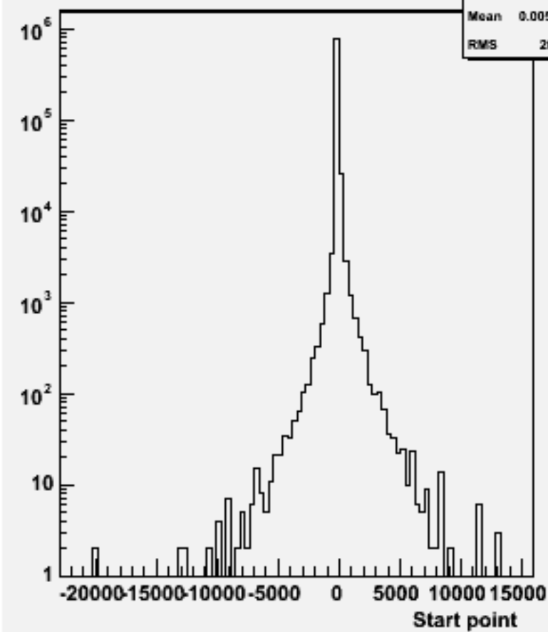
Start point Z : w101156 ssude1n1_o
