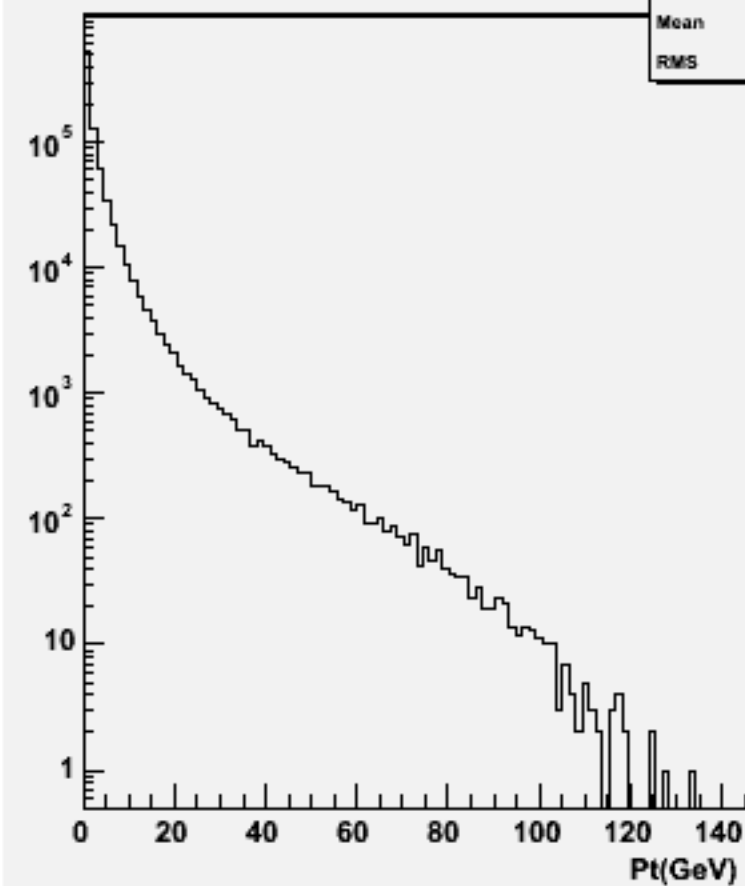
Particle Pt : w101156 ssude1n1_o
