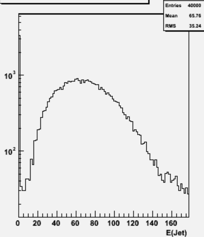
Jet energies(All jets)w101152 ssn3e3sc_o
