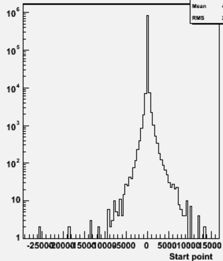
Start point Z : w101152 ssn3e3sc_o
