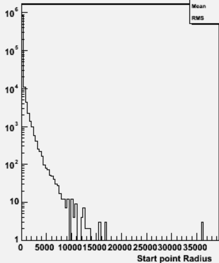
Start point R : w101152 ssn3e3sc_o
