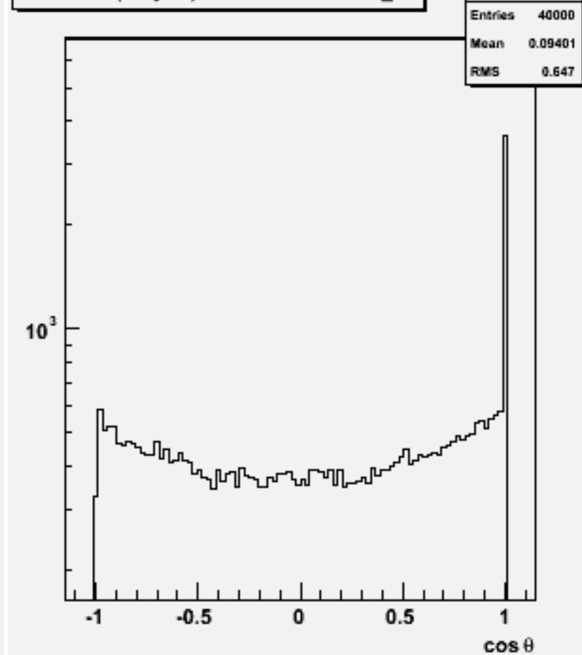
Jet cosθ (All jets)w101152 ssn3e3sc_o
