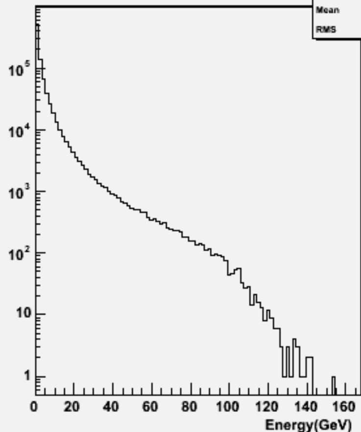
Particle Energy : w101152 ssn3e3sc_o
