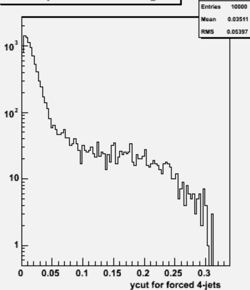
Ycut for 4-jets :w101152 ssn3e3sc_o
