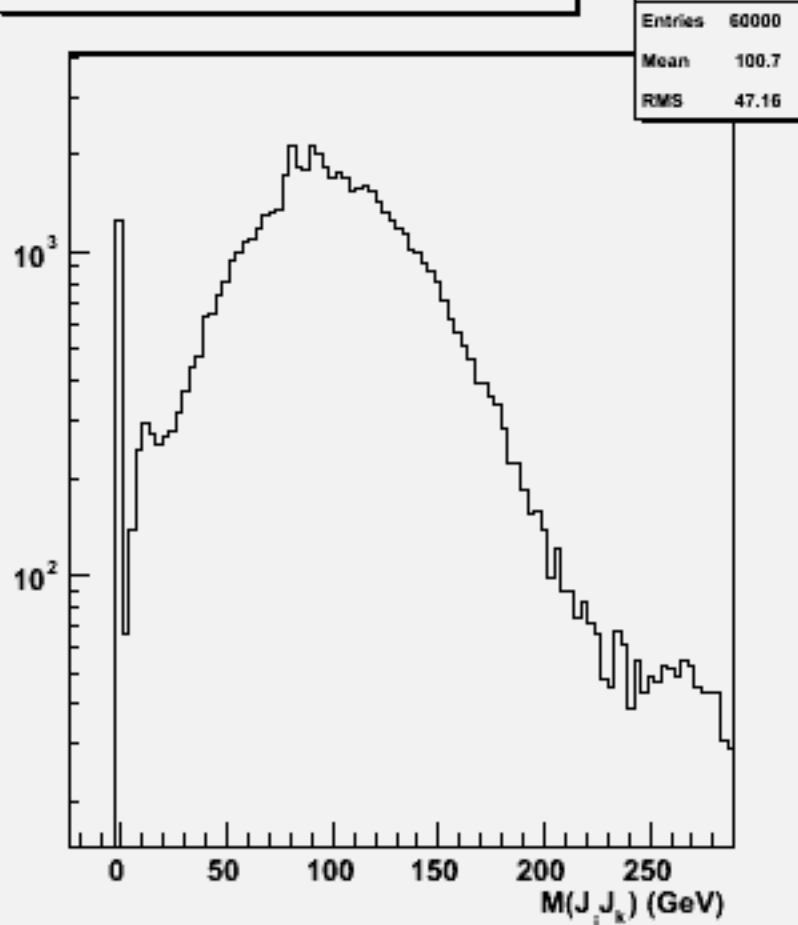
2jets mass(All comb)w101152 ssn3e3sc_o
