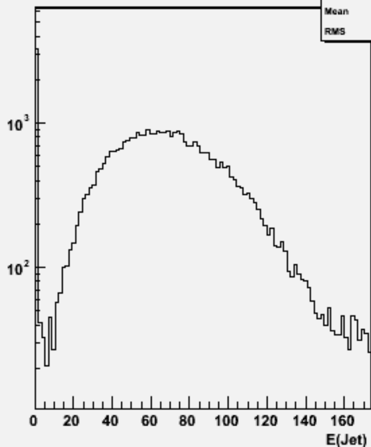
Jet energies(All jets)w101149 ssn3e3du_o
