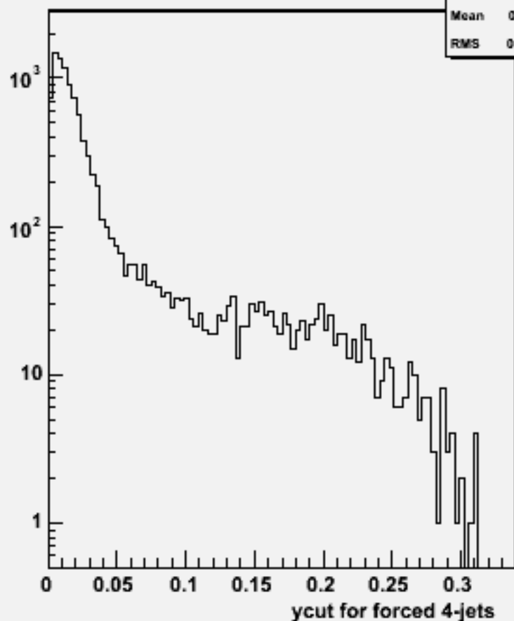
Ycut for 4-jets :w101149 ssn3e3du_o
