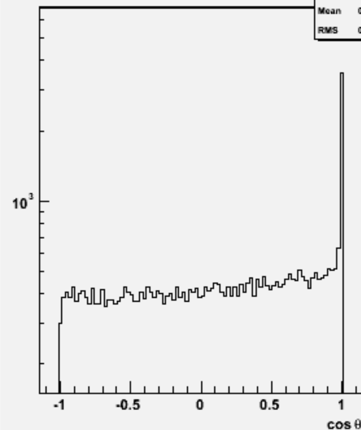
Jet cosθ (All jets)w101149 ssn3e3du_o
