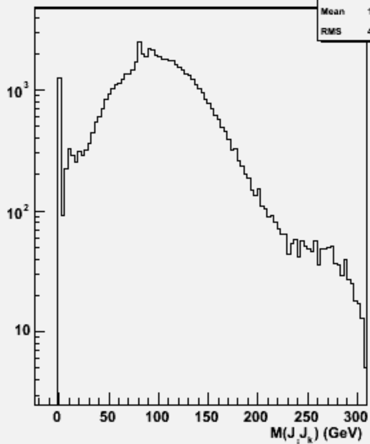
2jets mass(All comb)w101149 ssn3e3du_o
