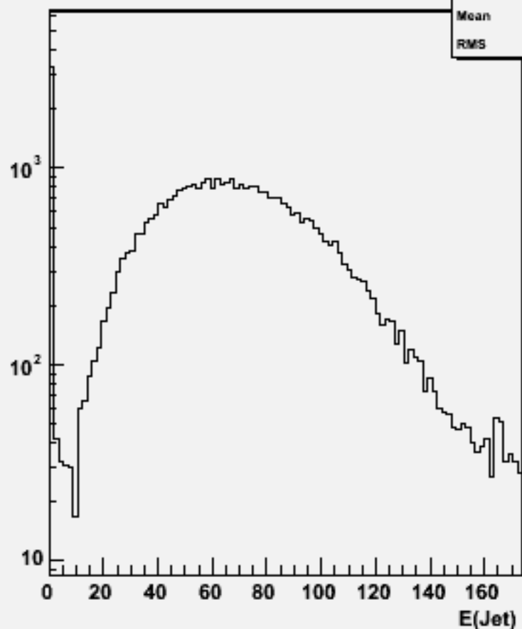
Jet energies(All jets)w101148 ssn3e3du_o
