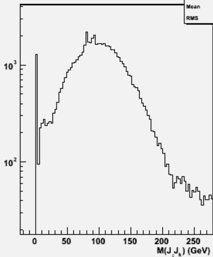
2jets mass(All comb)w101148 ssn3e3du_o
