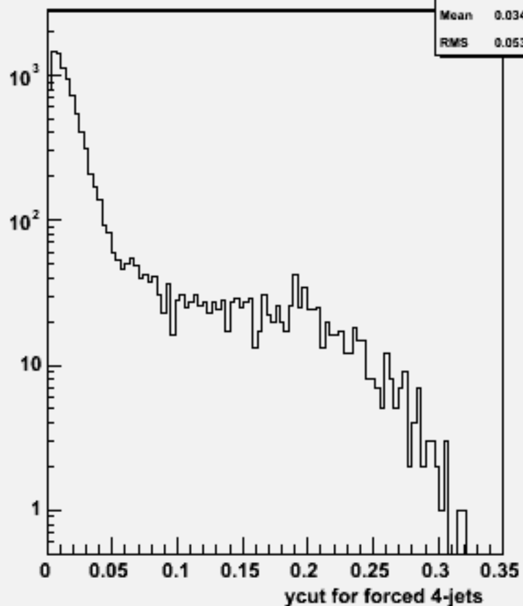
Ycut for 4-jets :w101148 ssn3e3du_o
