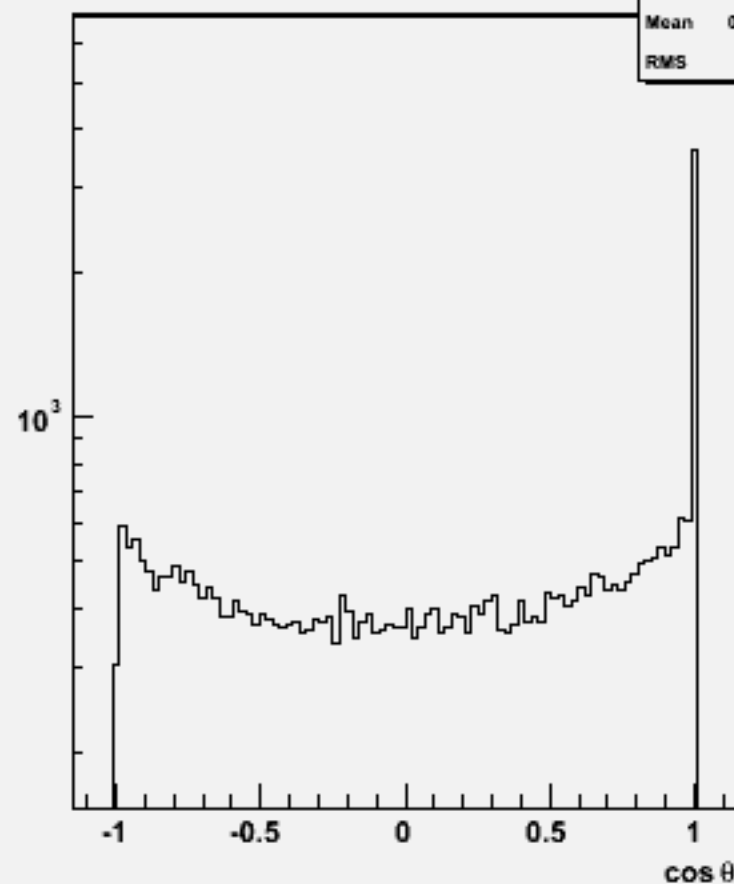
Jet cosθ (All jets)w101148 ssn3e3du_o
