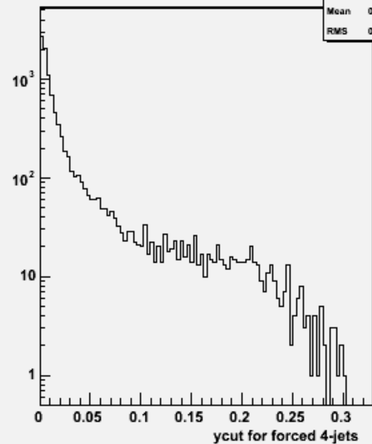
Ycut for 4-jets :w101141 ssn3e3e2n2_o
