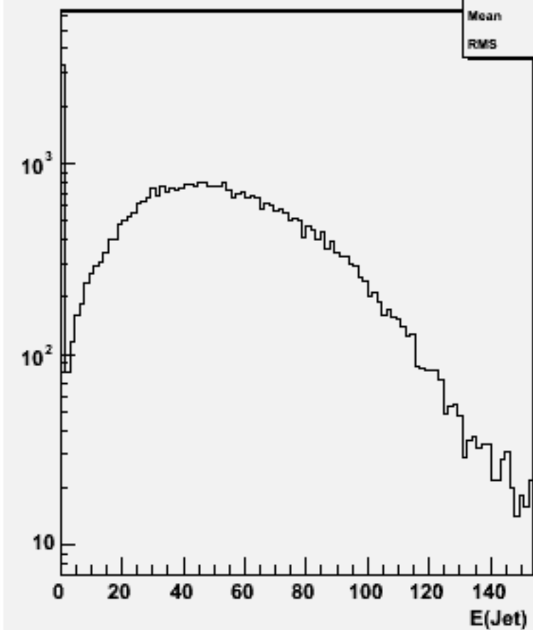
Jet energies(All jets)w101141 ssn3e3e2n2_o
