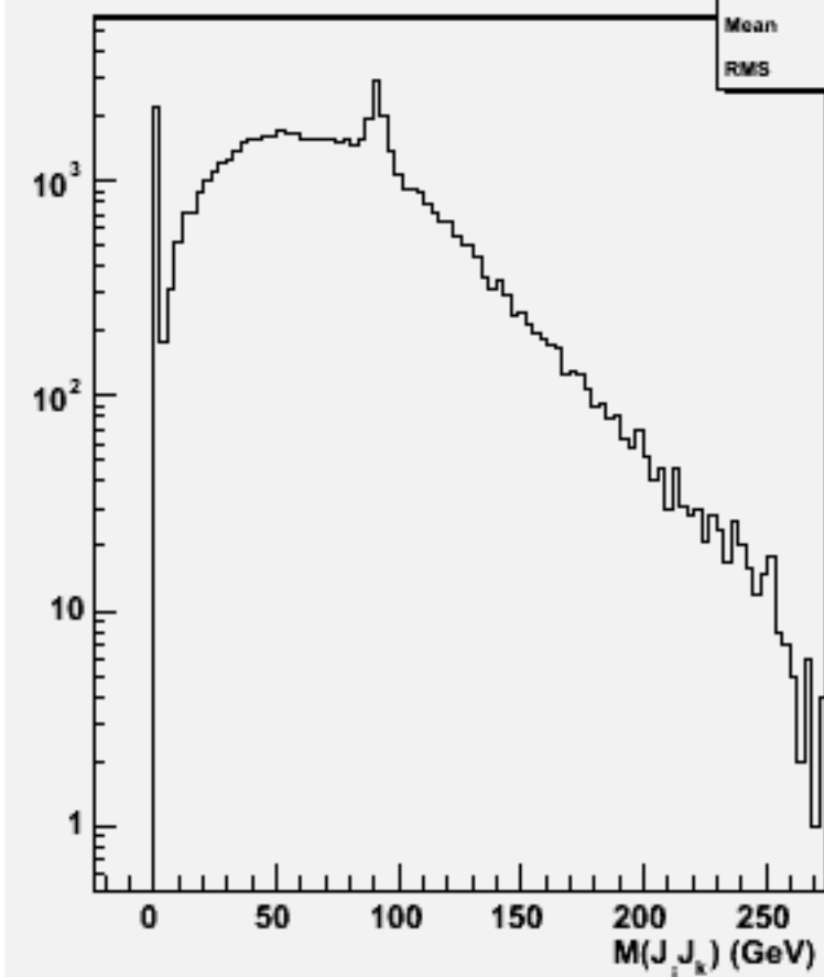
2jets mass(All comb)w101141 ssn3e3e2n2_o
