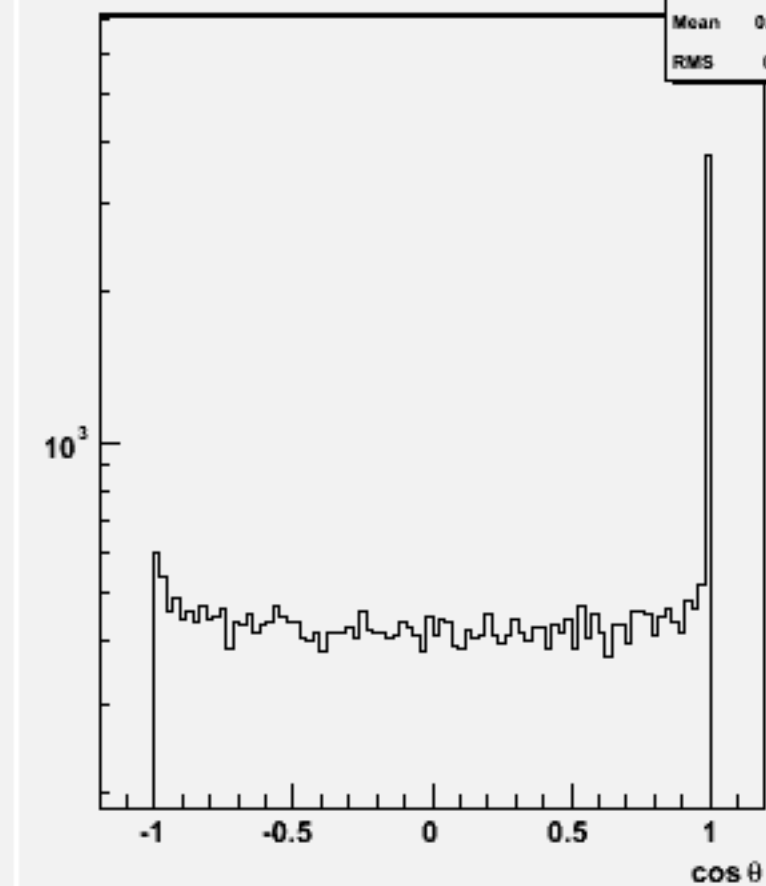
Jet cos \theta (All jets)w101141 ssn3e3e2n2_o
