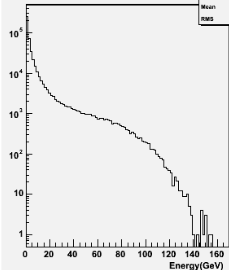
Particle Energy : w101136 ssn3e3e1n1_o
