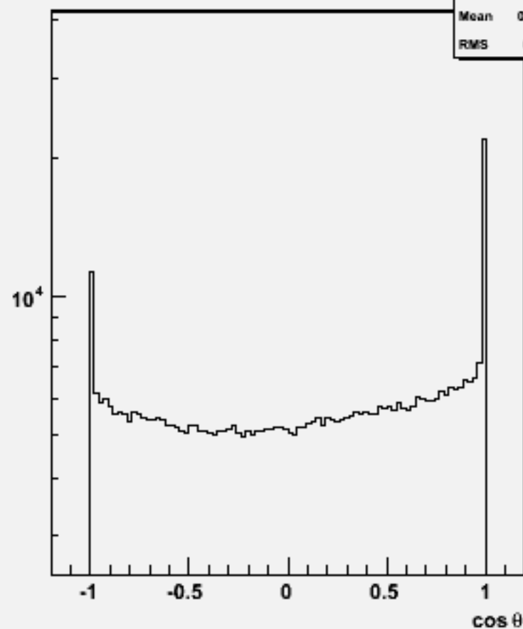
Particle cos \theta : w101136 ssn3e3e1n1_o
