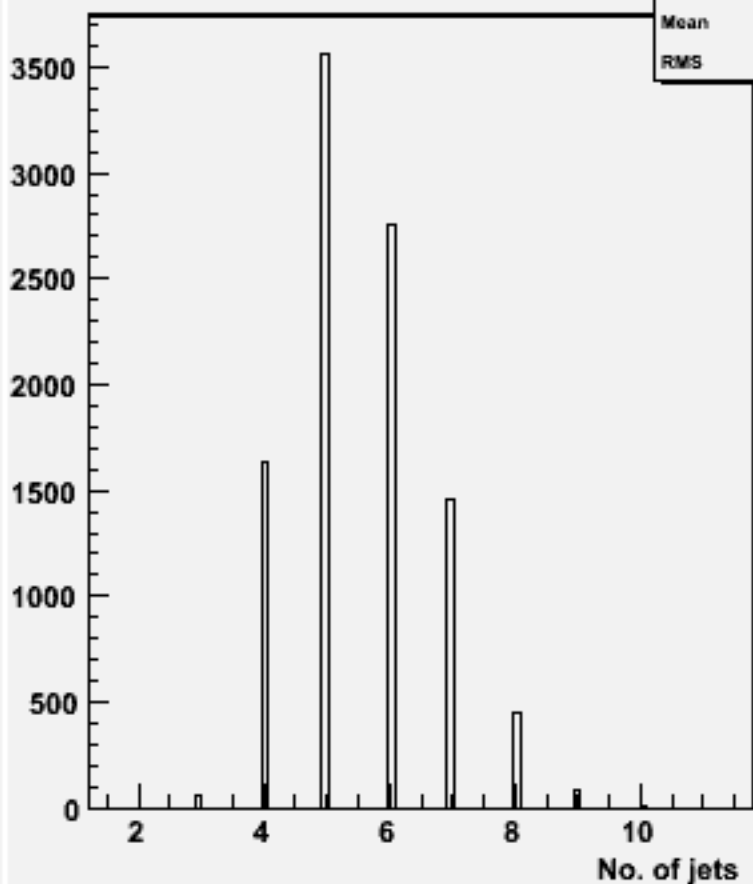
No. jets (ycut=0.001) : w101136 ssn3e3e1n1_o
