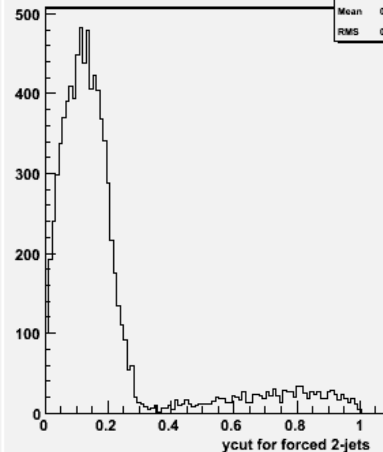
Ycut for 2-jets :w101136 ssn3e3e1n1_o
