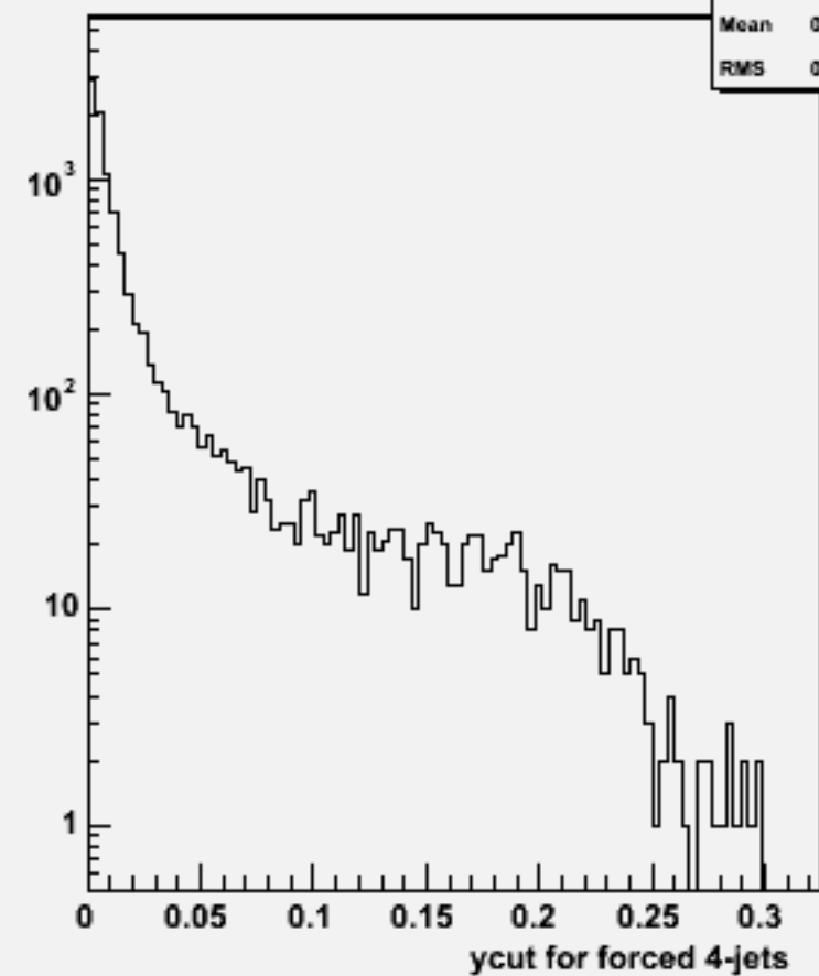
Ycut for 4-jets :w101136 ssn3e3e1n1_o
