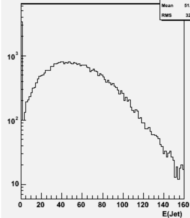
Jet energies(All jets)w101136 ssn3e3e1n1_o
