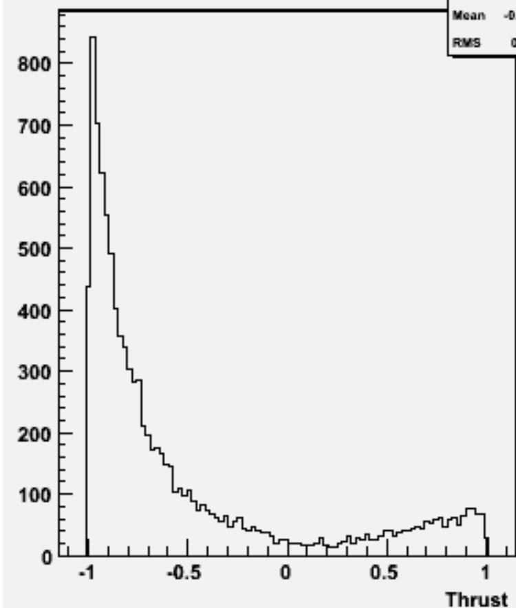
cos \Theta (thrust) w101136 ssn3e3e1n1_o
