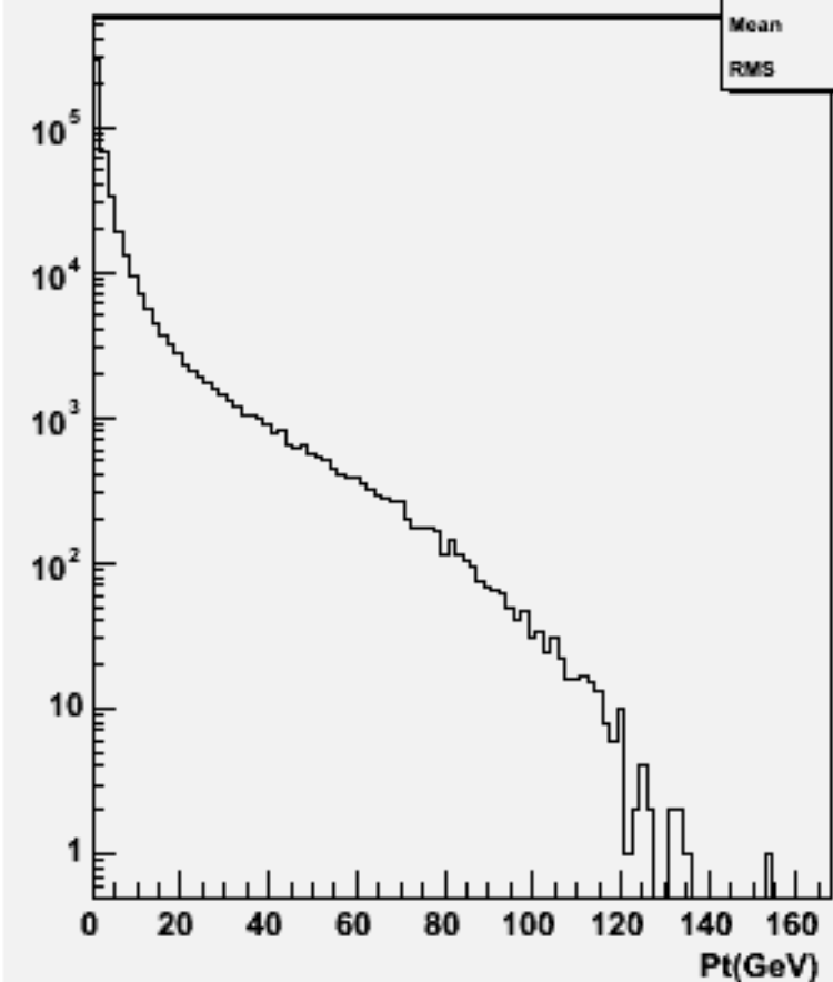
Particle Pt : w101136 ssn3e3e1n1_o
