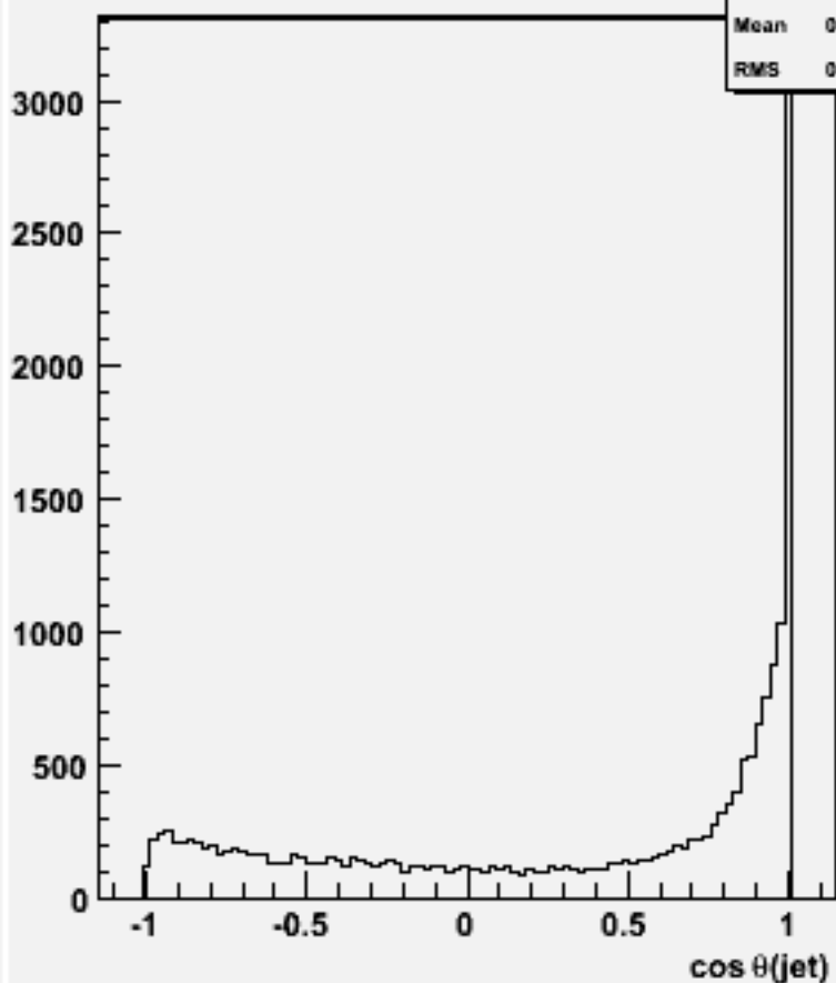
cos \theta for 2-jets :w101136 ssn3e3e1n1_o
