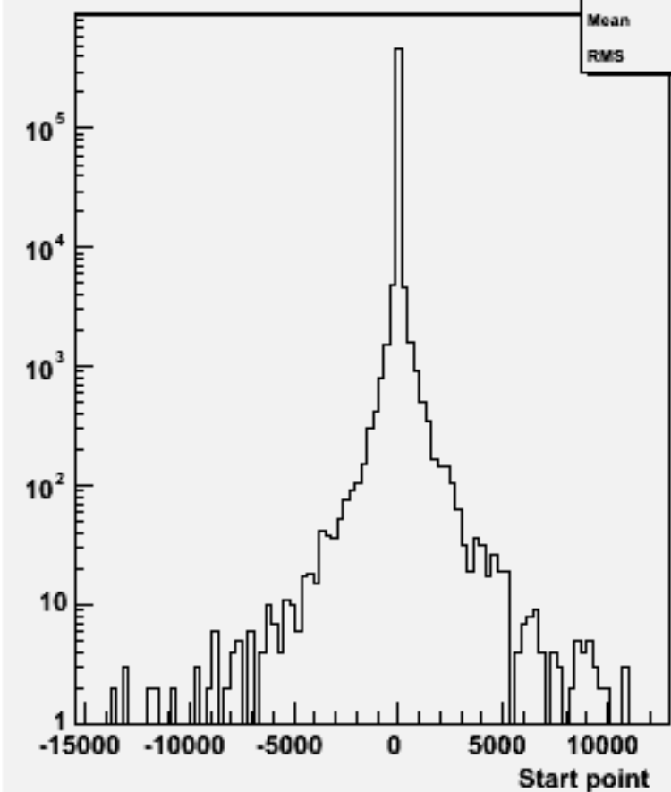
Start point Z : w101136 ssn3e3e1n1_o
