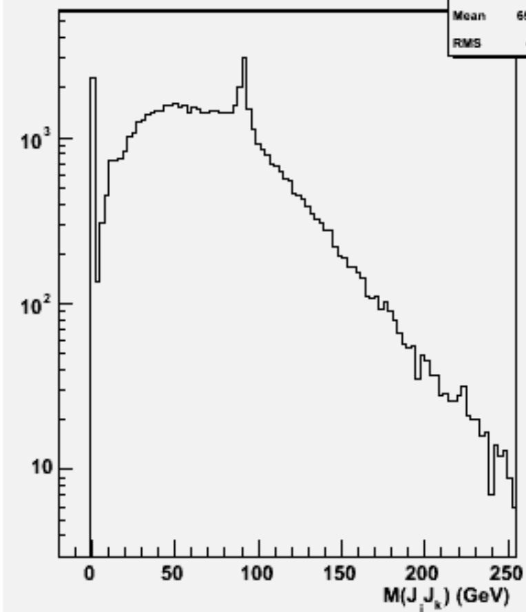
2jets mass(All comb)w101136 ssn3e3e1n1_o
