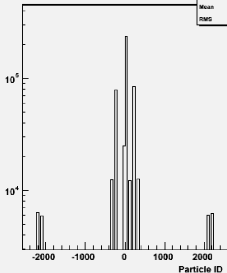
Particle ID : w101136 ssn3e3e1n1_o
