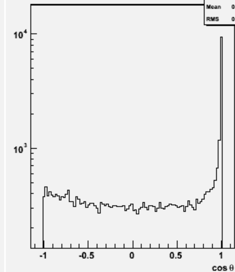
Jet cos \theta (All jets)w101136 ssn3e3e1n1_o
