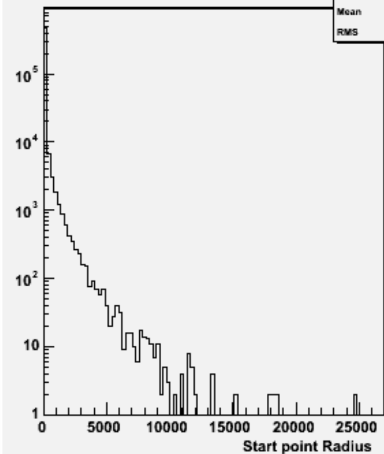
Start point R : w101136 ssn3e3e1n1_o
