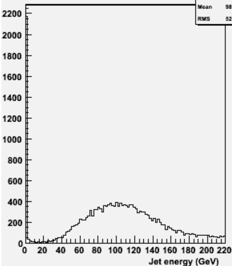
energy for 2-jets :w101136 ssn3e3e1n1_o
