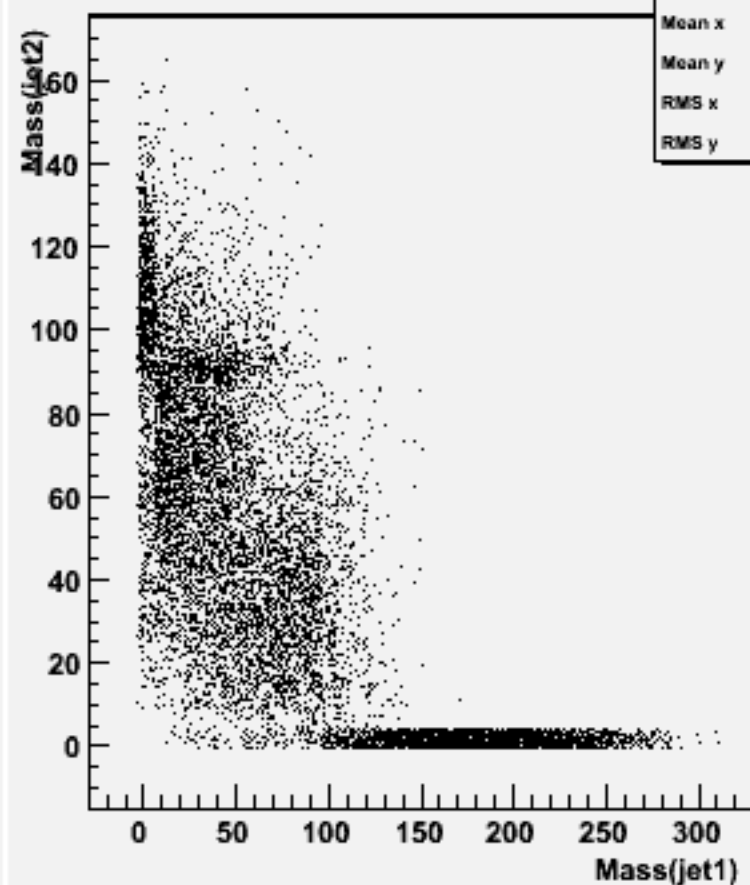
Jet mass for forced 2-jets : w101136 ssn3e3e1n1_o
