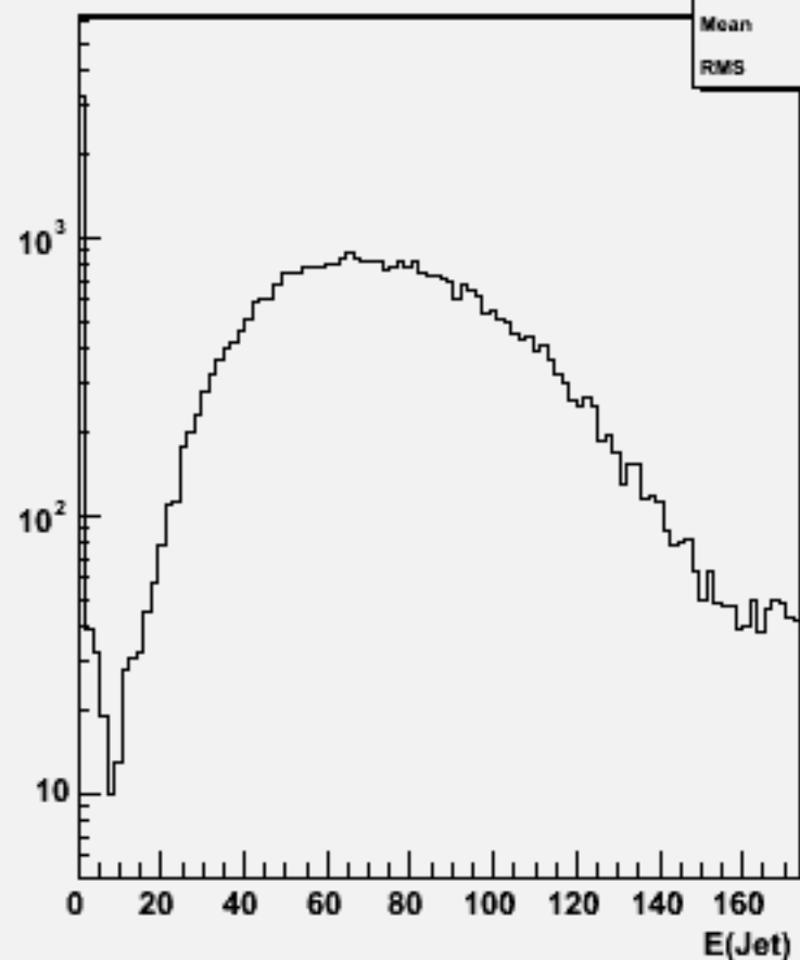
Jet energies(All jets)w101133 ssn2e2sc_o
