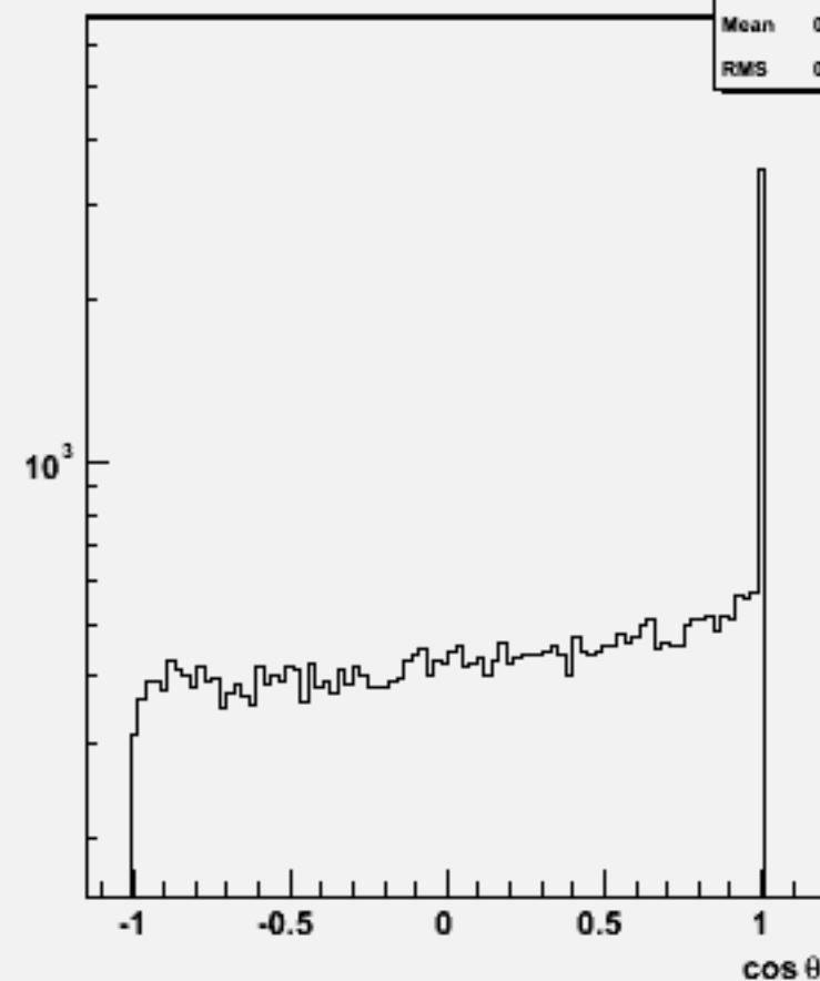
Jet cosθ (All jets)w101133 ssn2e2sc_o
