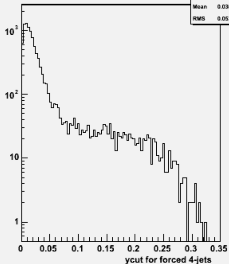
Ycut for 4-jets :w101133 ssn2e2sc_o
