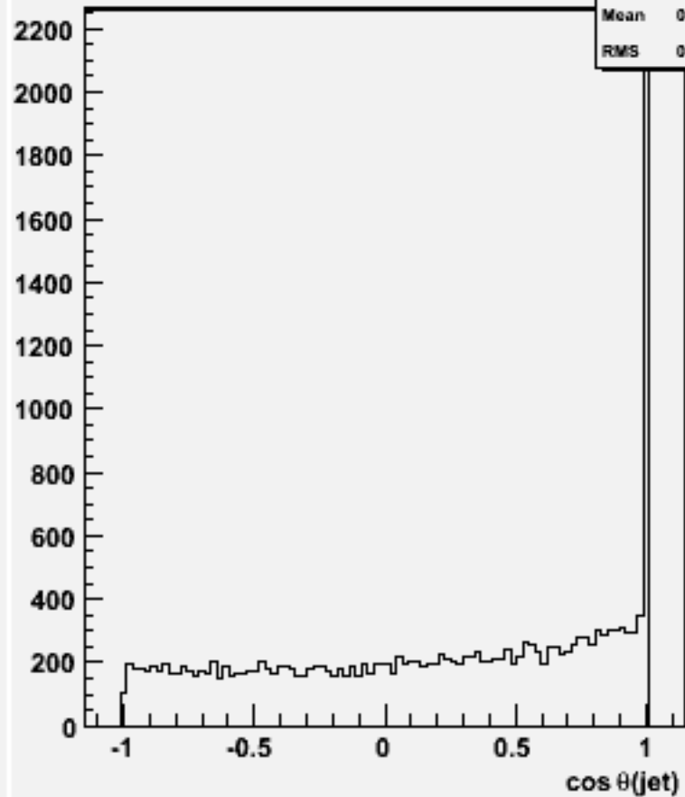
cos \theta for 2-jets :w101133 ssn2e2sc_o
