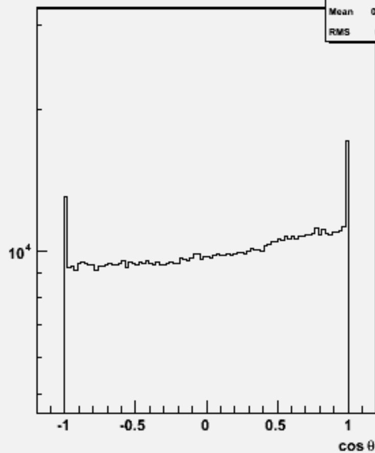
Particle cosθ : w101133 ssn2e2sc_o
