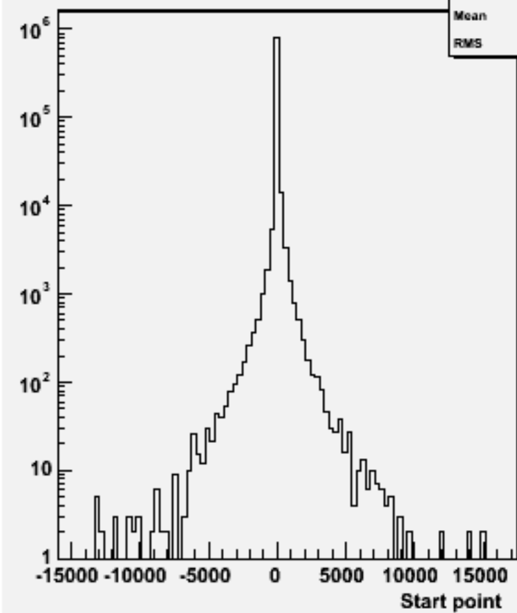
Start point Z : w101133 ssn2e2sc_o
