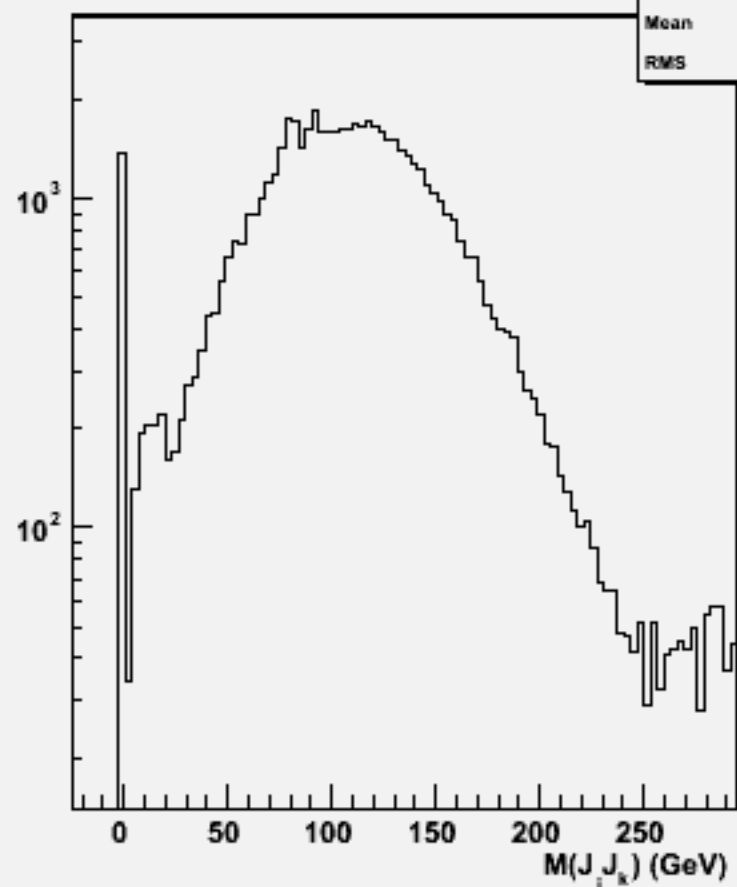
2jets mass(All comb)w101133 ssn2e2sc_o
