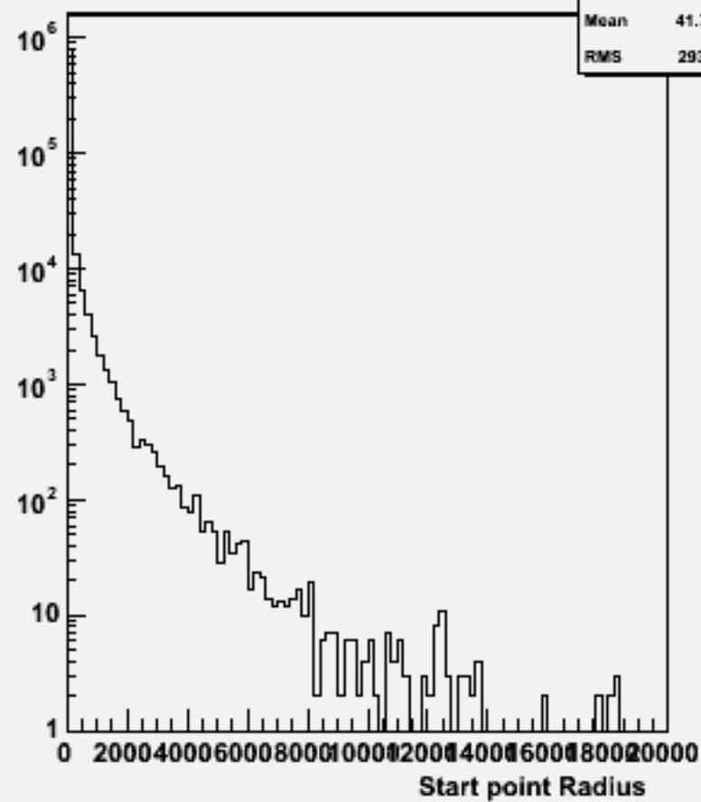
Start point R : w101133 ssn2e2sc_o
