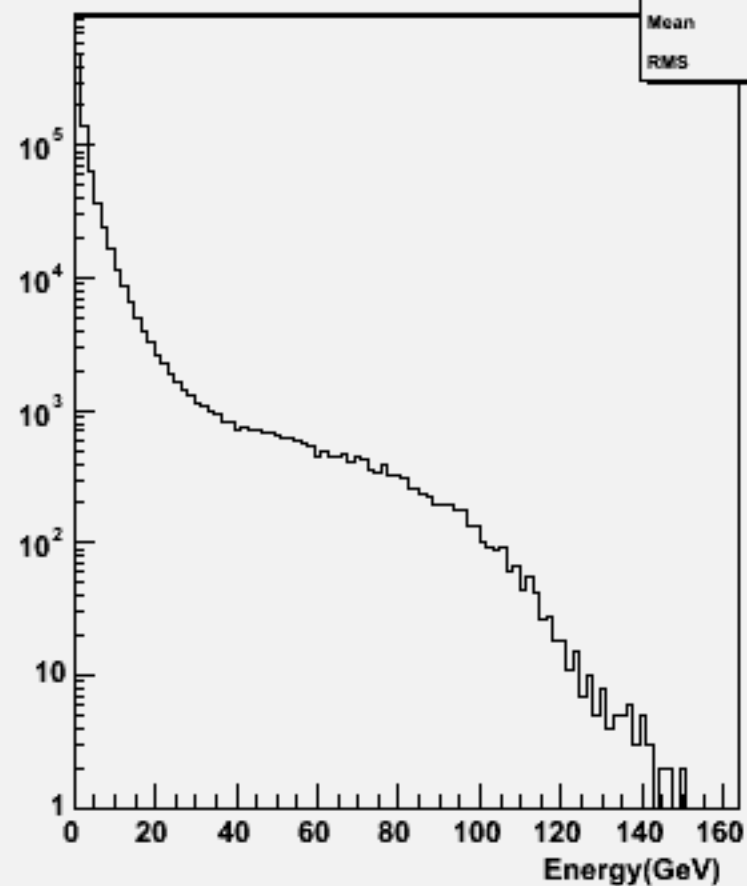
Particle Energy : w101133 ssn2e2sc_o
