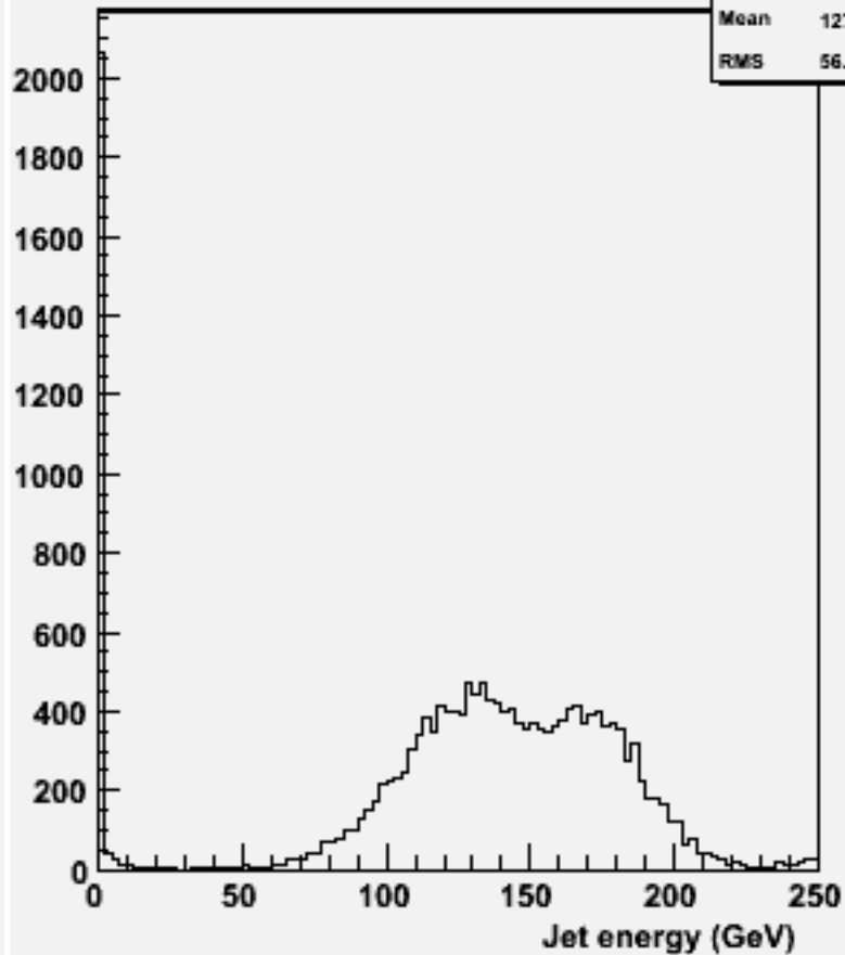
energy for 2-jets :w101133 ssn2e2sc_o
