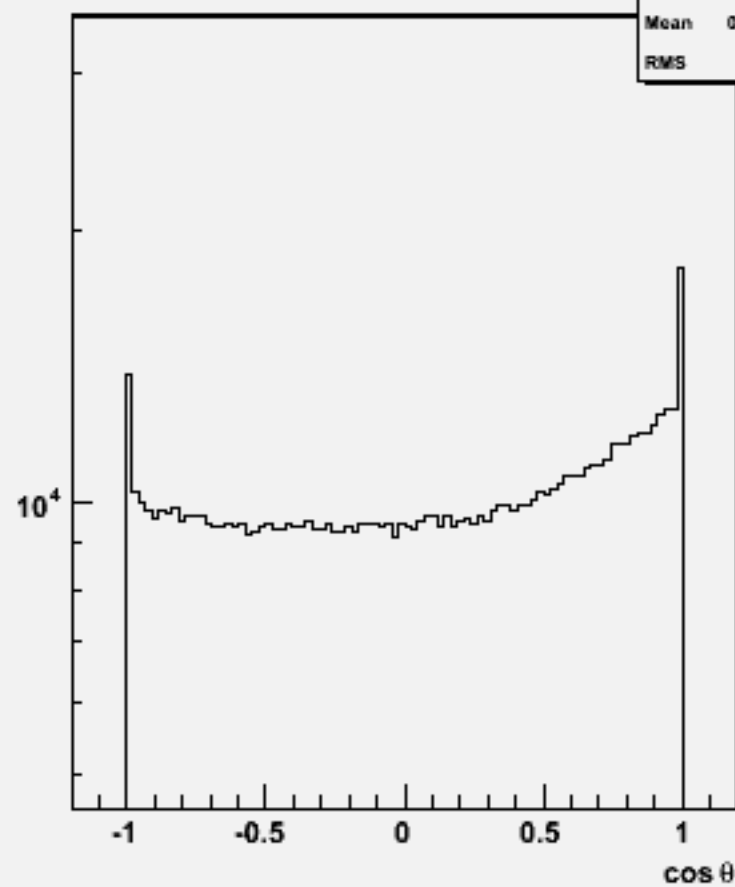
Particle cos \theta : w101132 ssn2e2sc_o
