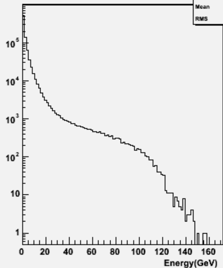
Particle Energy : w101132 ssn2e2sc_o
