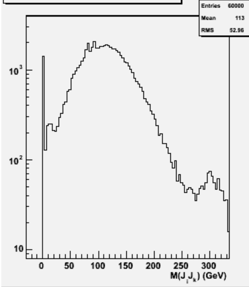
2jets mass(All comb)w101132 ssn2e2sc_o
