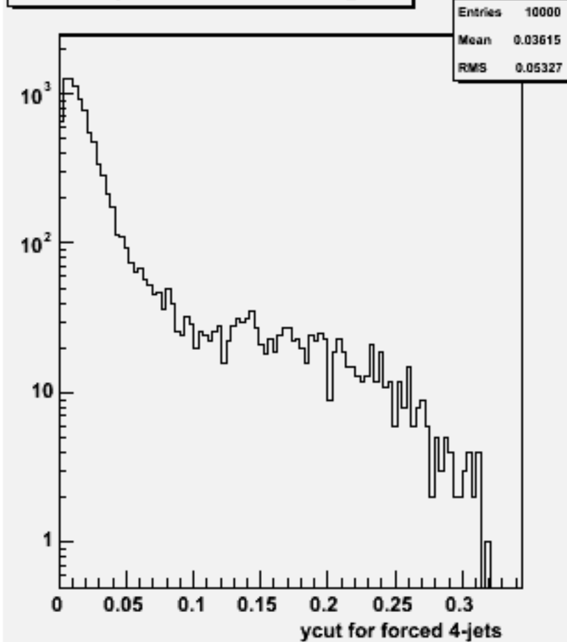
Ycut for 4-jets :w101132 ssn2e2sc_o
