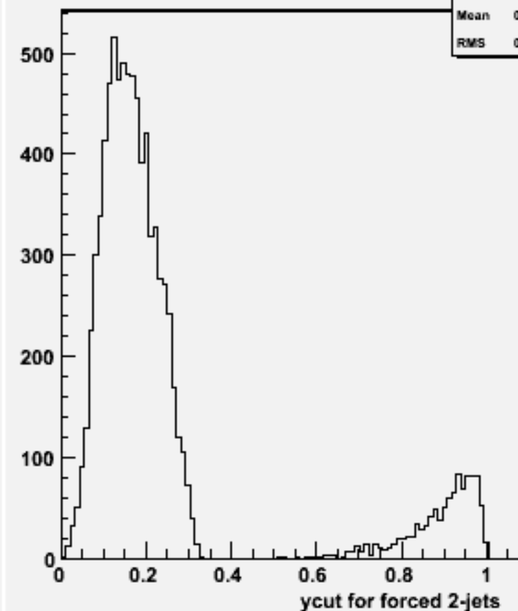
Ycut for 2-jets :w101132 ssn2e2sc_o
