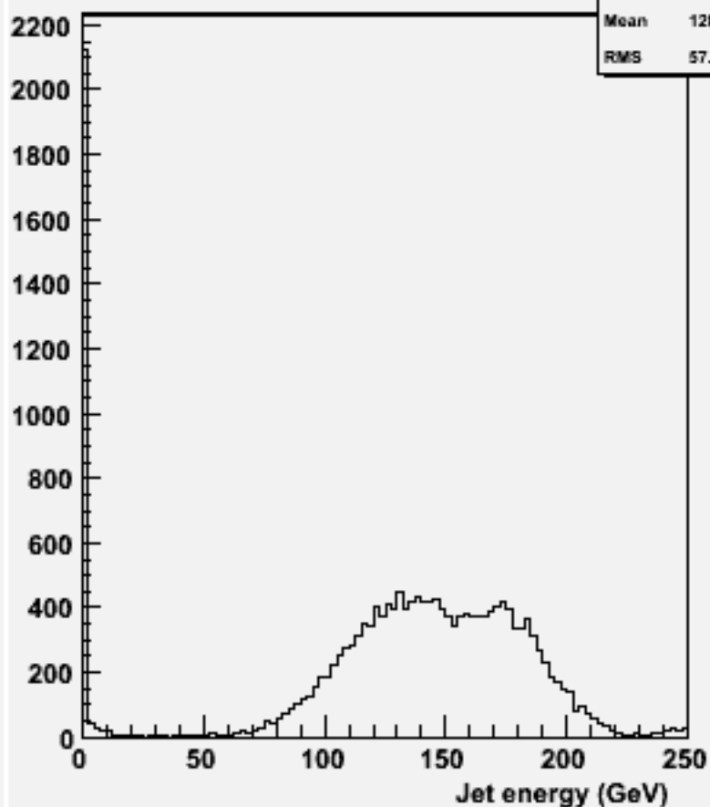
energy for 2-jets :w101132 ssn2e2sc_o
