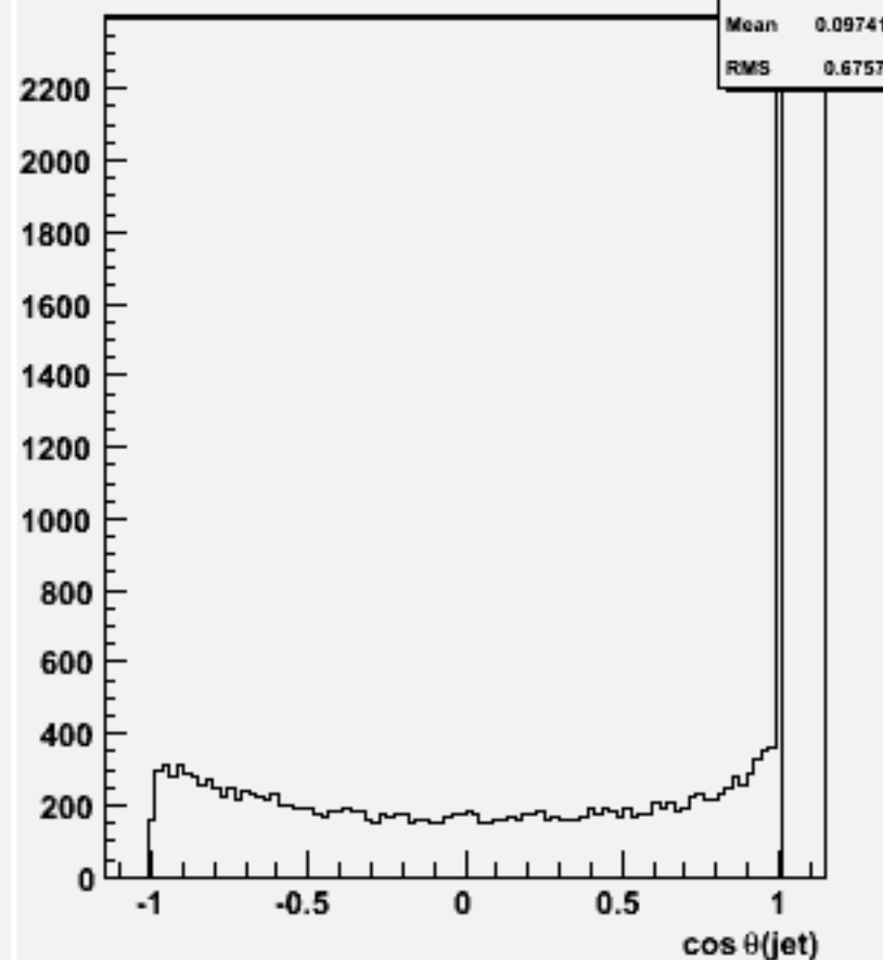
cos \theta for 2-jets :w101132 ssn2e2sc_o
