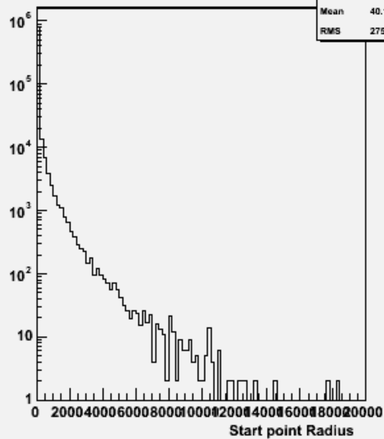
Start point R : w101132 ssn2e2sc_o
