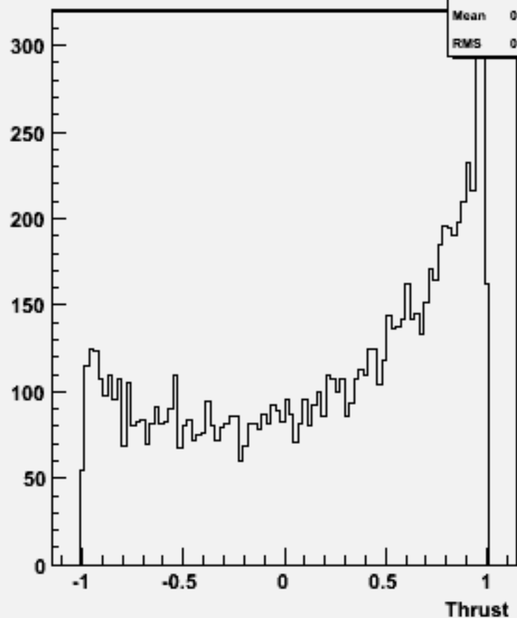
cos \Theta (thrust) w101132 ssn2e2sc_o
