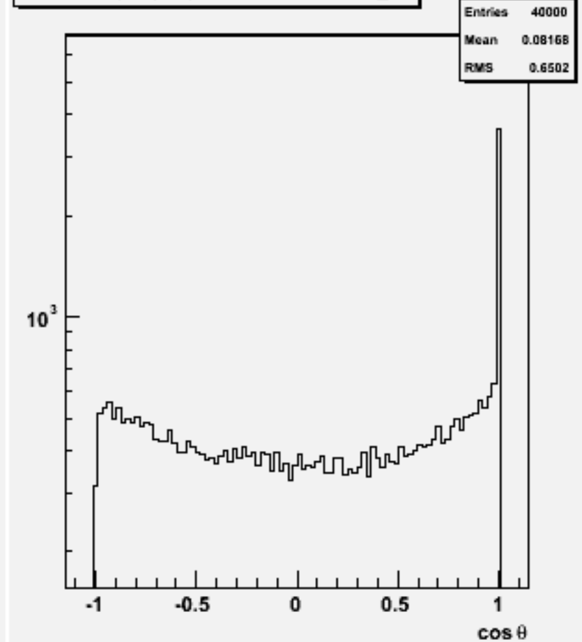
Jet cos \theta (All jets)w101132 ssn2e2sc_o
