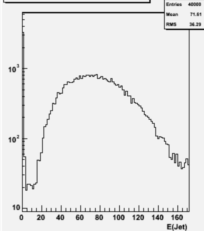
Jet energies(All jets)w101132 ssn2e2sc_o
