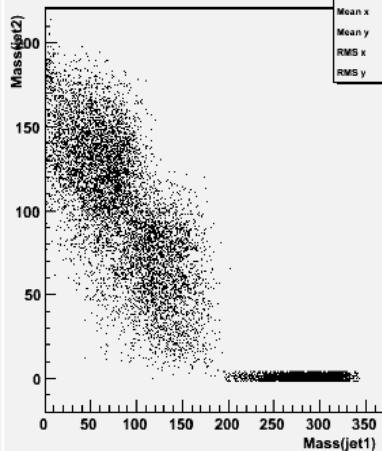
Jet mass for forced 2-jets : w101132 ssn2e2sc_o
