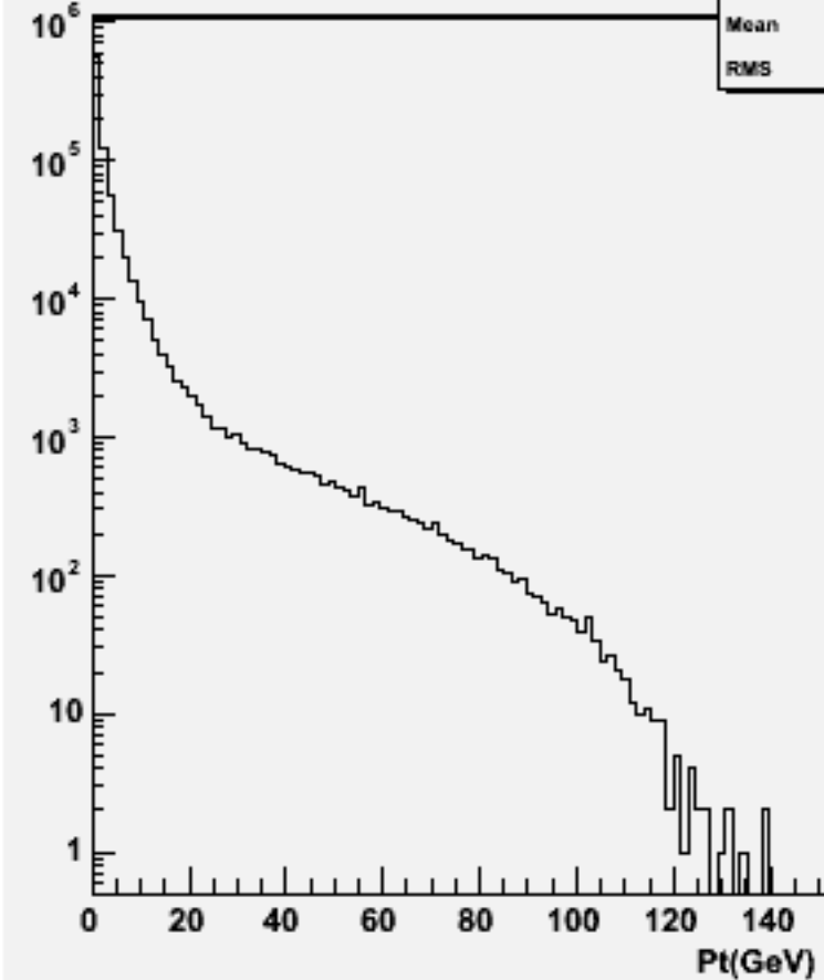
Particle Pt : w101132 ssn2e2sc_o
