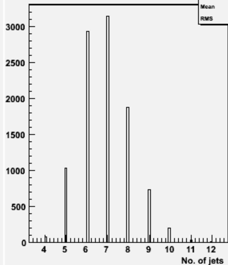
No. jets (ycut=0.001) : w101132 ssn2e2sc_o
