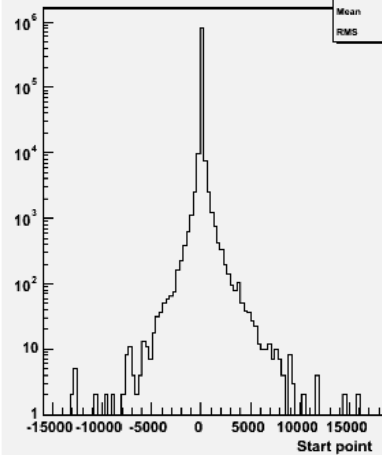
Start point Z : w101132 ssn2e2sc_o
