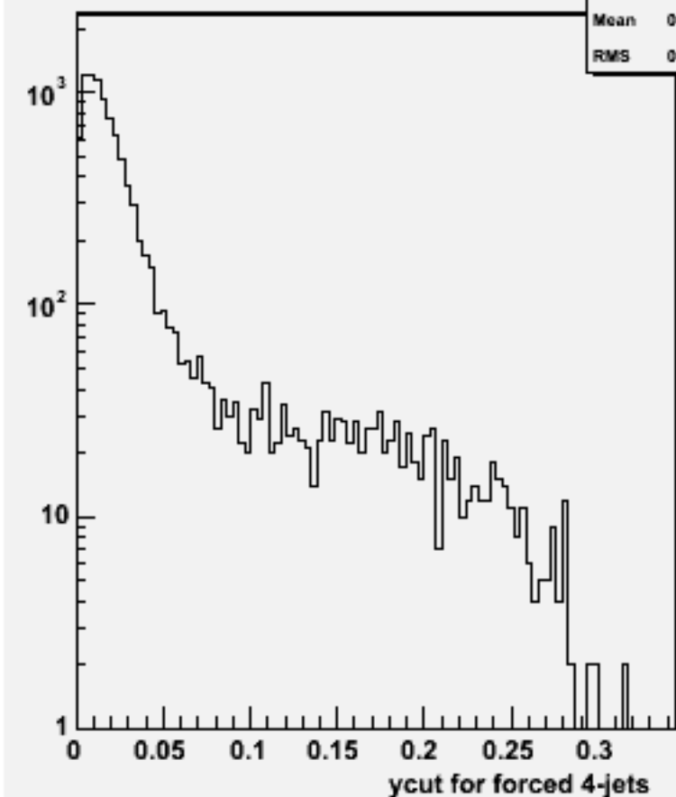
Ycut for 4-jets :w101129 ssn2e2du_o
