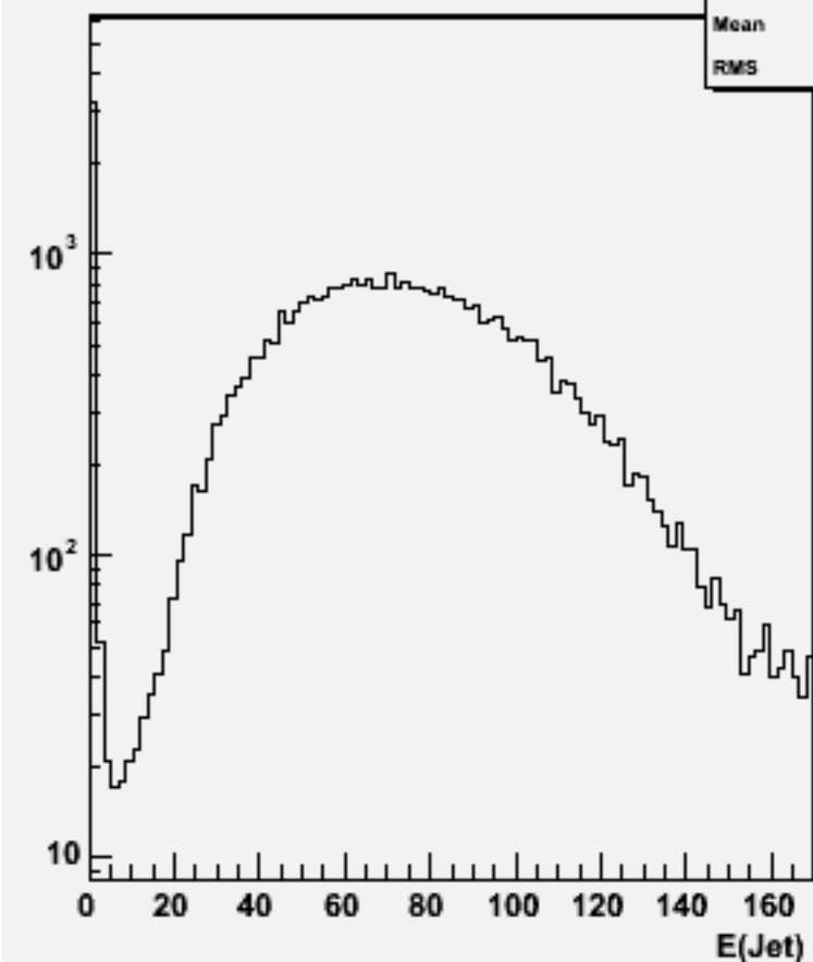
Jet energies(All jets)w101129 ssn2e2du_o
