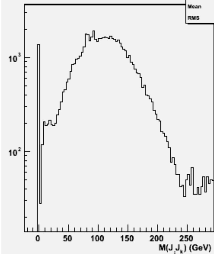
2jets mass(All comb)w101129 ssn2e2du_o
