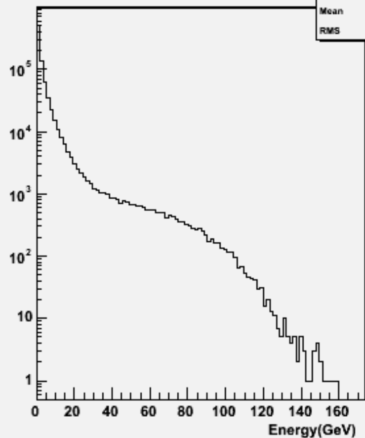
Particle Energy : w101129 ssn2e2du_o
