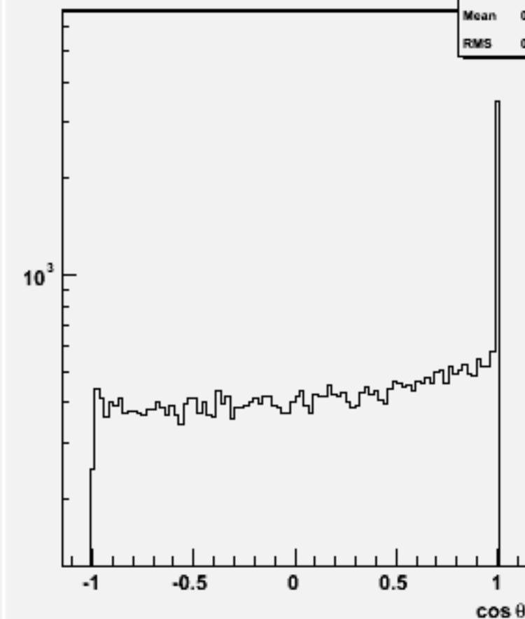
Jet cos \theta (All jets)w101129 ssn2e2du_o
