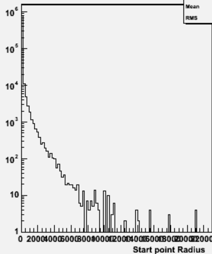
Start point R : w101128 ssn2e2du_o
