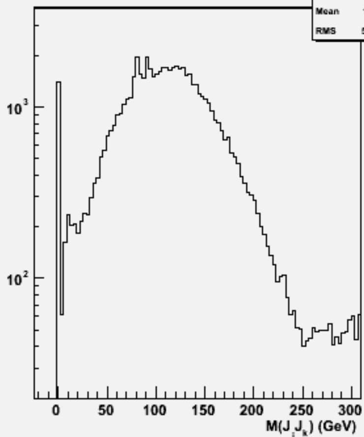
2jets mass(All comb)w101128 ssn2e2du_o
