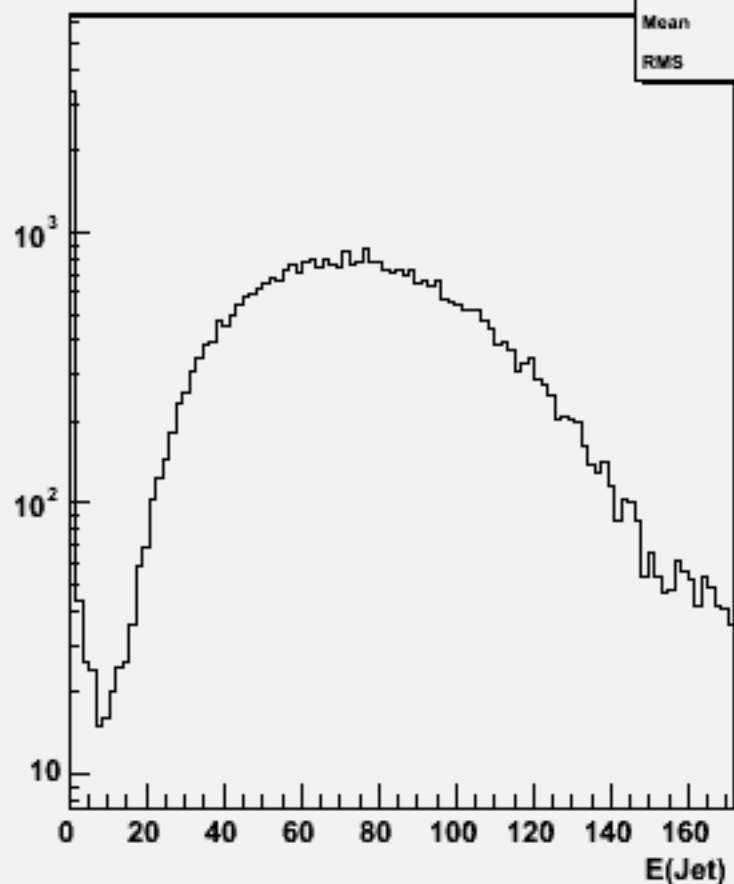
Jet energies(All jets)w101128 ssn2e2du_o
