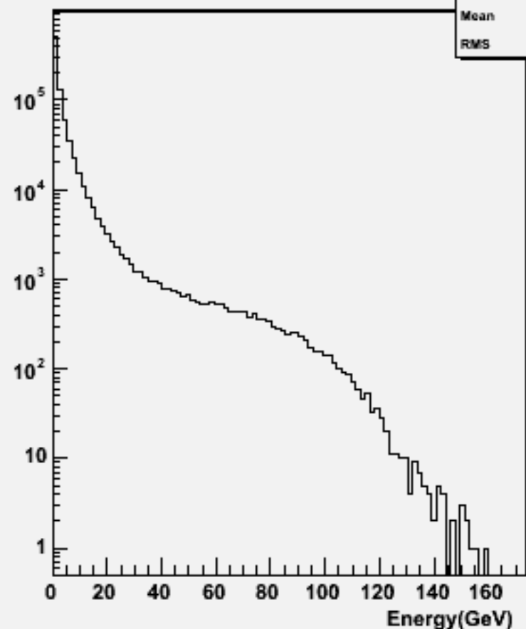
Particle Energy : w101128 ssn2e2du_o
