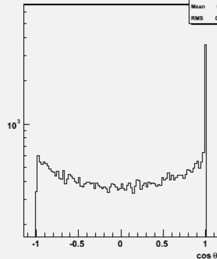
Jet cos \theta (All jets)w101128 ssn2e2du_o
