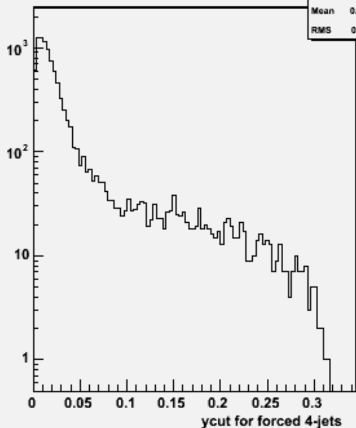
Ycut for 4-jets :w101128 ssn2e2du_o
