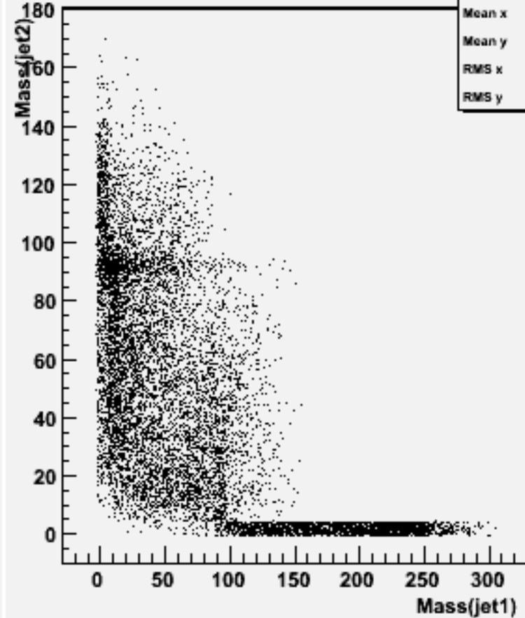
Jet mass for forced 2-jets : w101121 ssn2e2e2n2_o
