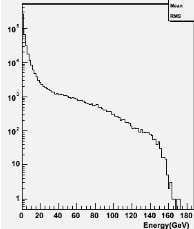
Particle Energy : w101121 ssn2e2e2n2_o
