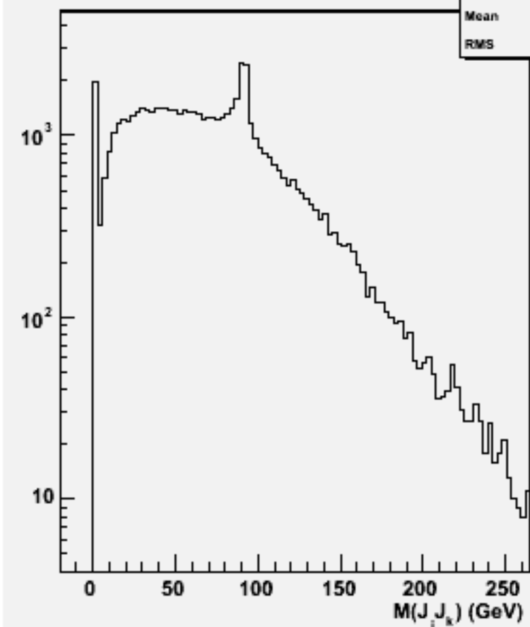
2jets mass(All comb)w101121 ssn2e2e2n2_o
