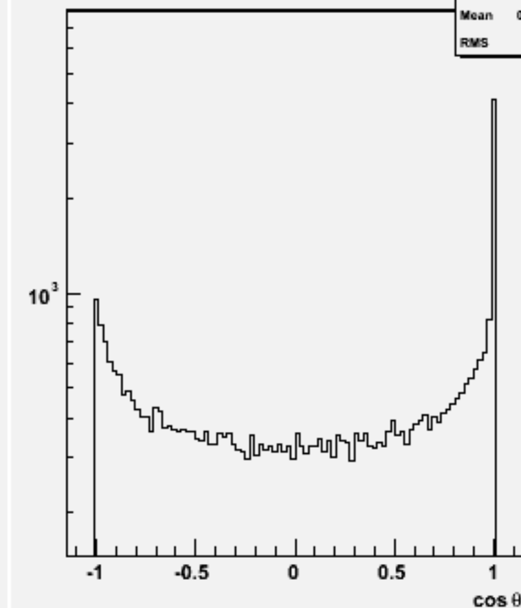
Jet cos \theta (All jets)w101121 ssn2e2e2n2_o
