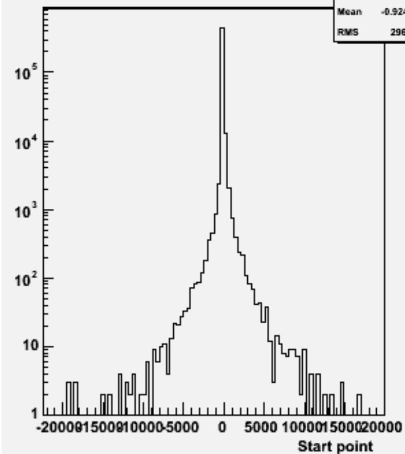
Start point Z : w101121 ssn2e2e2n2_o
