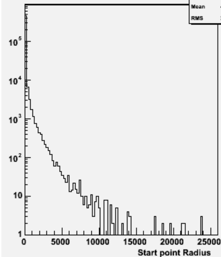
Start point R : w101121 ssn2e2e2n2_o
