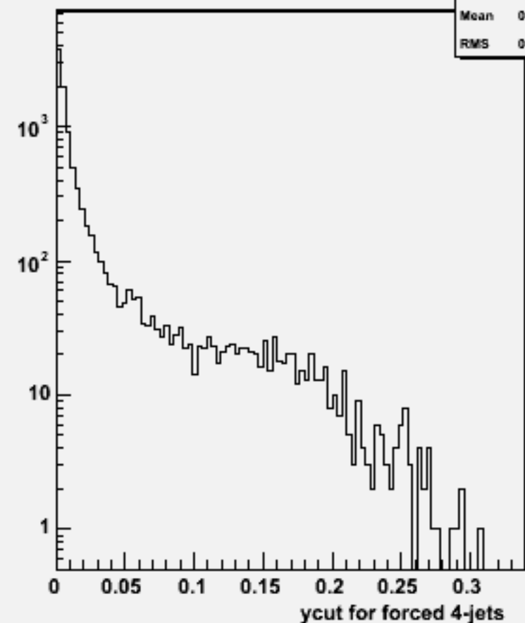
Ycut for 4-jets :w101121 ssn2e2e2n2_o
