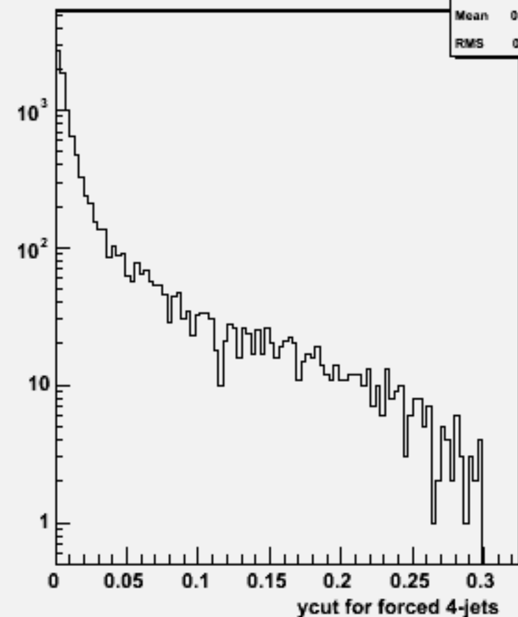
Ycut for 4-jets :w101120 ssn2e2e2n2_o
