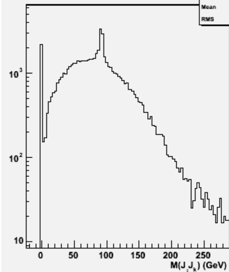
2jets mass(All comb)w101120 ssn2e2e2n2_o
