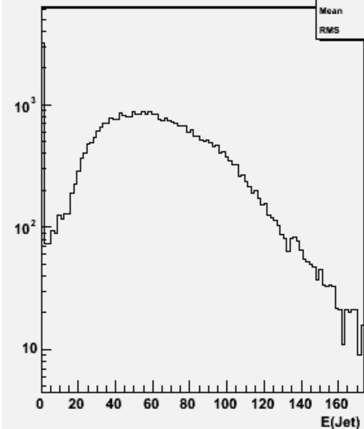
Jet energies(All jets)w101120 ssn2e2e2n2_o
