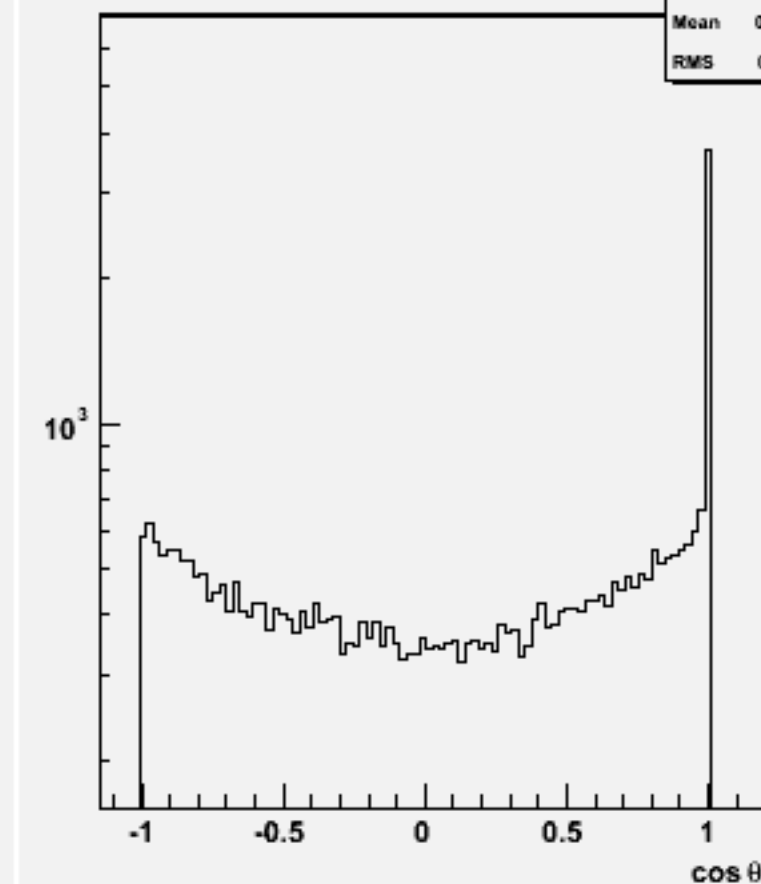
Jet cos \theta (All jets)w101120 ssn2e2e2n2_o
