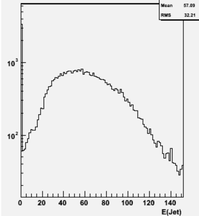
Jet energies(All jets)w101117 ssn2e2e1n1_o
