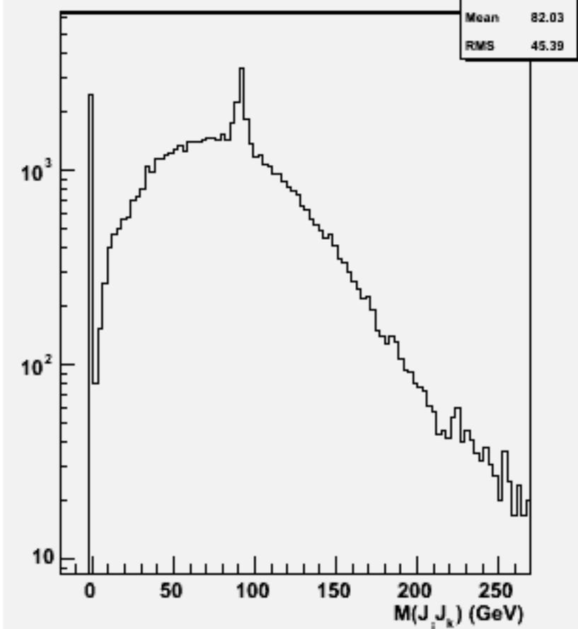
2jets mass(All comb)w101117 ssn2e2e1n1_o
