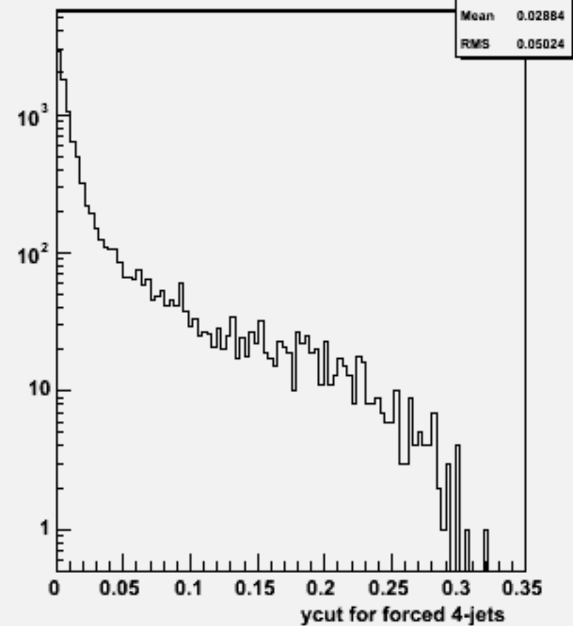
Ycut for 4-jets :w101117 ssn2e2e1n1_o
