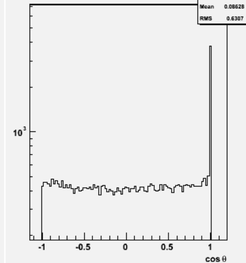
Jet cos \theta (All jets)w101117 ssn2e2e1n1_o
