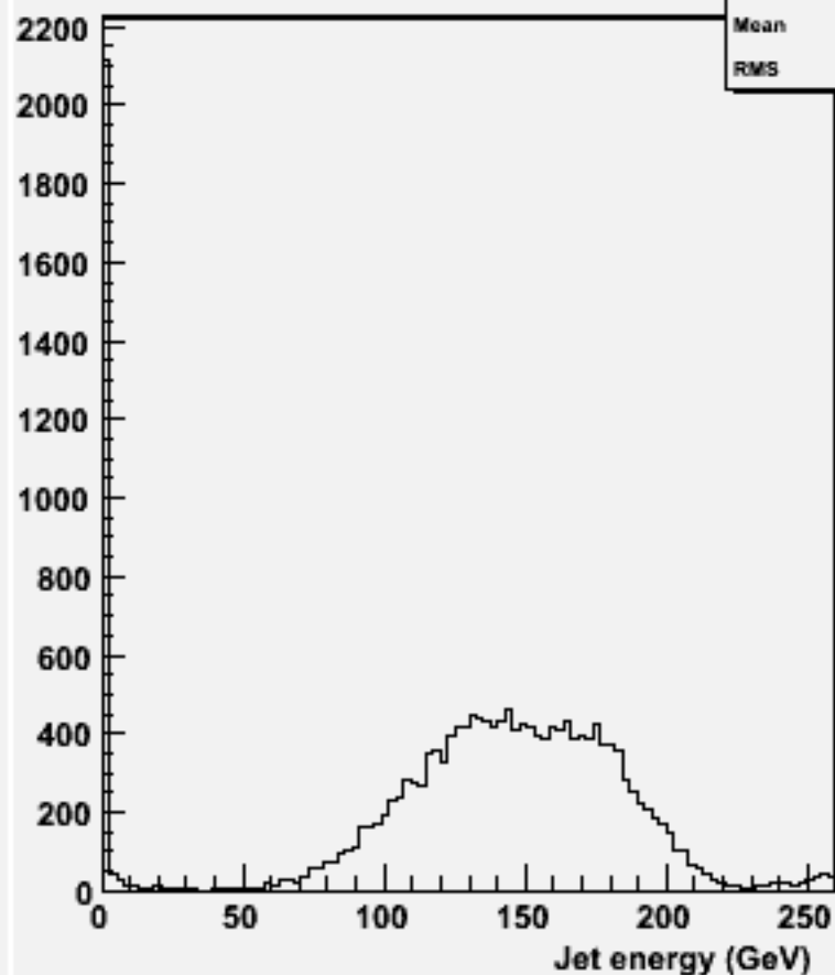
energy for 2-jets :w101112 ssn1e1sc_o
