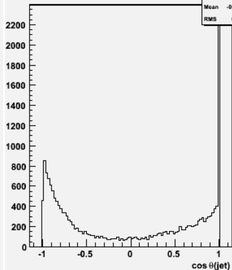
cos \theta for 2-jets :w101112 ssn1e1sc_o
