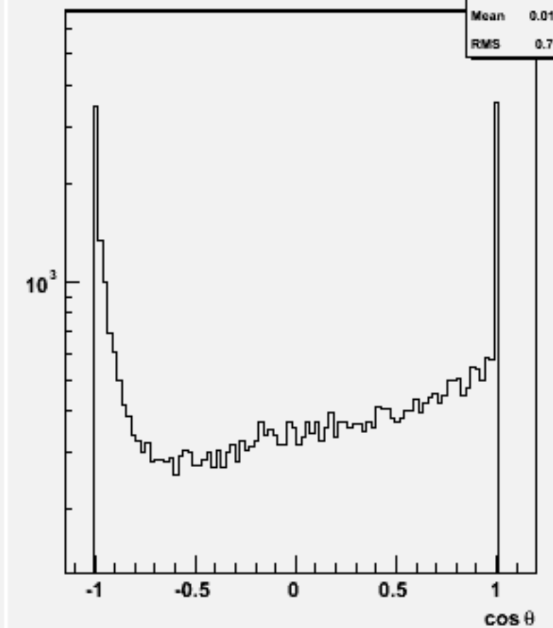
Jet cosθ (All jets)w101112 ssn1e1sc_o
