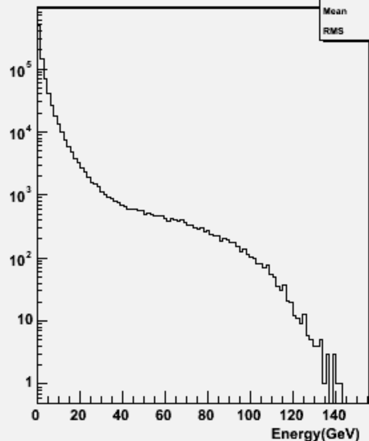
Particle Energy : w101112 ssn1e1sc_o
