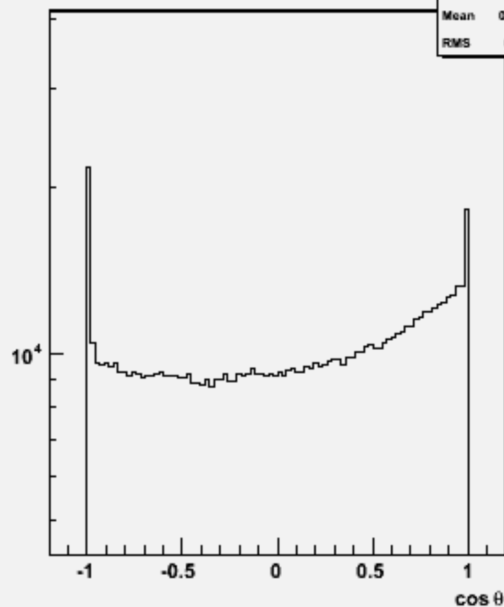
Particle cosθ : w101112 ssn1e1sc_o
