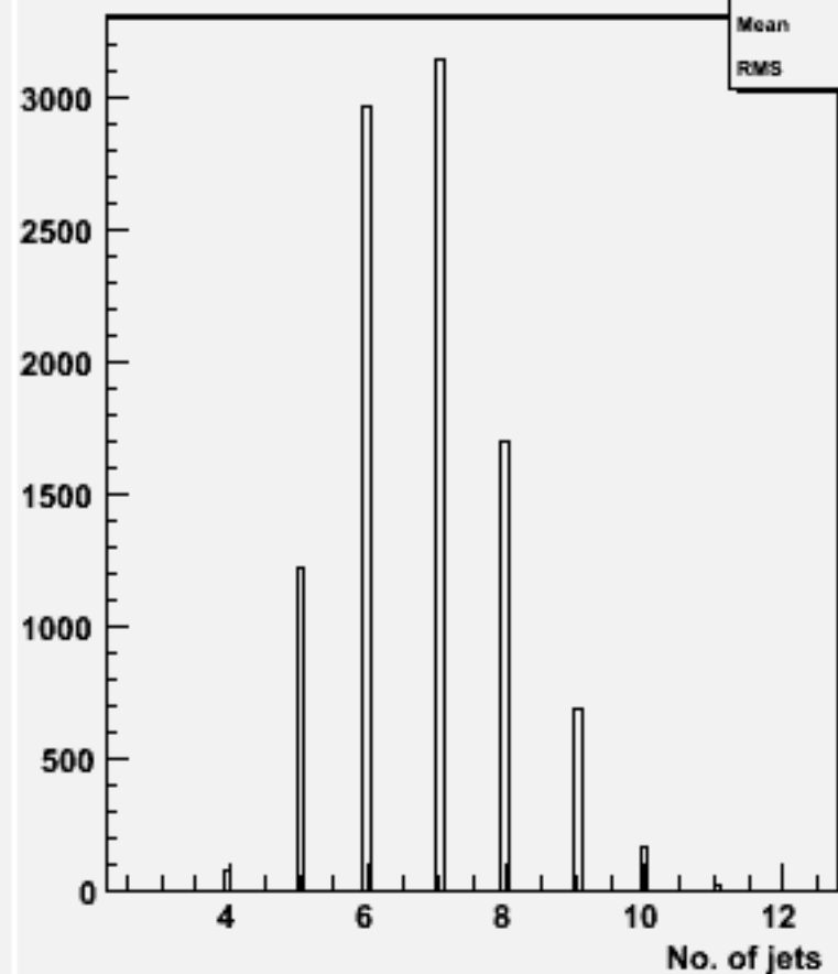
No. jets (ycut=0.001) : w101112 ssn1e1sc_o
