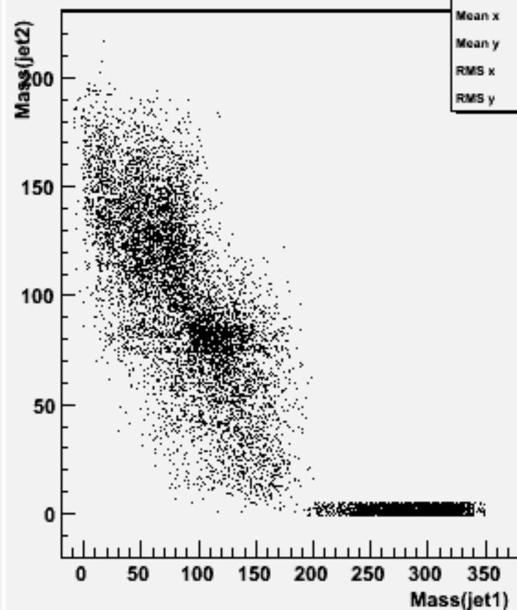
Jet mass for forced 2-jets : w101112 ssn1e1sc_o
