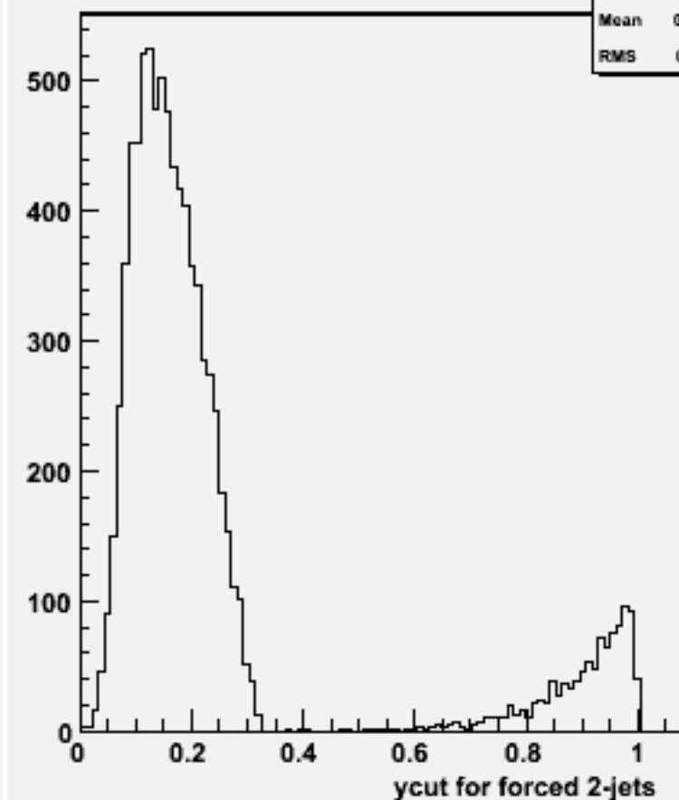
Ycut for 2-jets :w101112 ssn1e1sc_o
