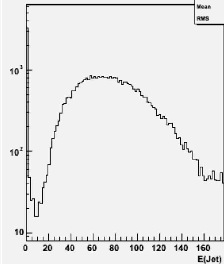
Jet energies(All jets)w101112 ssn1e1sc_o
