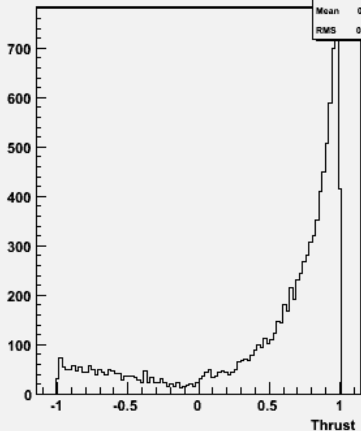
cos \Theta (thrust) w101112 ssn1e1sc_o
