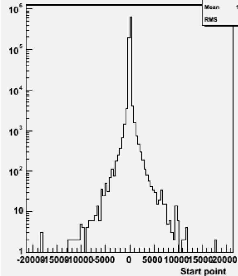
Start point Z : w101112 ssn1e1sc_o
