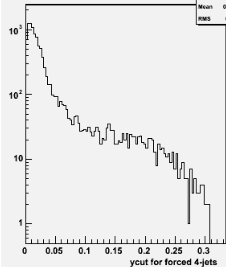
Ycut for 4-jets :w101112 ssn1e1sc_o
