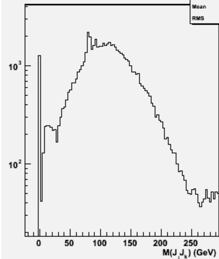
2jets mass(All comb)w101112 ssn1e1sc_o
