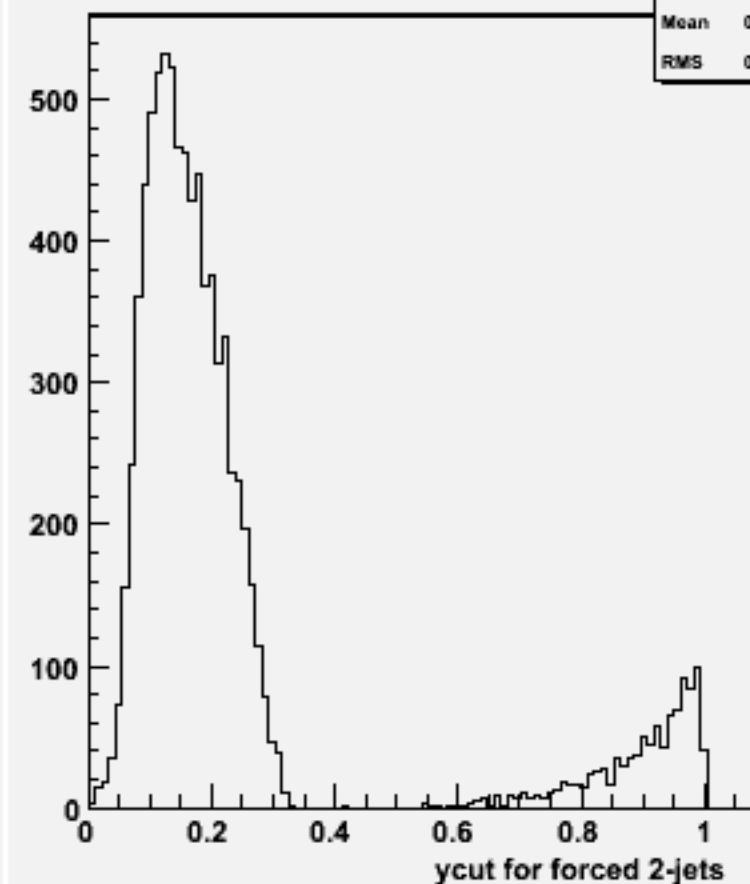
Ycut for 2-jets :w101111 ssn1e1sc_o
