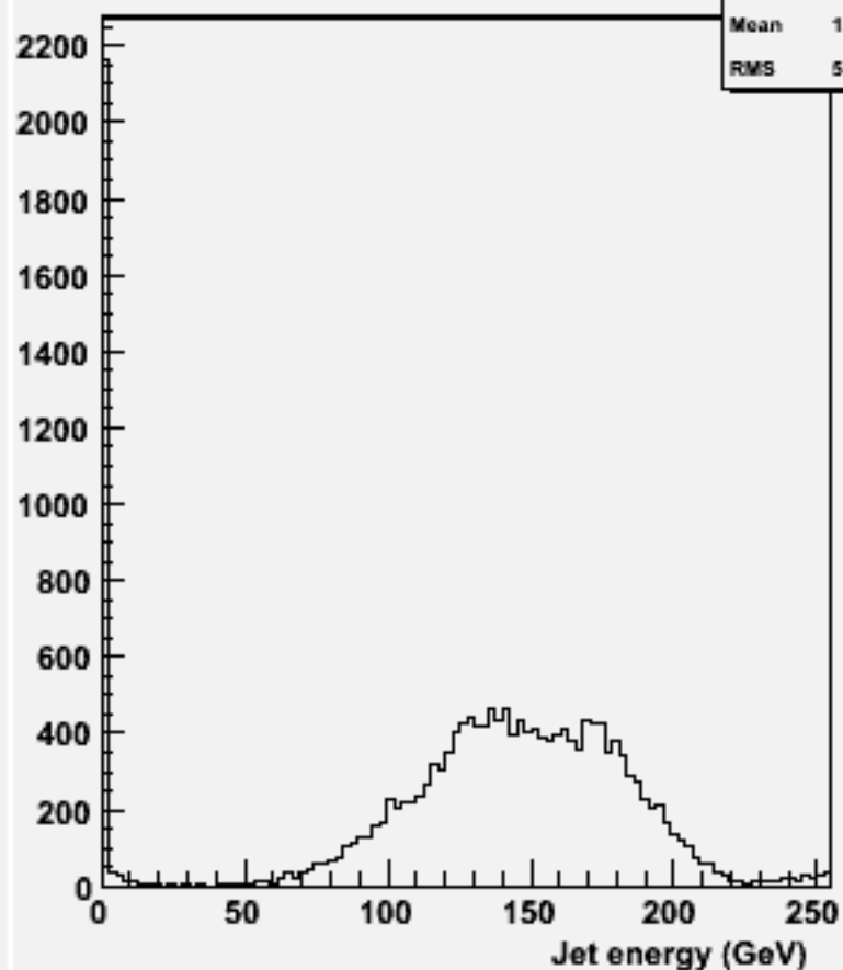
energy for 2-jets :w101111 ssn1e1sc_o
