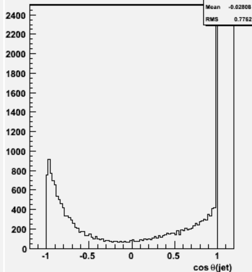
cos \theta for 2-jets :w101111 ssn1e1sc_o
