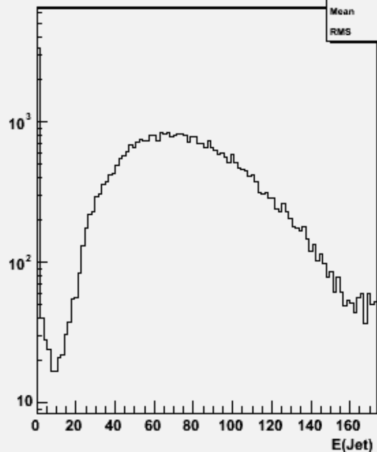
Jet energies(All jets)w101111 ssn1e1sc_o
