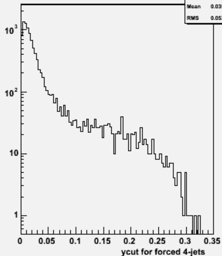
Ycut for 4-jets :w101111 ssn1e1sc_o
