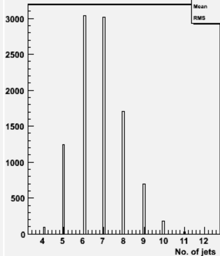
No. jets (ycut=0.001) : w101111 ssn1e1sc_o
