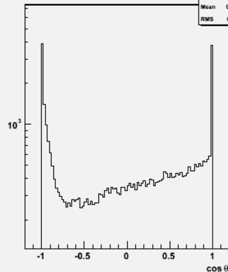
Jet cos \theta (All jets)w101111 ssn1e1sc_o
