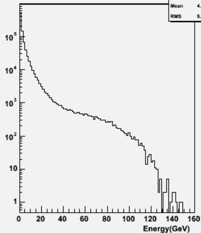
Particle Energy : w101111 ssn1e1sc_o
