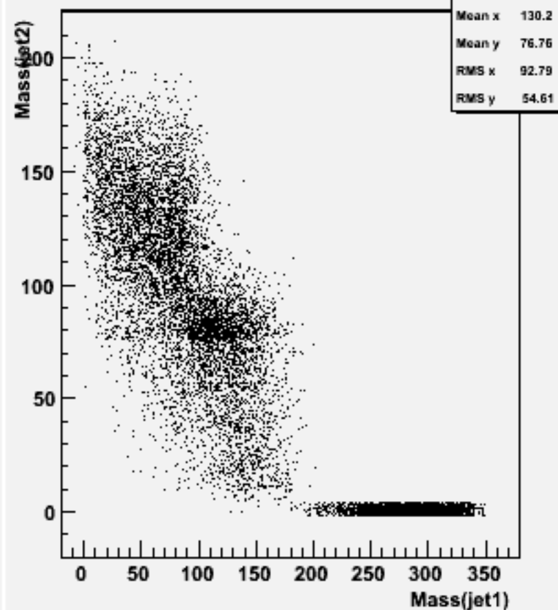
Jet mass for forced 2-jets : w101111 ssn1e1sc_o
