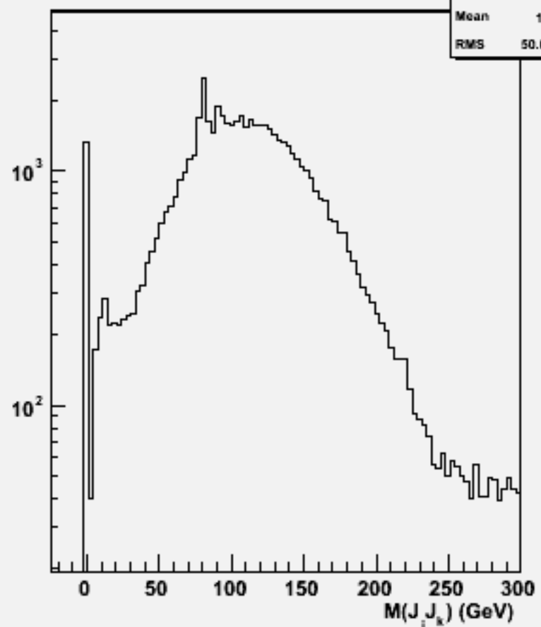
2jets mass(All comb)w101111 ssn1e1sc_o
