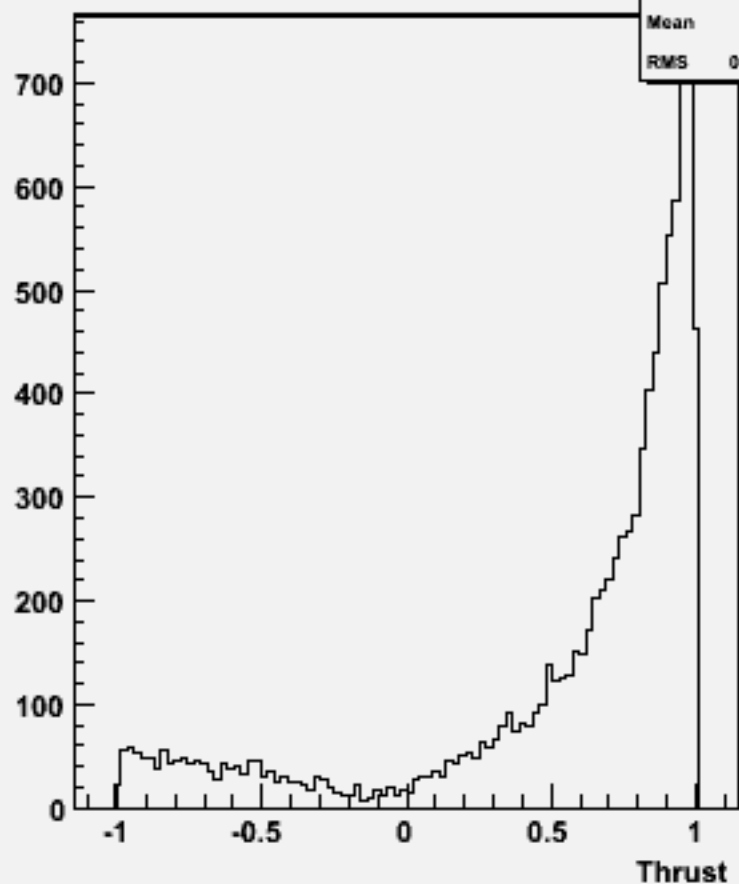
cos \Theta (thrust) w101111 ssn1e1sc_o
