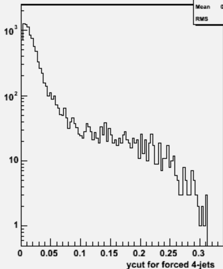
Ycut for 4-jets :w101108 ssn1e1du_o
