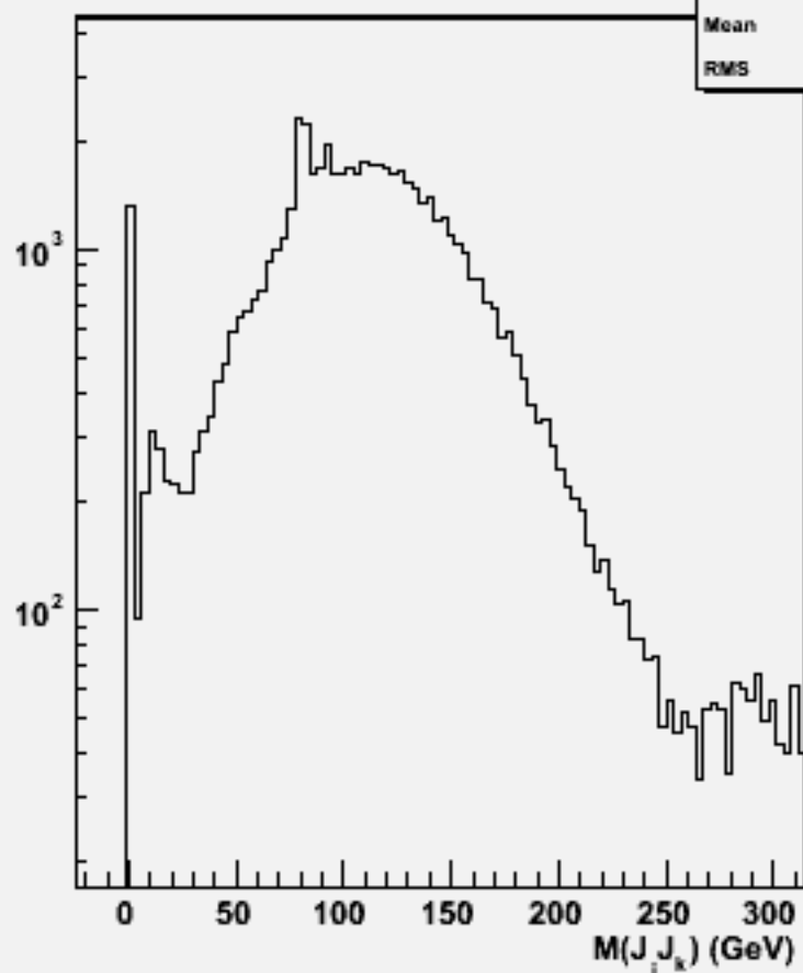
2jets mass(All comb)w101108 ssn1e1du_o
