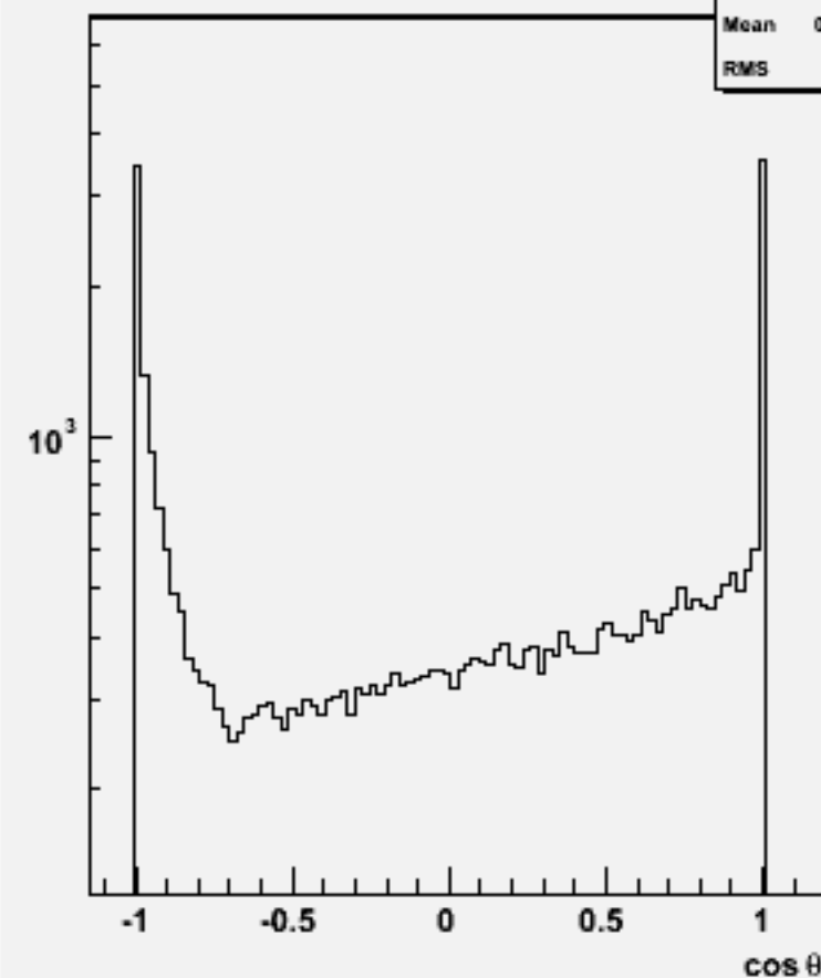
Jet cos \theta (All jets)w101108 ssn1e1du_o
