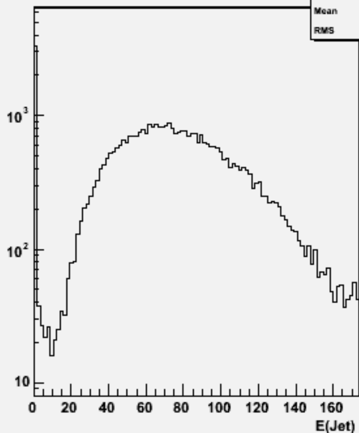
Jet energies(All jets)w101108 ssn1e1du_o
