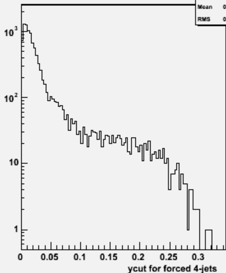
Ycut for 4-jets :w101107 ssn1e1du_o
