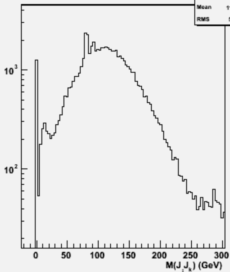
2jets mass(All comb)w101107 ssn1e1du_o
