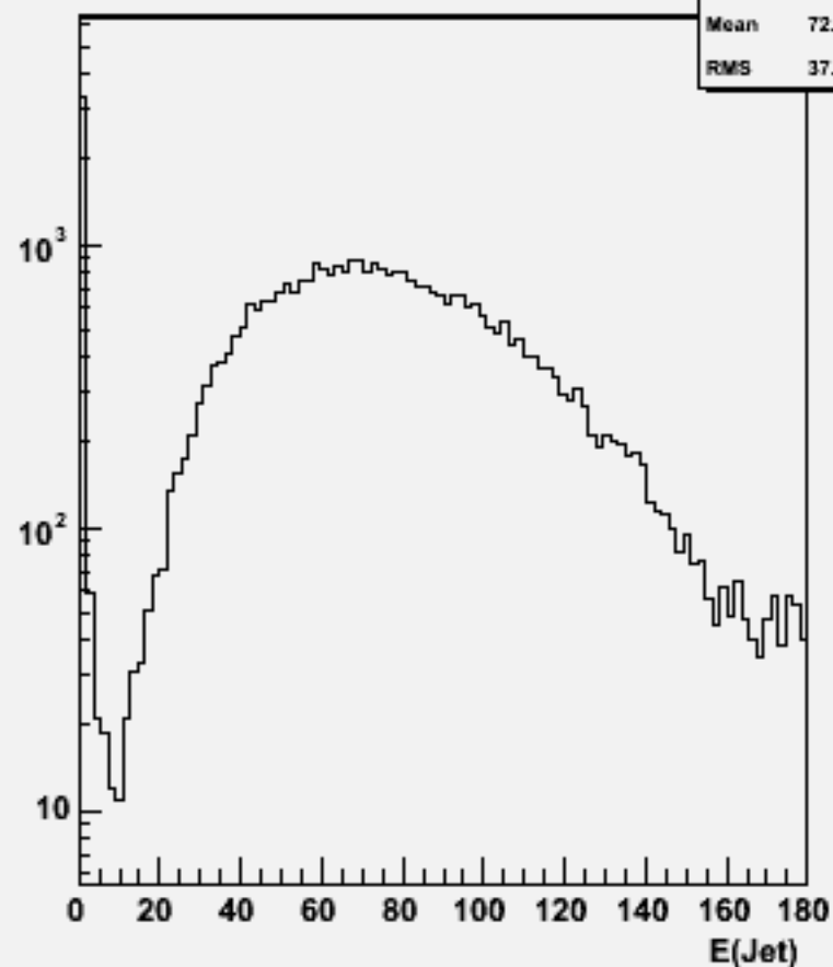
Jet energies(All jets)w101107 ssn1e1du_o
