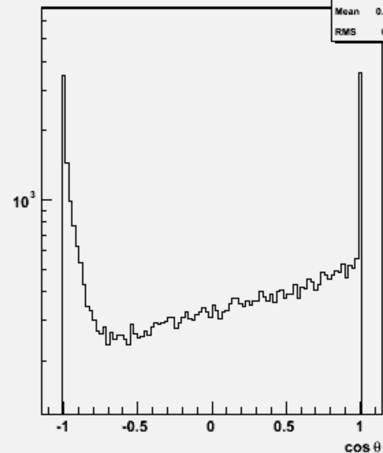
Jet cos \theta (All jets)w101107 ssn1e1du_o
