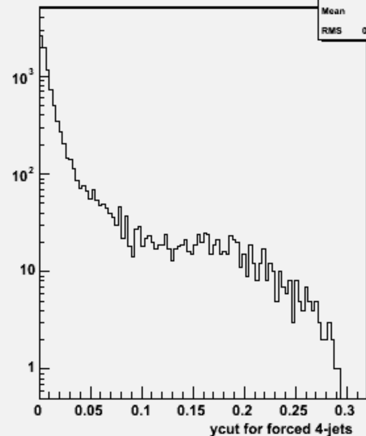
Ycut for 4-jets :w101105 ssn1e1e3n3_o
