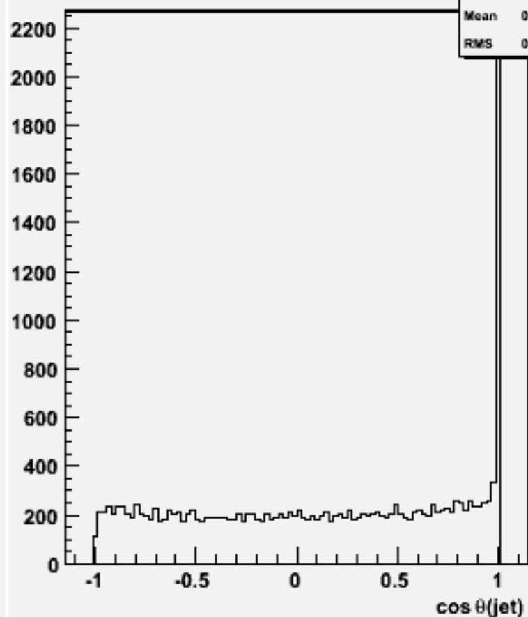
cos \theta for 2-jets :w101105 ssn1e1e3n3_o
