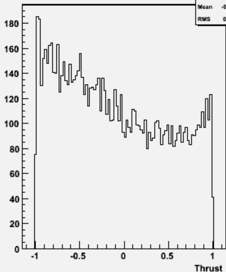
cos \Theta (thrust) w101105 ssn1e1e3n3_o
