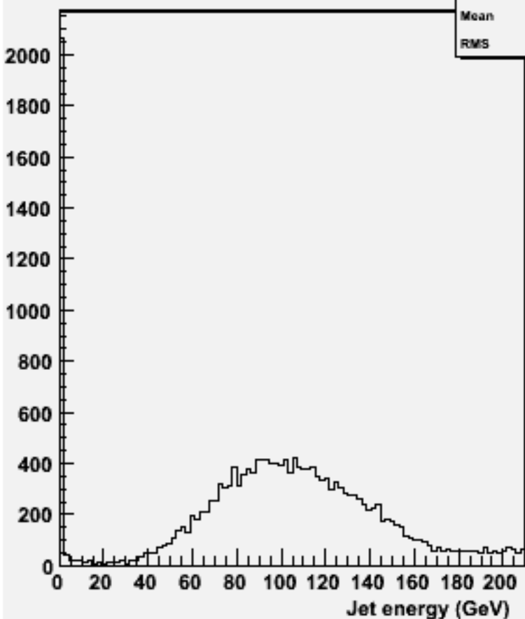
energy for 2-jets :w101105 ssn1e1e3n3_o
