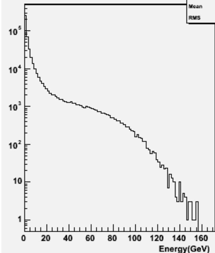
Particle Energy : w101105 ssn1e1e3n3_o
