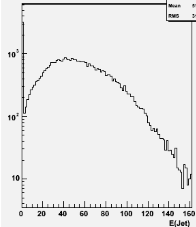
Jet energies(All jets)w101105 ssn1e1e3n3_o
