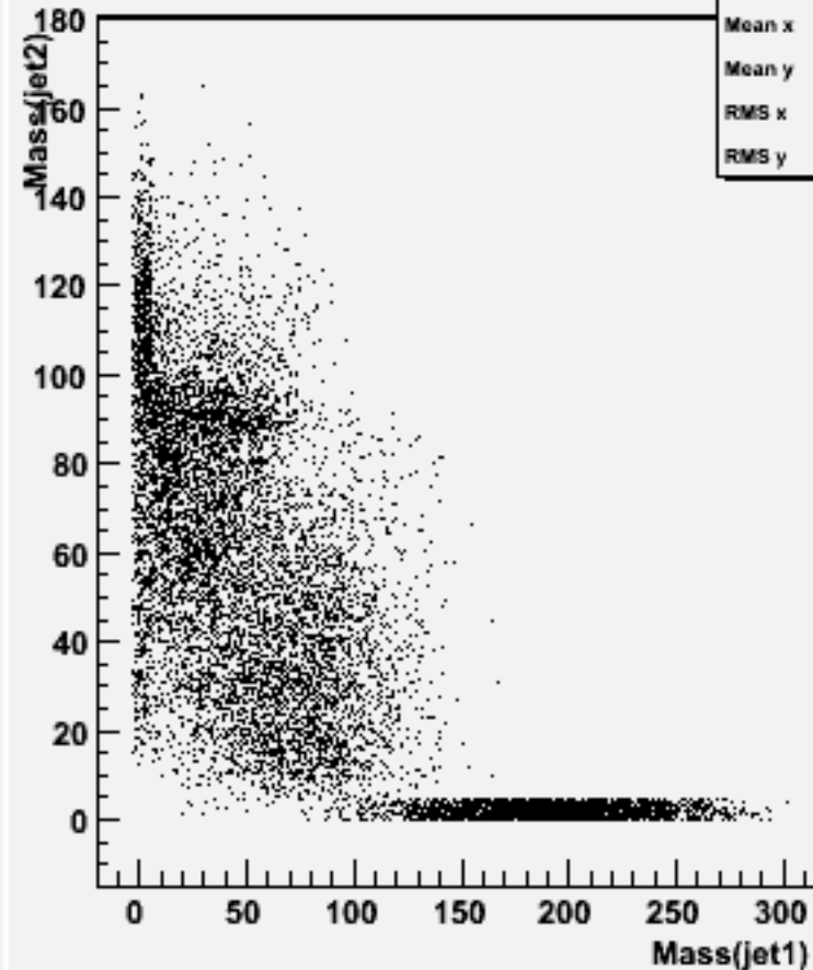
Jet mass for forced 2-jets : w101105 ssn1e1e3n3_o
