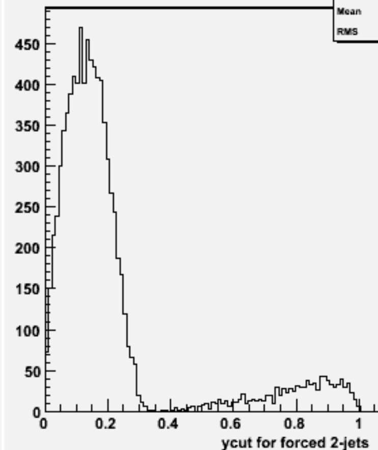
Ycut for 2-jets :w101105 ssn1e1e3n3_o
