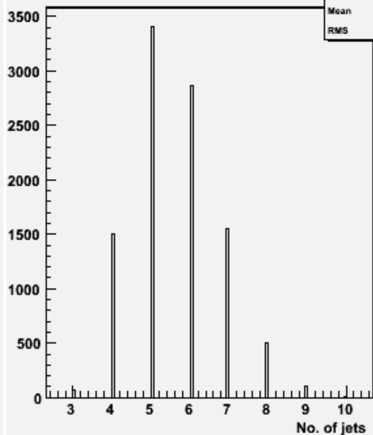
No. jets (ycut=0.001) : w101105 ssn1e1e3n3_o
