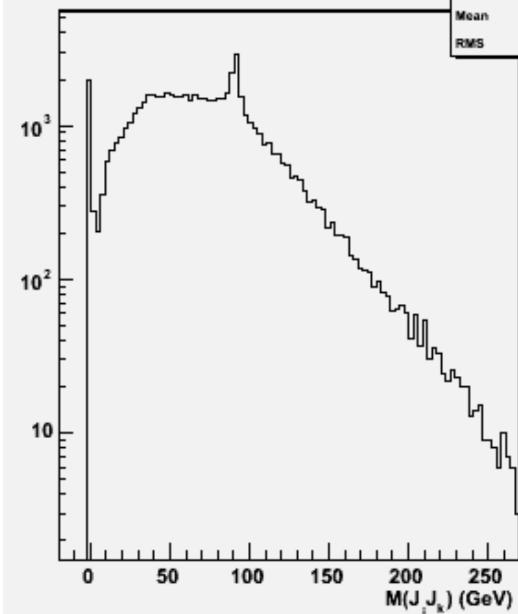
2jets mass(All comb)w101105 ssn1e1e3n3_o
