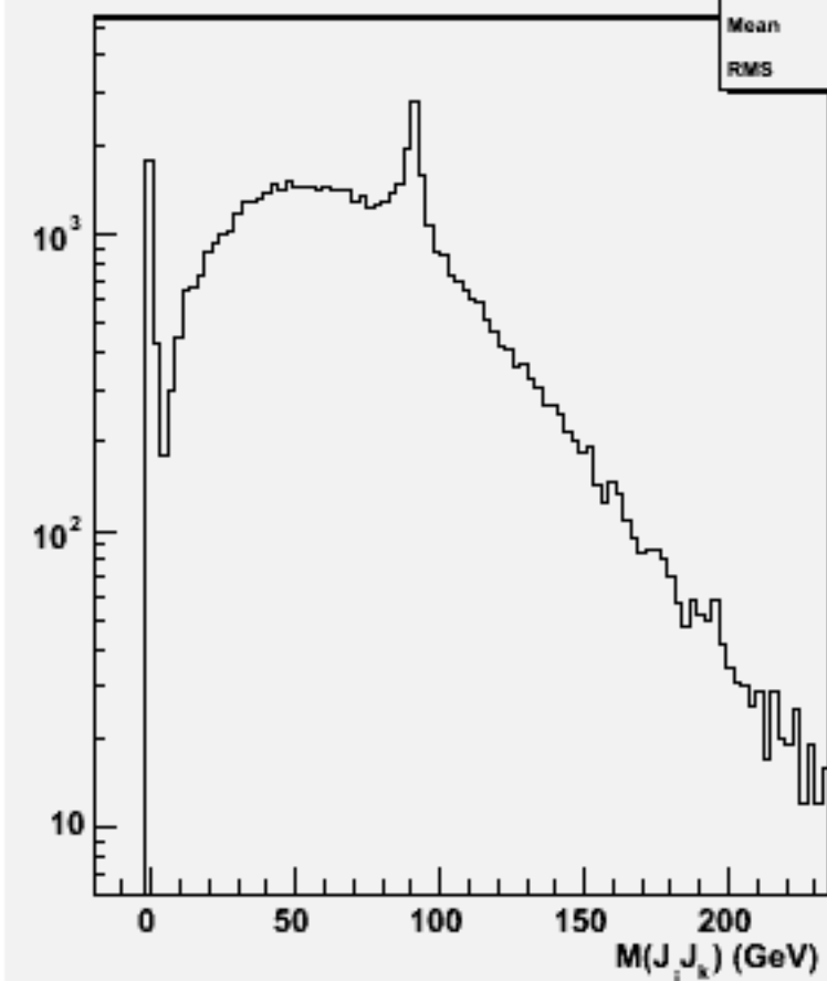
2jets mass(All comb)w101103 ssn1e1e3n3_o
