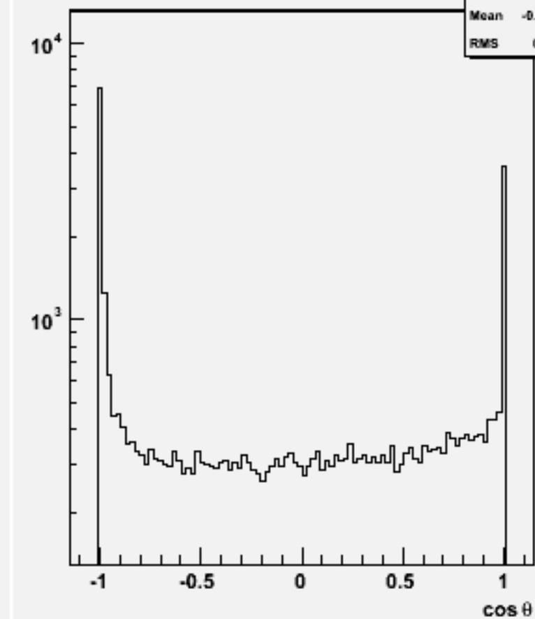
Jet cos \theta (All jets)w101103 ssn1e1e3n3_o
