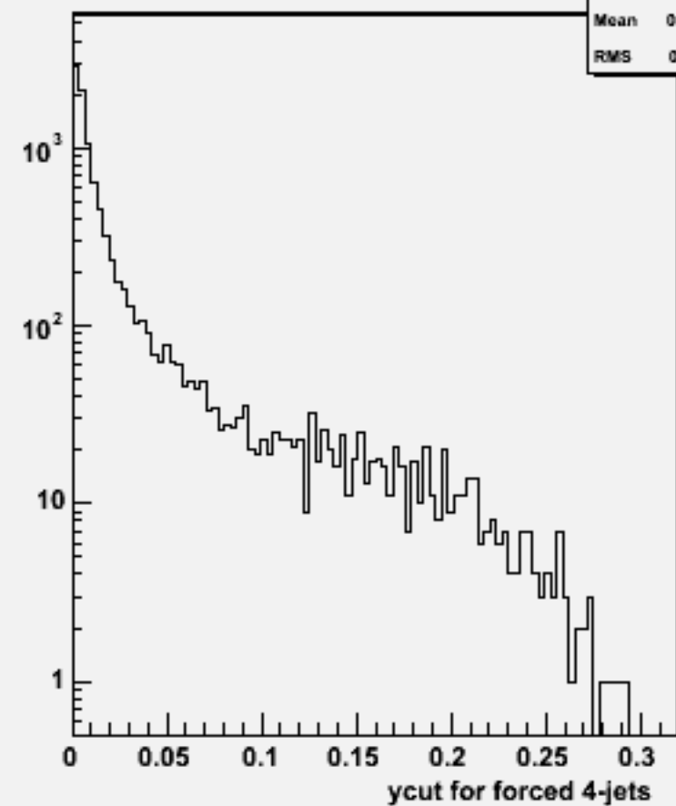
Ycut for 4-jets :w101103 ssn1e1e3n3_o
