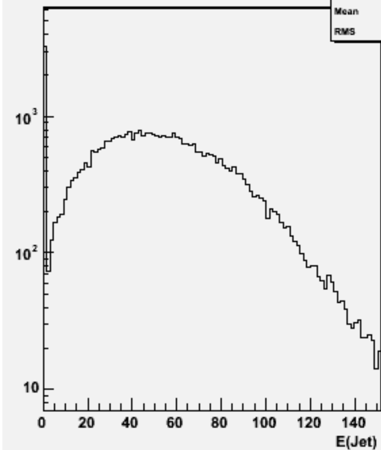
Jet energies(All jets)w101103 ssn1e1e3n3_o
