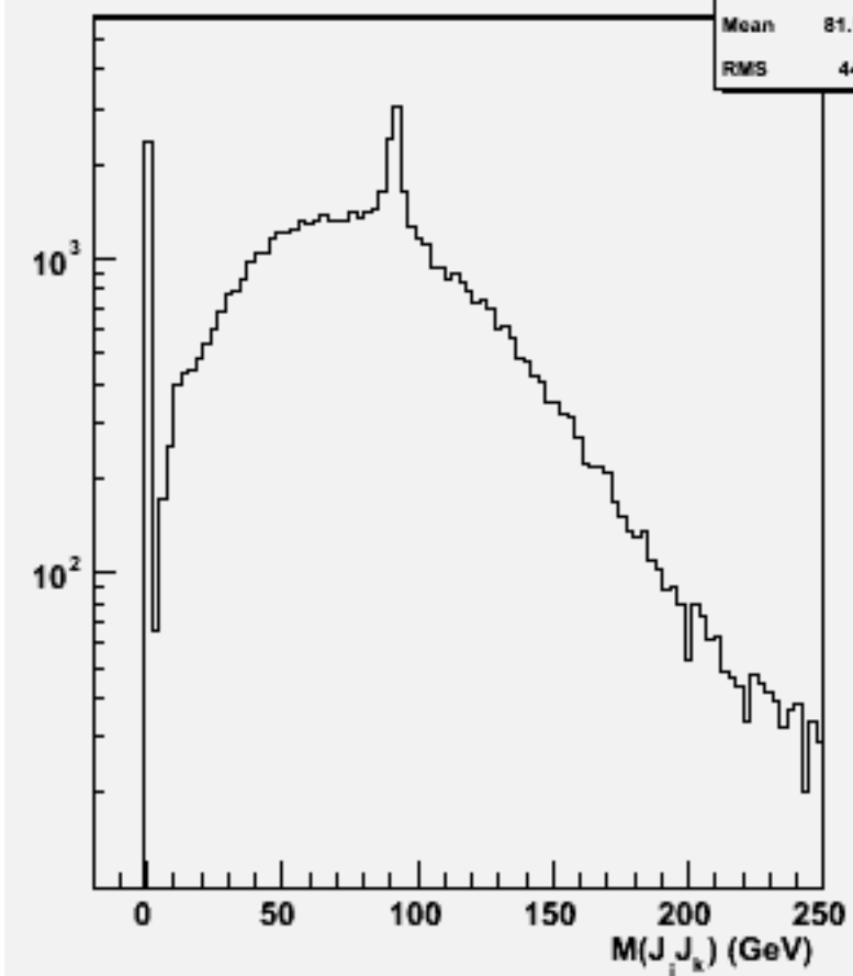
2jets mass(All comb)w101101 ssn1e1e2n2_o
