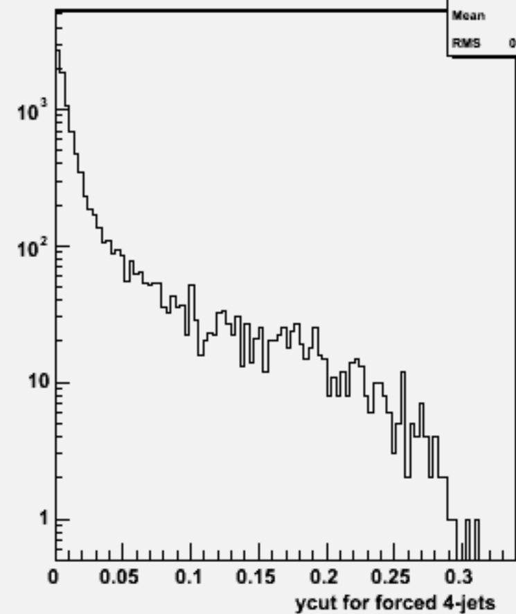
Ycut for 4-jets :w101101 ssn1e1e2n2_o
