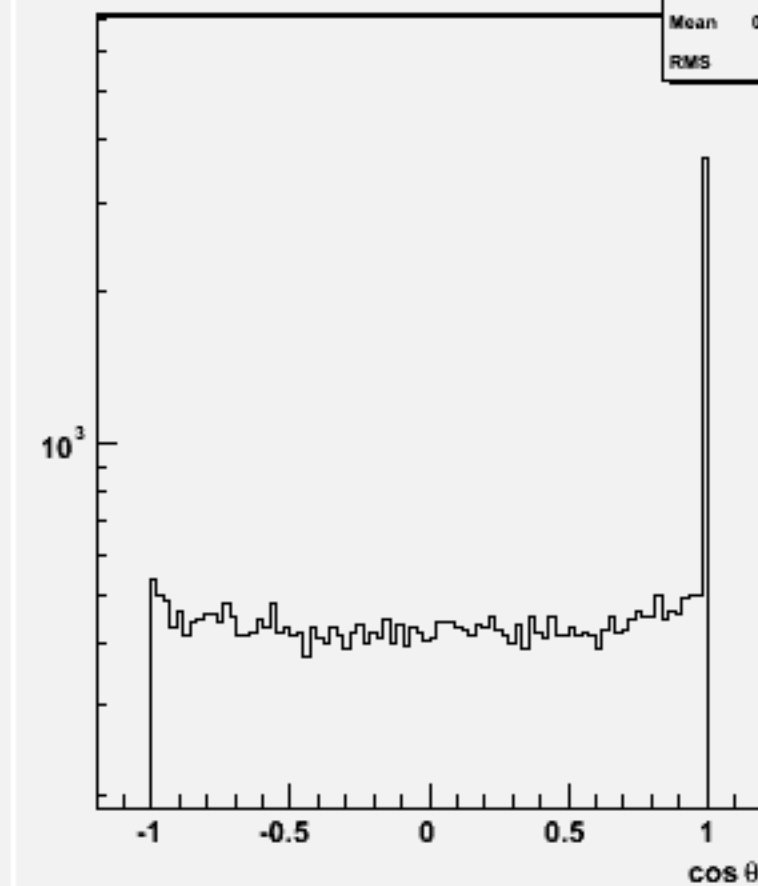
Jet cos \theta (All jets)w101101 ssn1e1e2n2_o
