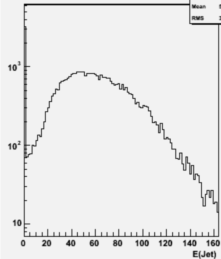
Jet energies(All jets)w101101 ssn1e1e2n2_o
