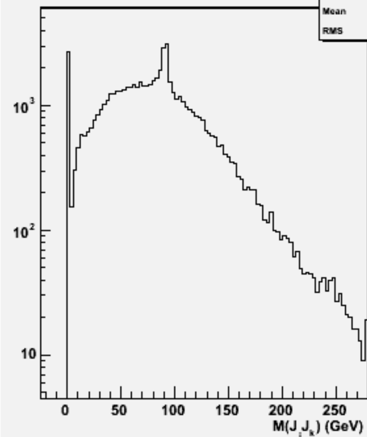
2jets mass(All comb)w101099 ssn1e1e2n2_o
