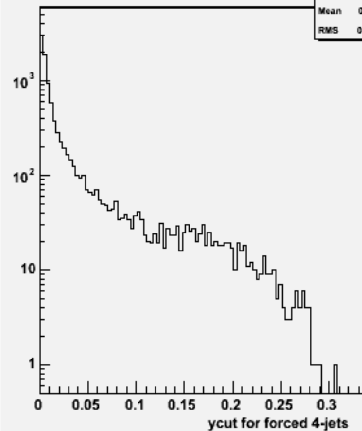
Ycut for 4-jets :w101099 ssn1e1e2n2_o
