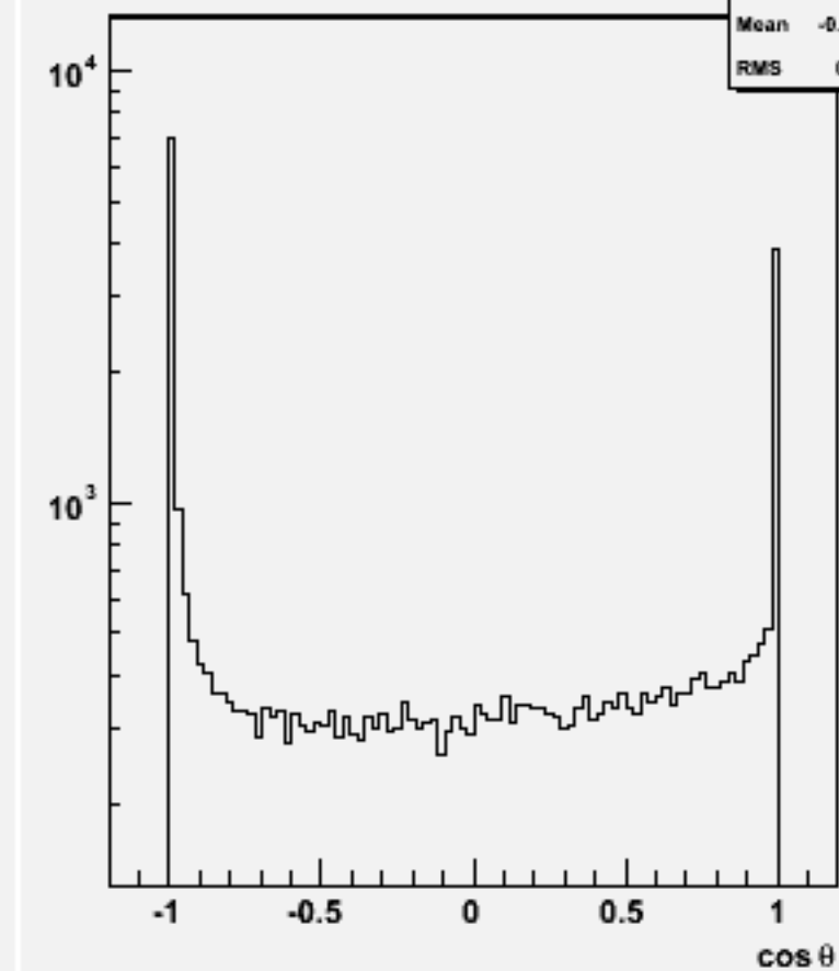
Jet cos \theta (All jets)w101099 ssn1e1e2n2_o
