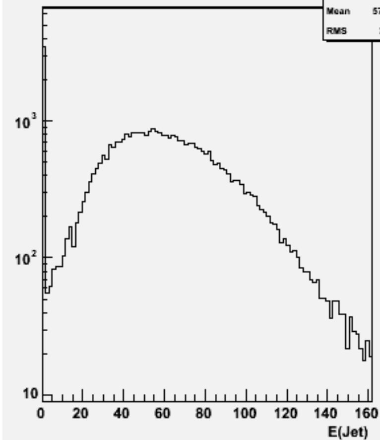
Jet energies(All jets)w101099 ssn1e1e2n2_o
