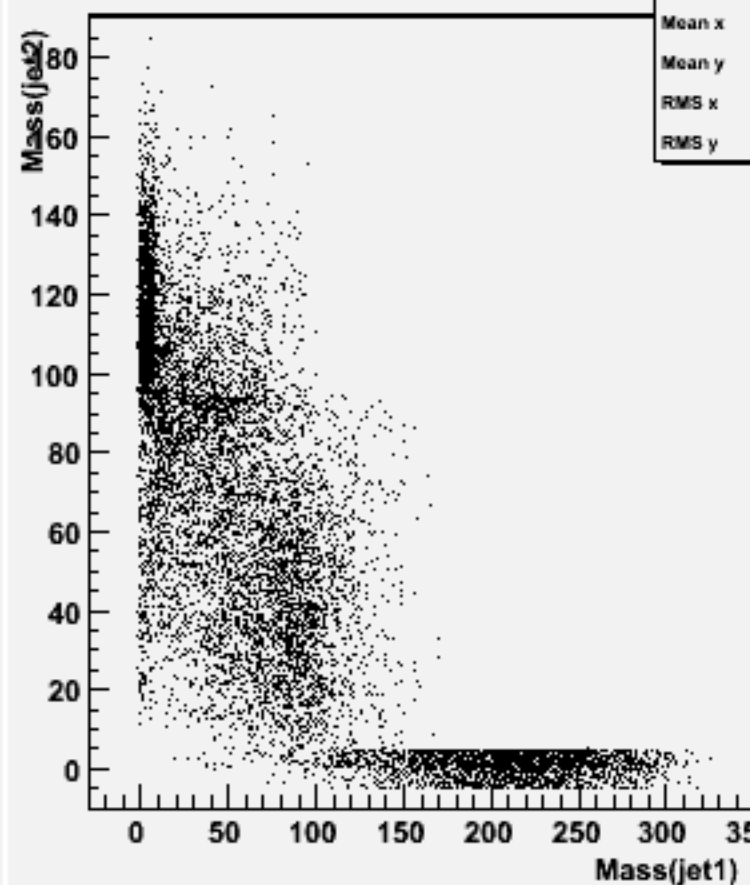
Jet mass for forced 2-jets : w101098 ssn1e1e1n1_o
