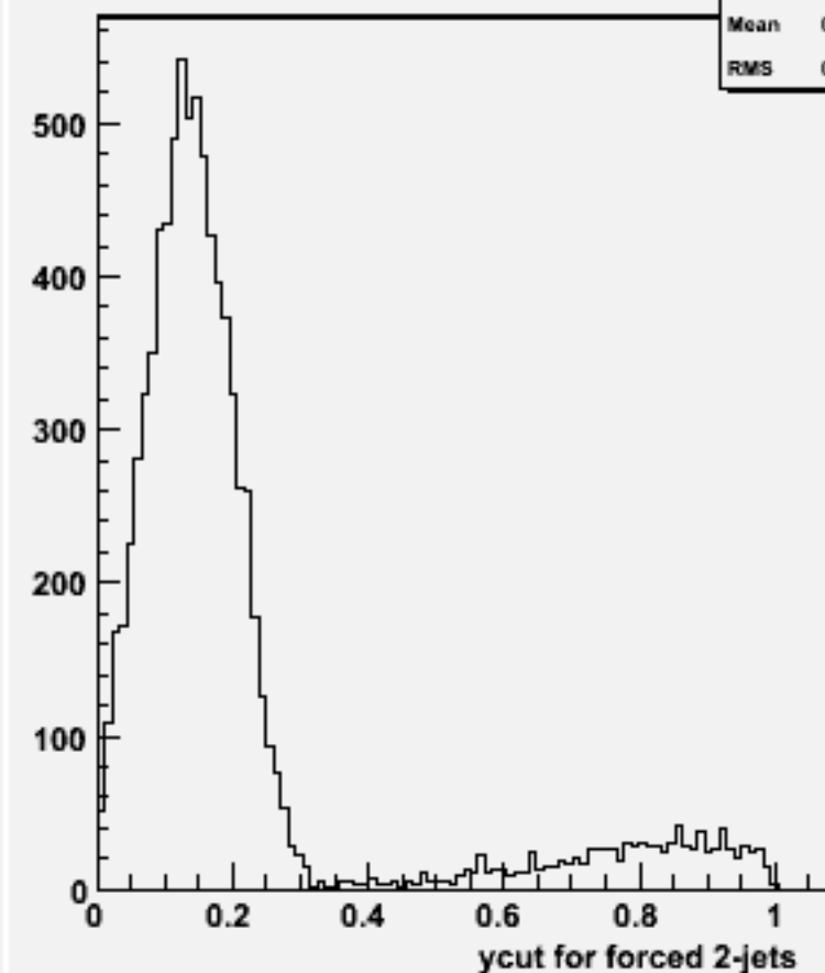
Ycut for 2-jets :w101098 ssn1e1e1n1_o
