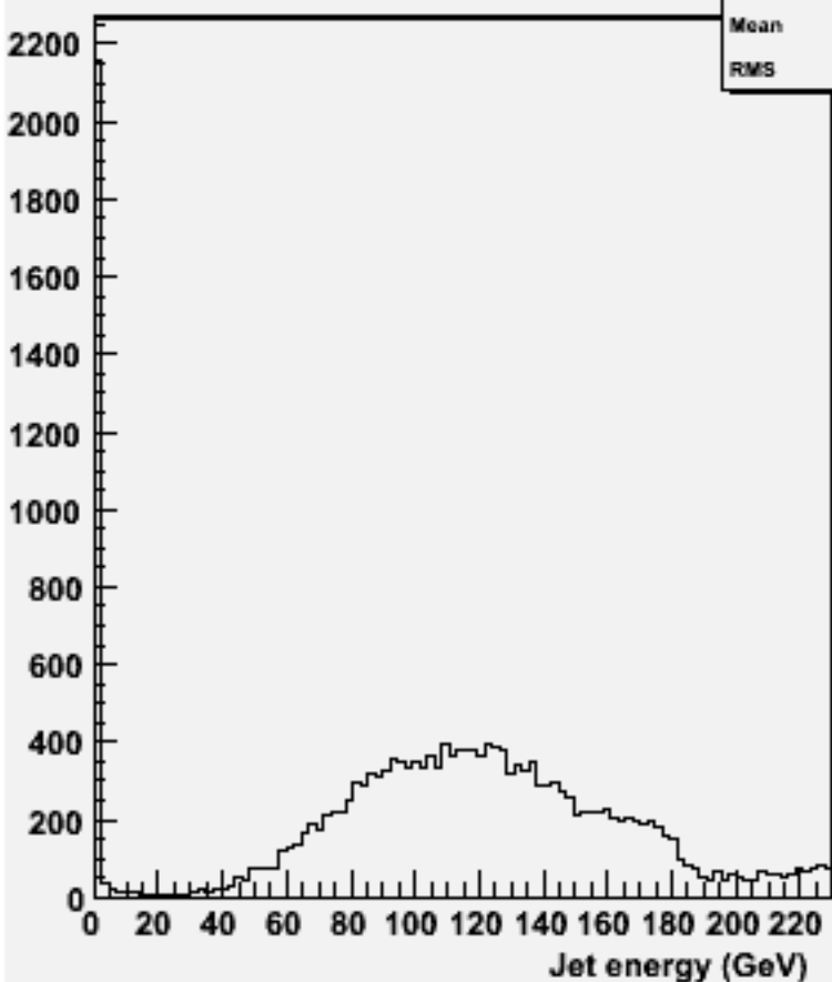
energy for 2-jets :w101098 ssn1e1e1n1_o
