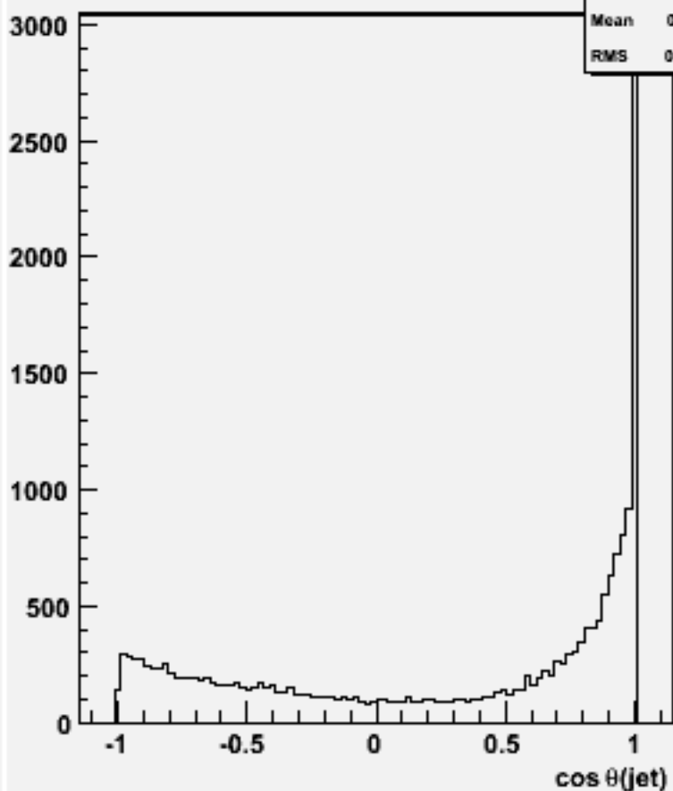
cos \Theta for 2-jets :w101098 ssn1e1e1n1_o
