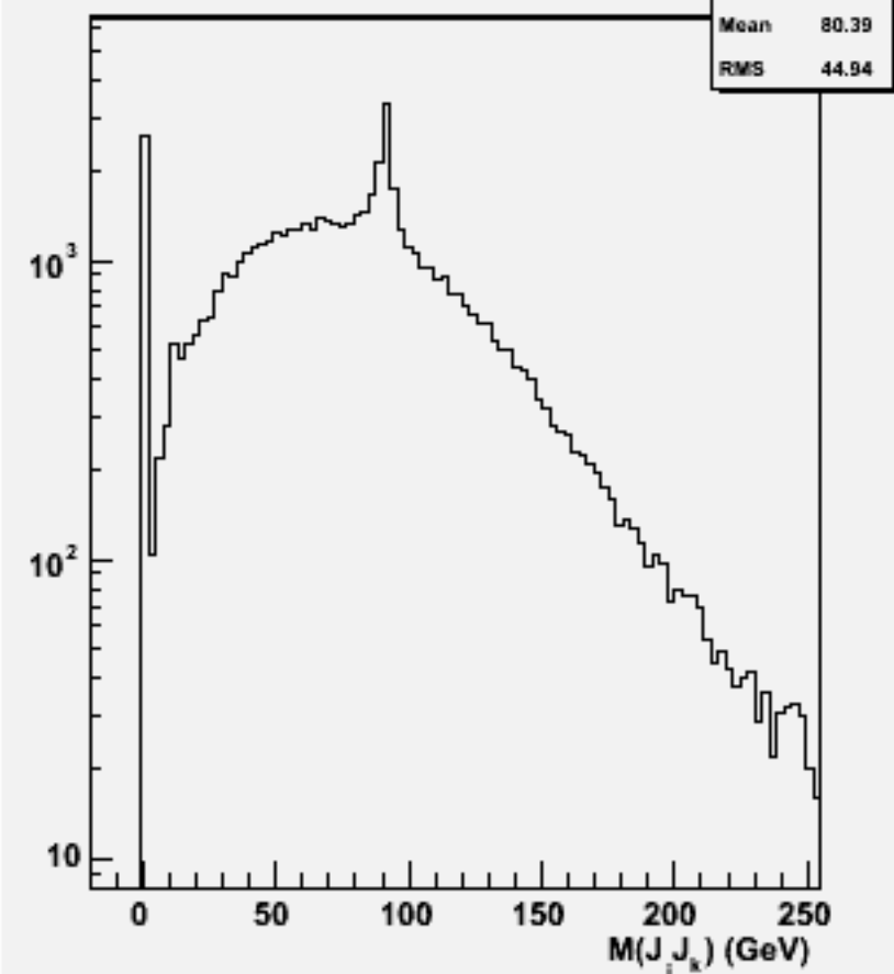
2jets mass(All comb)w101098 ssn1e1e1n1_o
