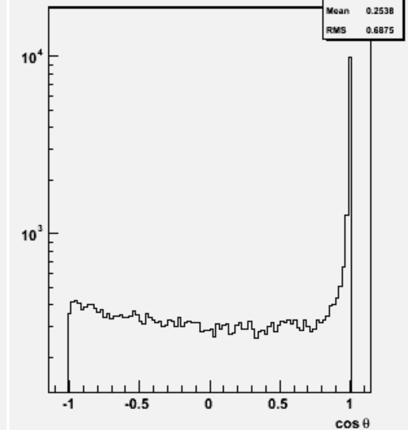
Jet cos \theta (All jets)w101098 ssn1e1e1n1_o
