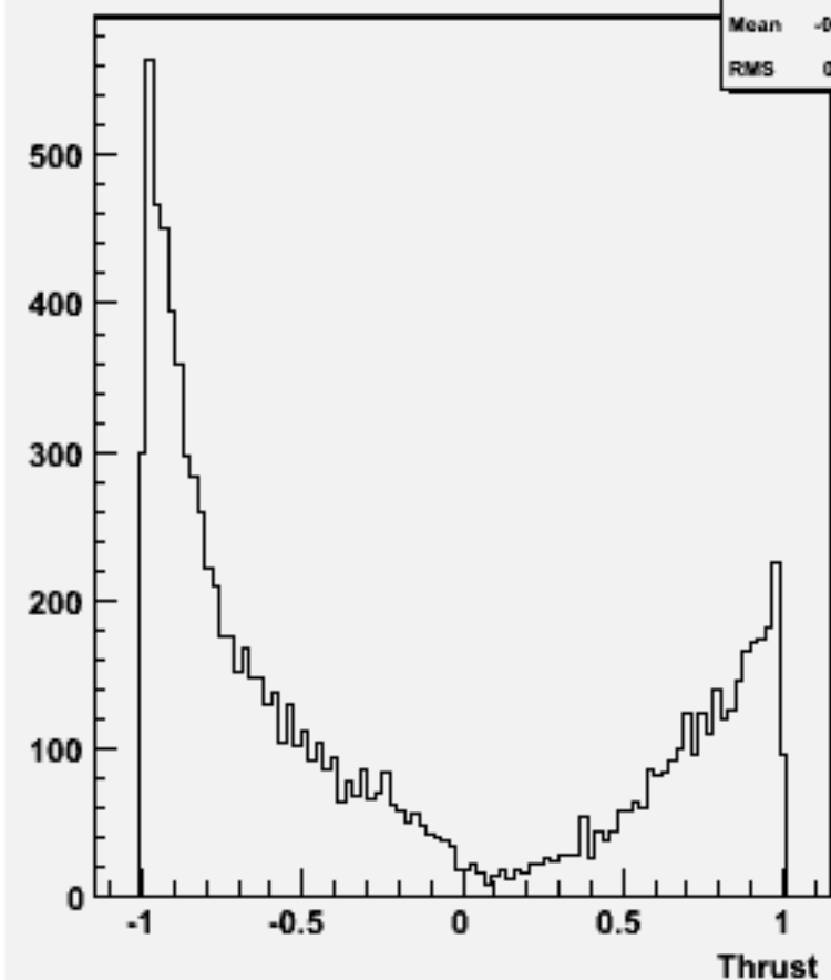
cos \Theta (thrust) w101098 ssn1e1e1n1_o
