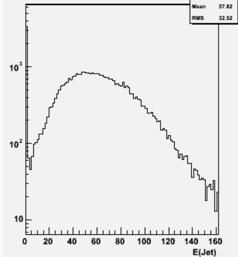
Jet energies(All jets)w101098 ssn1e1e1n1_o
