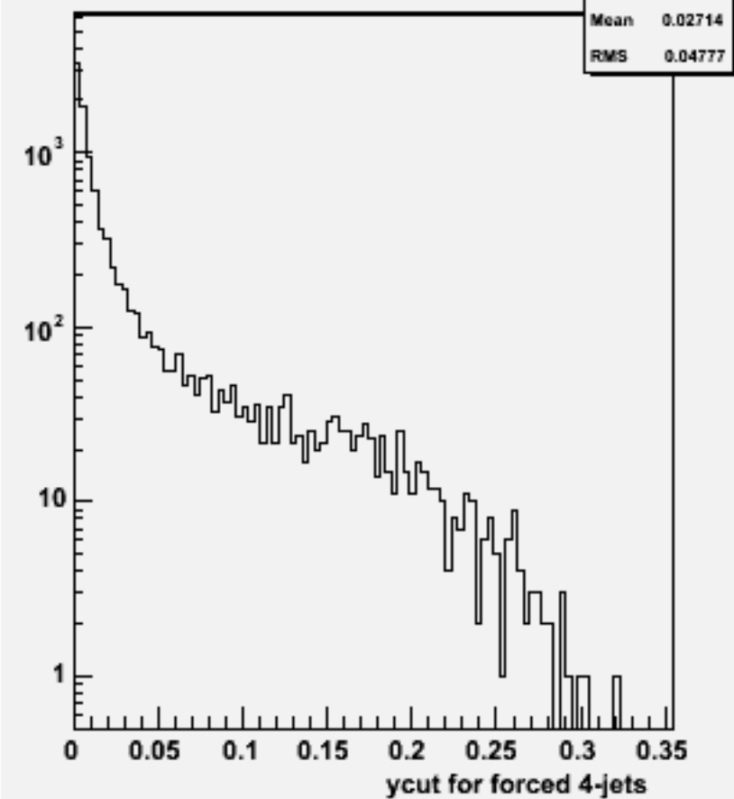
Ycut for 4-jets :w101098 ssn1e1e1n1_o
