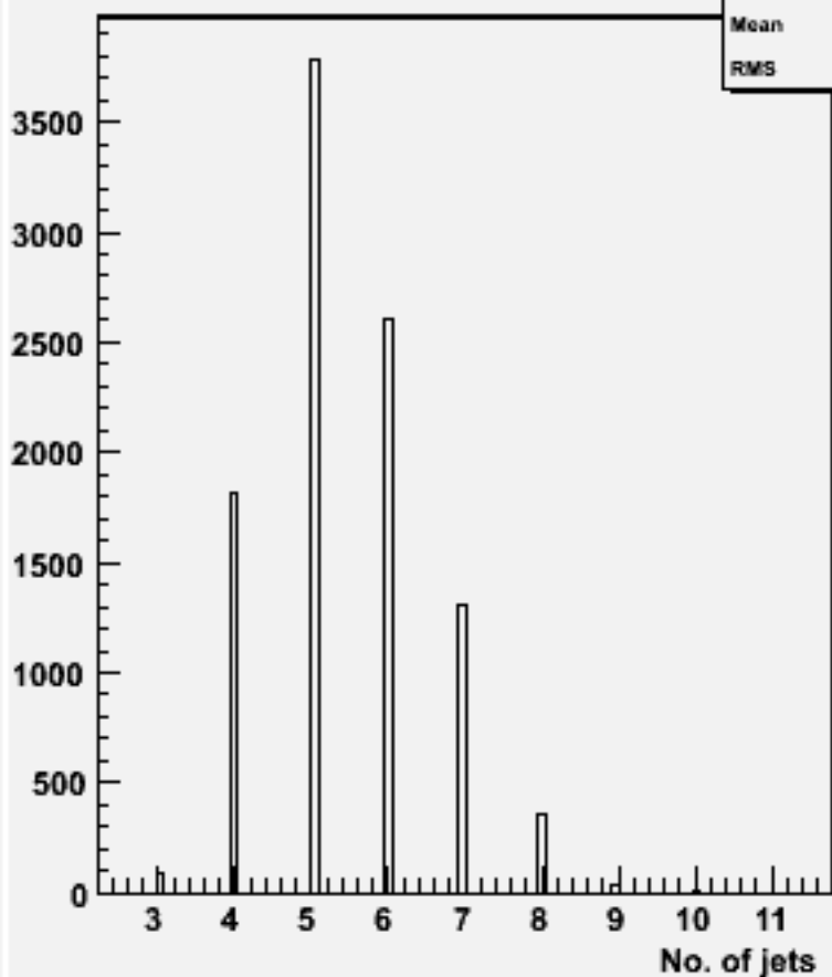
No. jets (ycut=0.001) : w101098 ssn1e1e1n1_o
