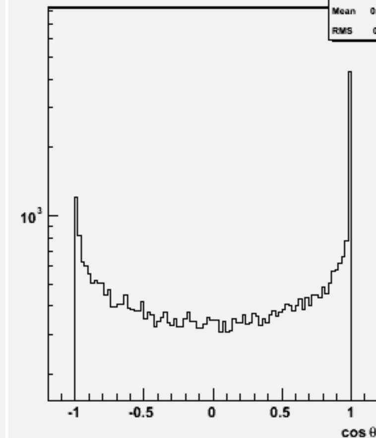
Jet cos \theta (All jets)w101097 ssn1e1e1n1_o
