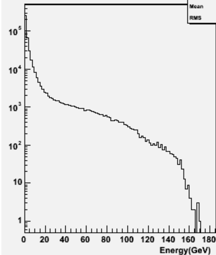
Particle Energy : w101097 ssn1e1e1n1_o
