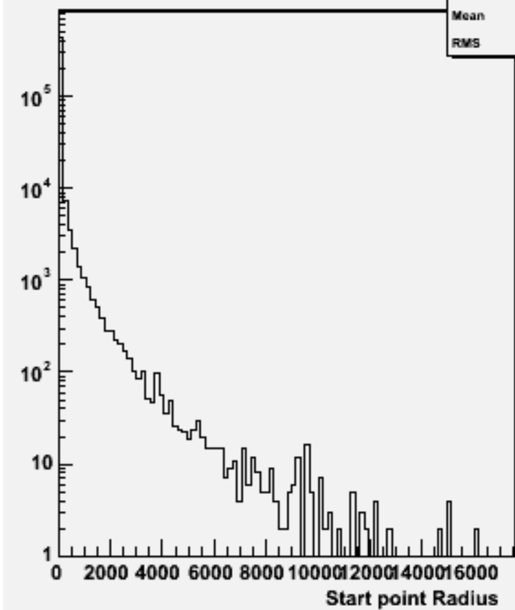
Start point R : w101097 ssn1e1e1n1_o
