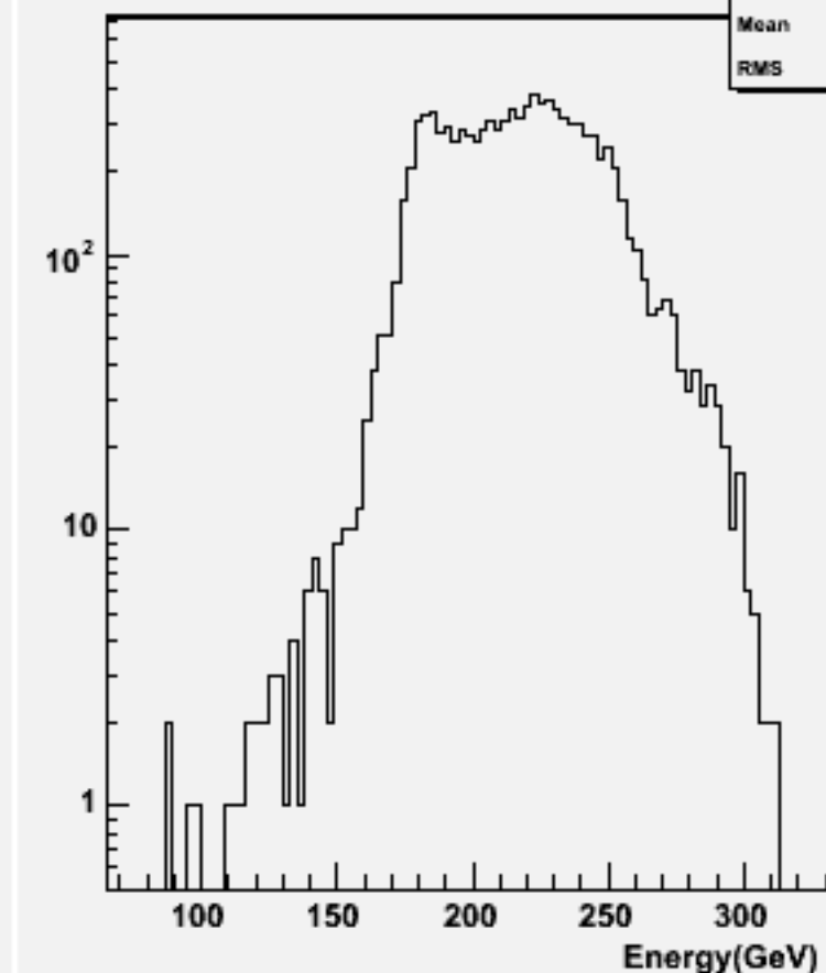
Thrust w101097 ssn1e1e1n1_o
