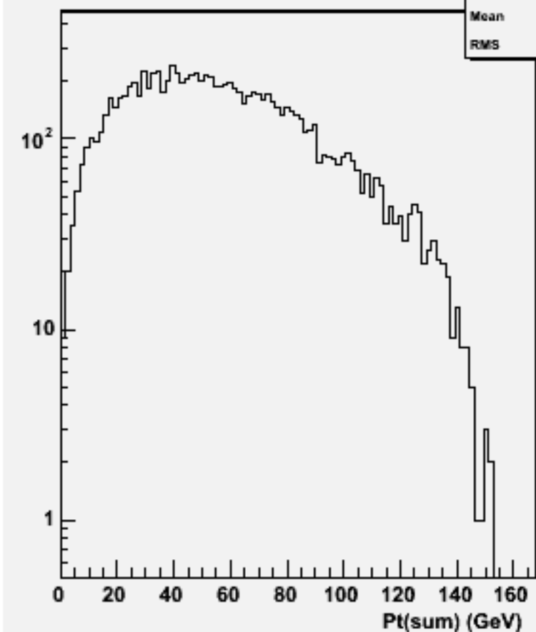
Pt Sum: w101097 ssn1e1e1n1_o
