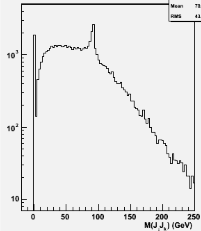
2jets mass(All comb)w101097 ssn1e1e1n1_o
