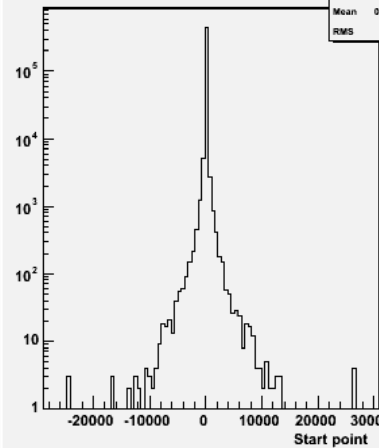
Start point Z : w101097 ssn1e1e1n1_o
