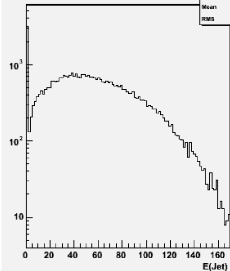
Jet energies(All jets)w101097 ssn1e1e1n1_o
