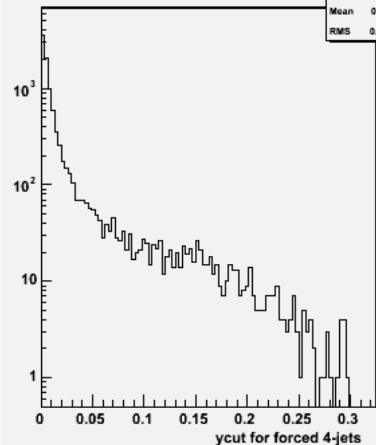
Ycut for 4-jets :w101097 ssn1e1e1n1_o
