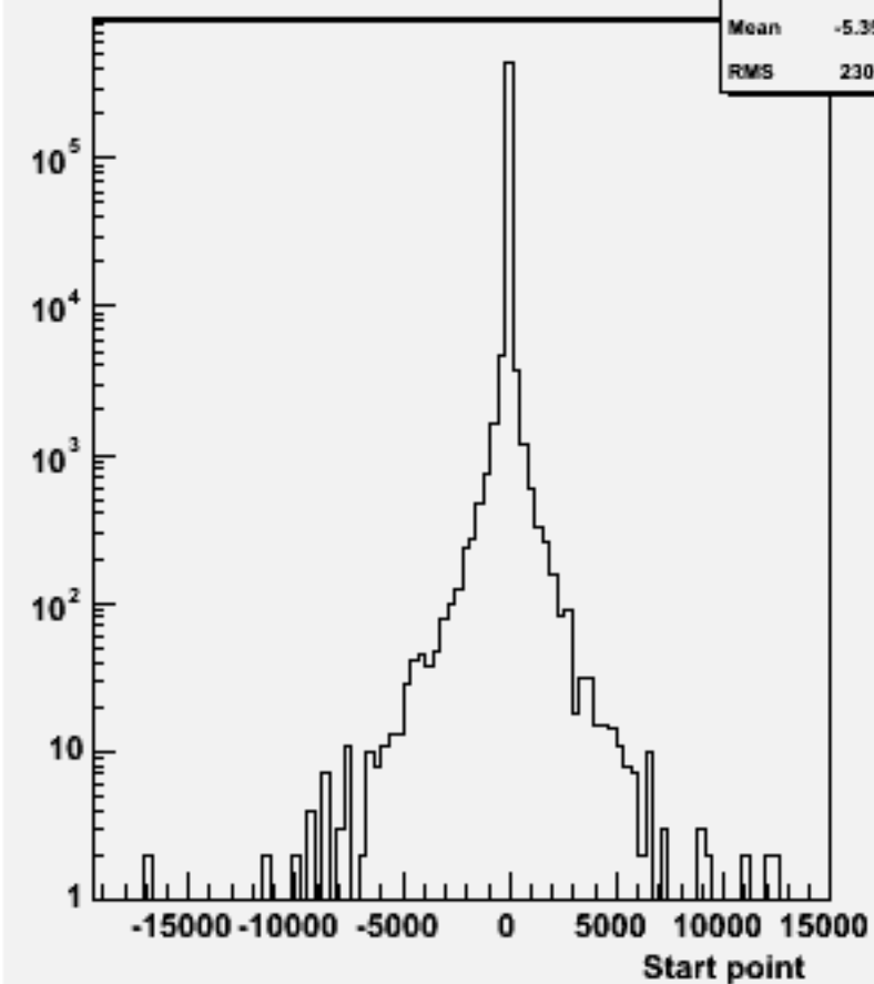
Start point Z : w101095 ssn1e1e1n1_o
