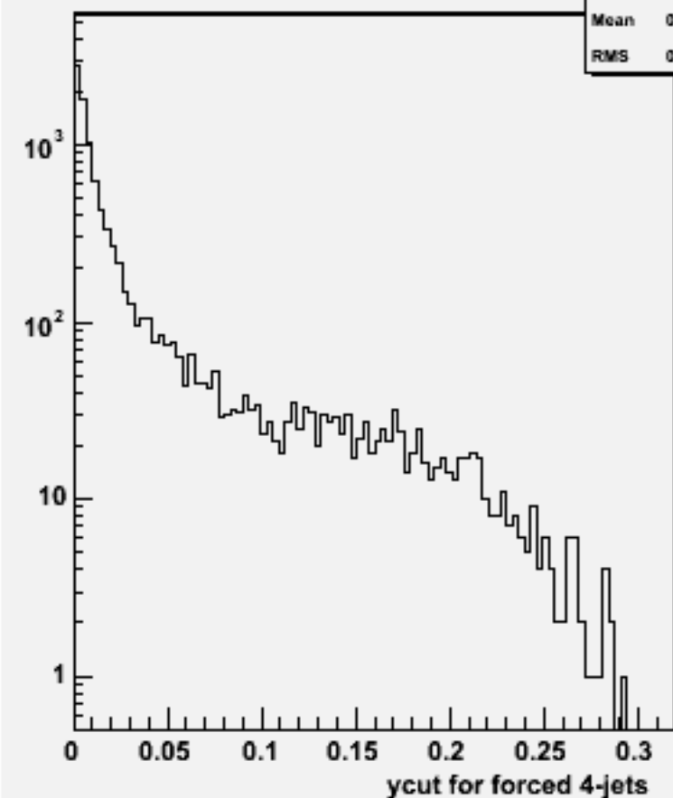
Ycut for 4-jets :w101095 ssn1e1e1n1_o
