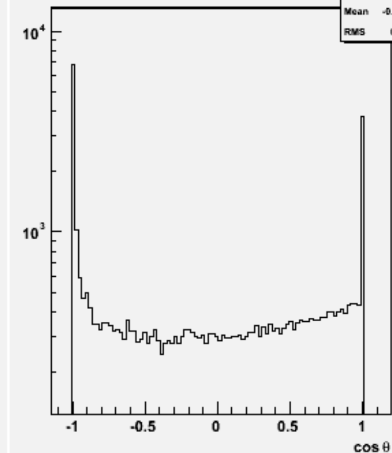
Jet cos \theta (All jets)w101095 ssn1e1e1n1_o
