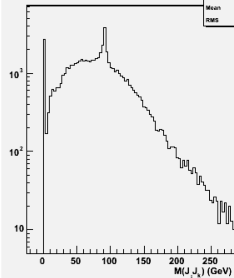
2jets mass(All comb)w101095 ssn1e1e1n1_o
