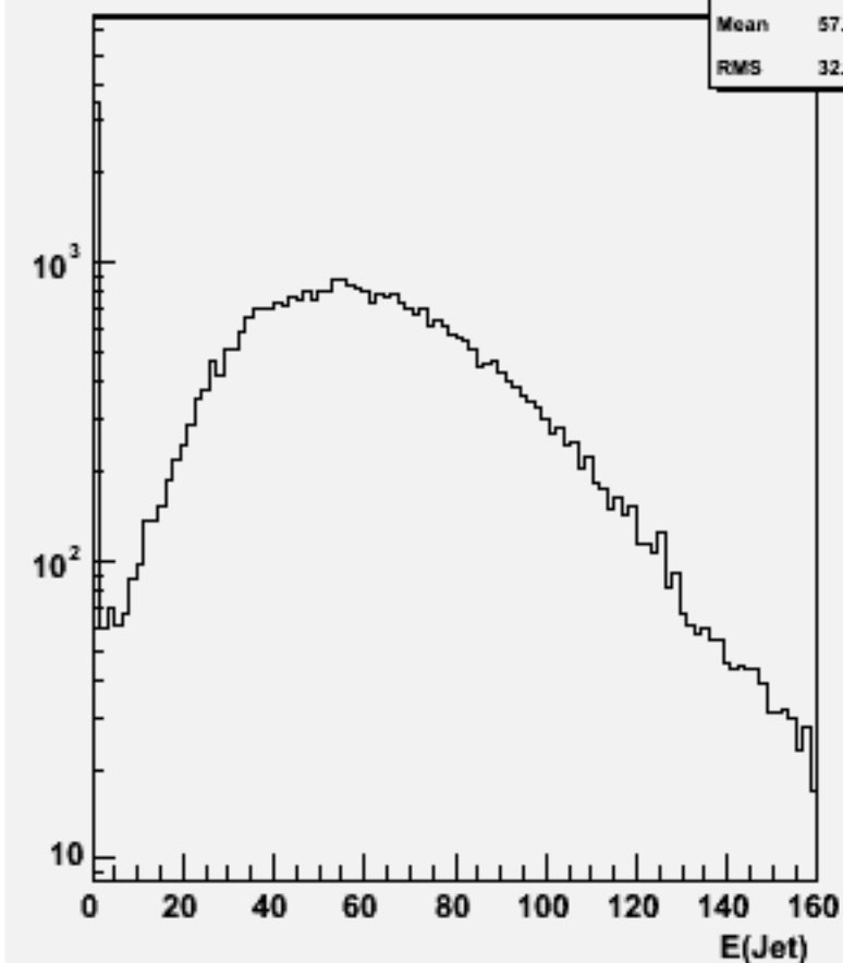
Jet energies(All jets)w101095 ssn1e1e1n1_o
