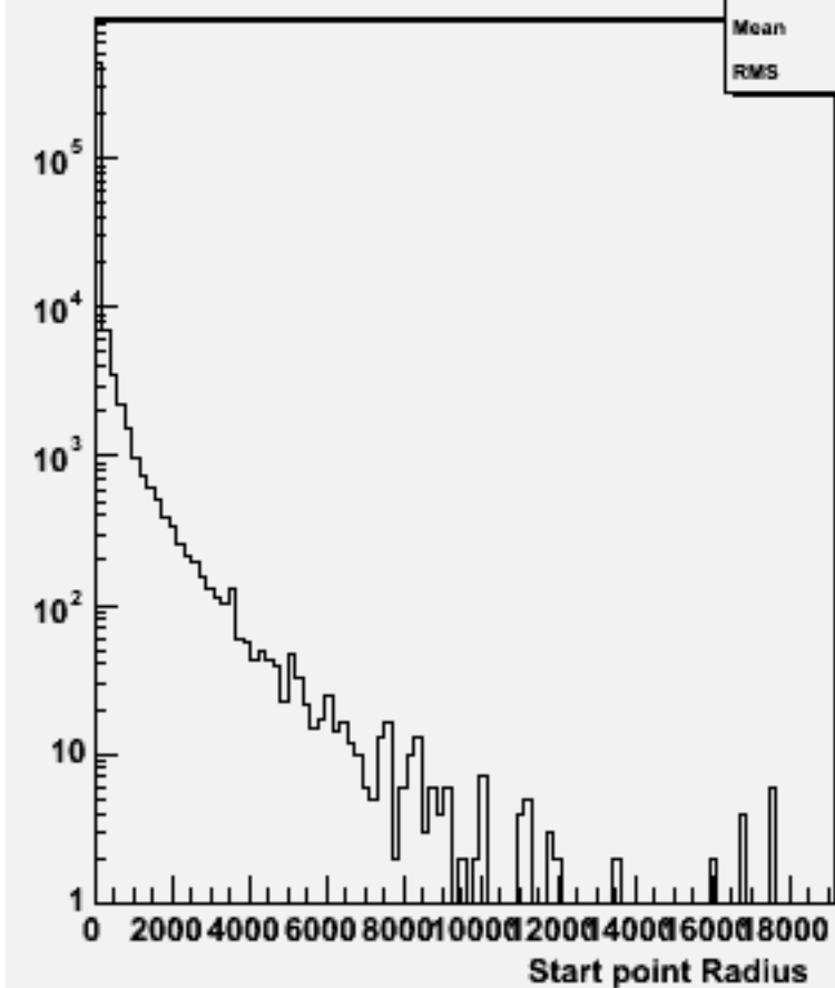
Start point R : w101095 ssn1e1e1n1_o
