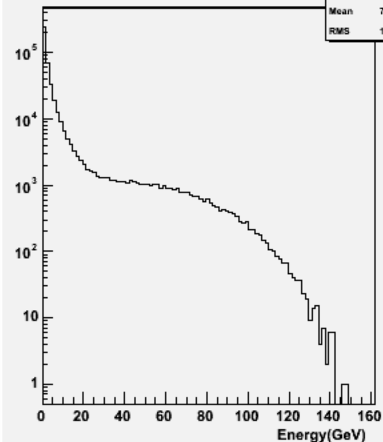
Particle Energy : w101095 ssn1e1e1n1_o
