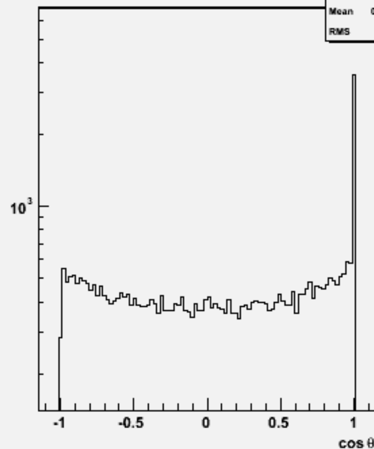
Jet cos \theta (All jets)w101092 ddcssc_o
