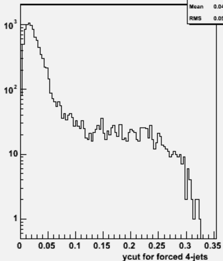
Ycut for 4-jets :w101092 ddcssc_o
