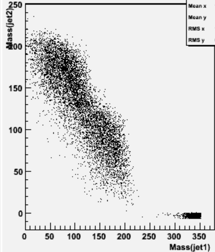
Jet mass for forced 2-jets : w101092 ddcssc_o
