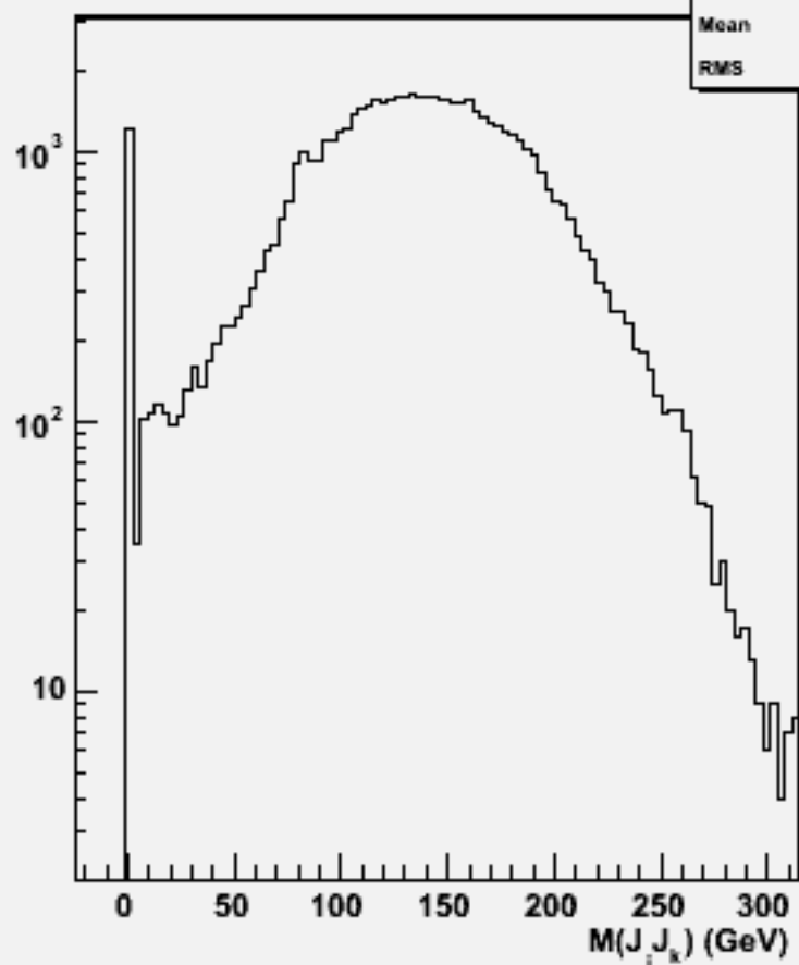
2jets mass(All comb)w101092 ddcssc_o
