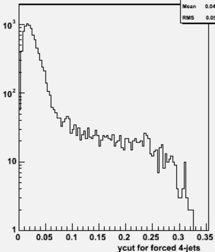
Ycut for 4-jets :w101089 ddcdu_o
