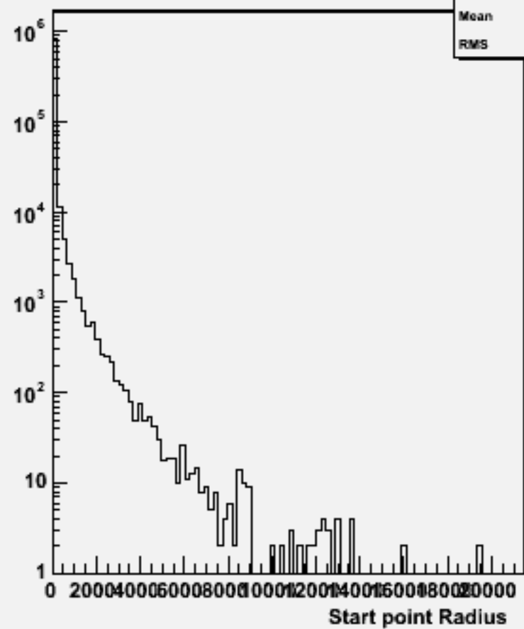
Start point R : w101085 ddcse3n3_o
