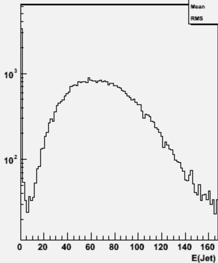
Jet energies(All jets)w101085 ddcse3n3_o
