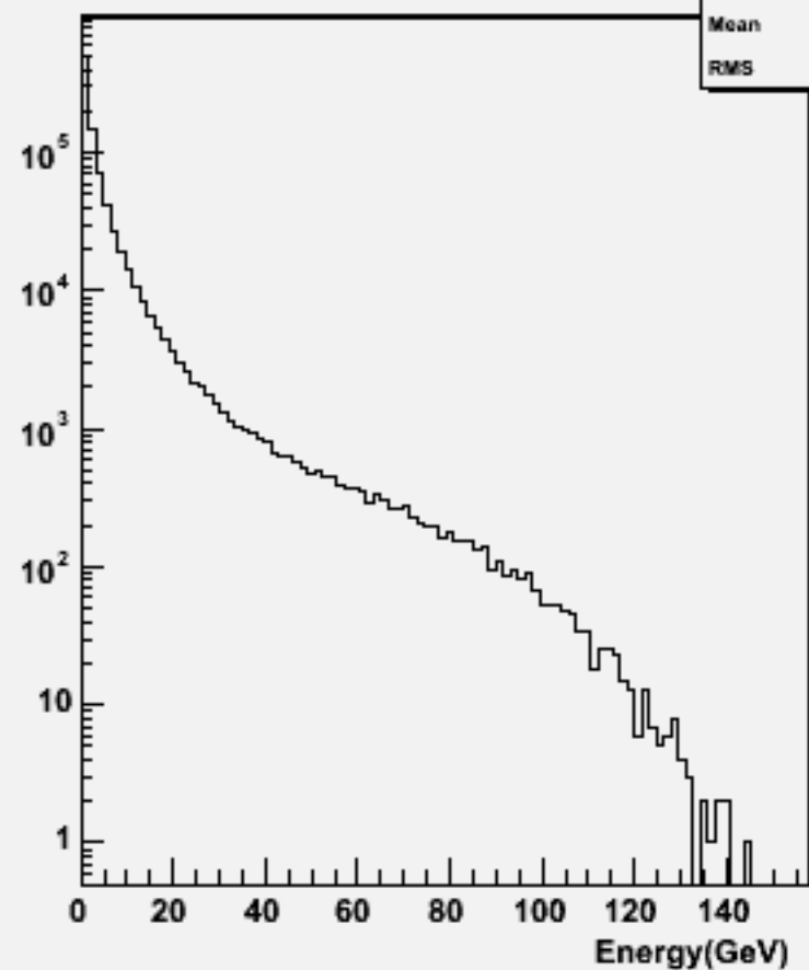
Particle Energy : w101085 ddcse3n3_o
