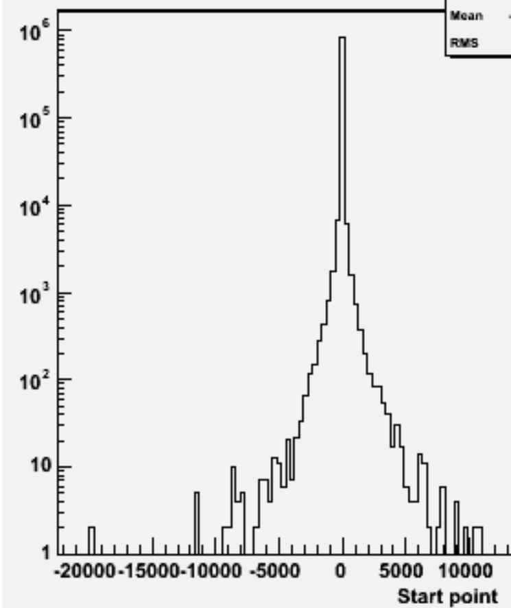
Start point Z : w101085 ddcse3n3_o
