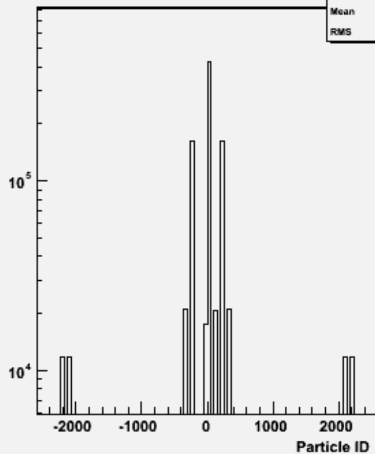
Particle ID : w101085 ddcse3n3_o
