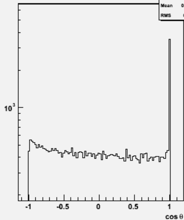
Jet cos \theta (All jets)w101085 ddcse3n3_o
