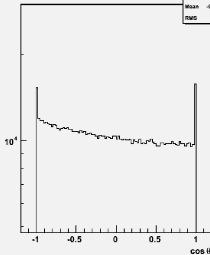
Particle cos \theta : w101085 ddcse3n3_o
