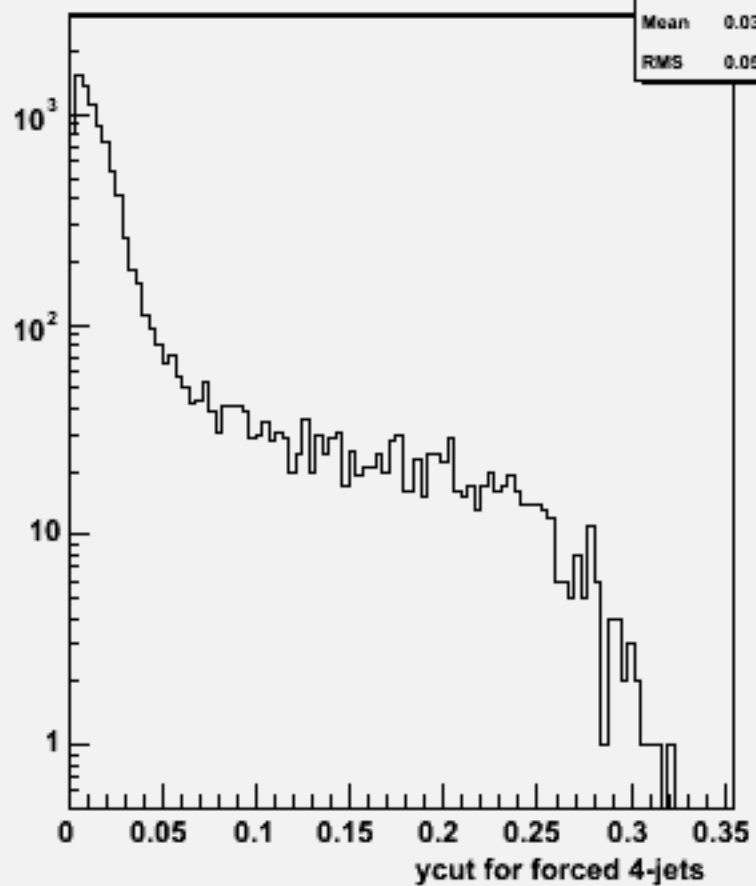
Ycut for 4-jets :w101085 ddcse3n3_o
