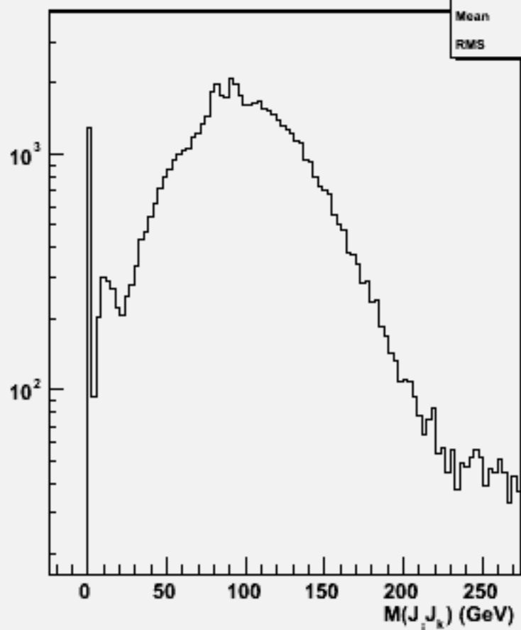
2jets mass(All comb)w101085 ddcse3n3_o
