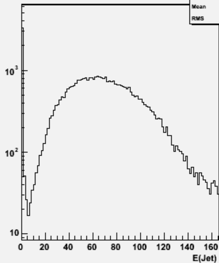
Jet energies(All jets)w101084 ddcse3n3_o
