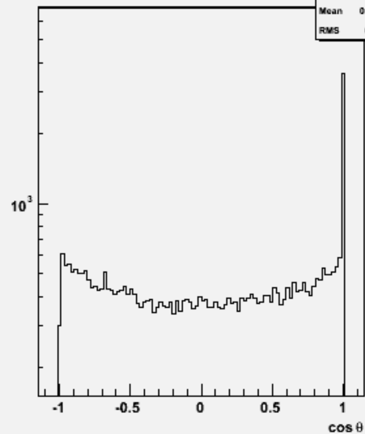
Jet cos \theta (All jets)w101084 ddcse3n3_o
