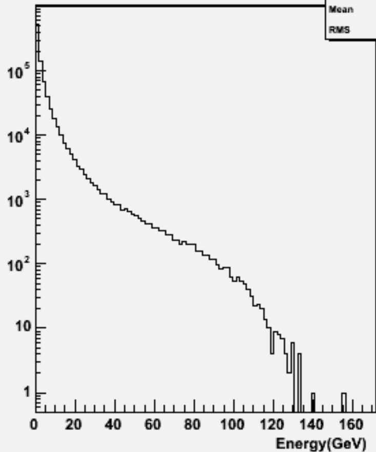
Particle Energy : w101084 ddcse3n3_o
