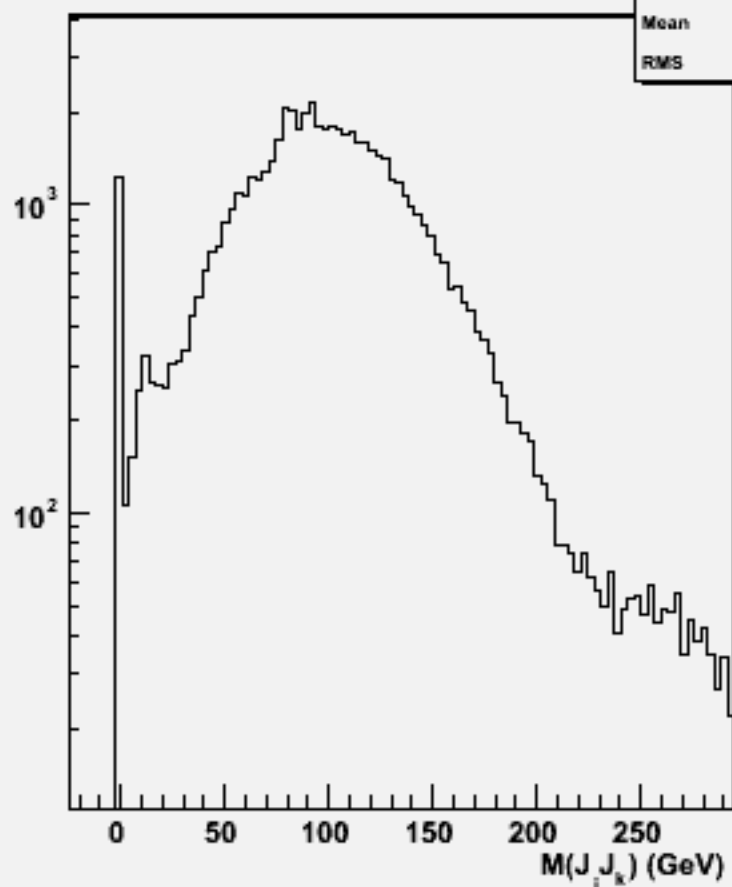
2jets mass(All comb)w101084 ddcse3n3_o
