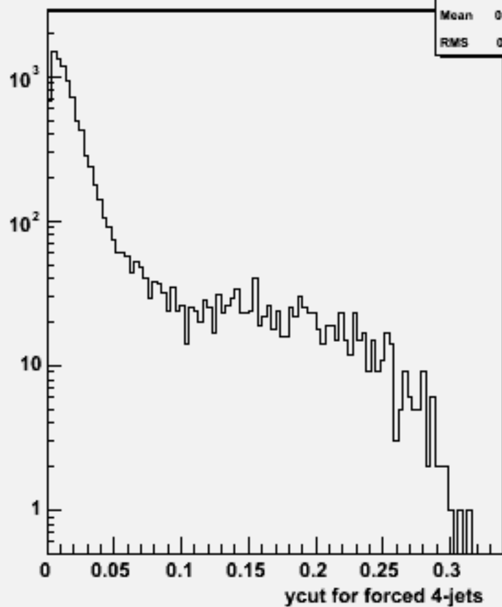
Ycut for 4-jets :w101084 ddcse3n3_o
