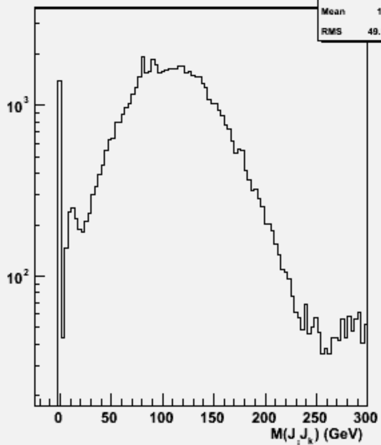
2jets mass(All comb)w101081 ddcse2n2_o
