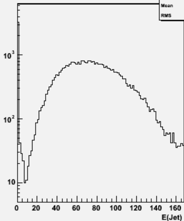
Jet energies(All jets)w101081 ddcse2n2_o
