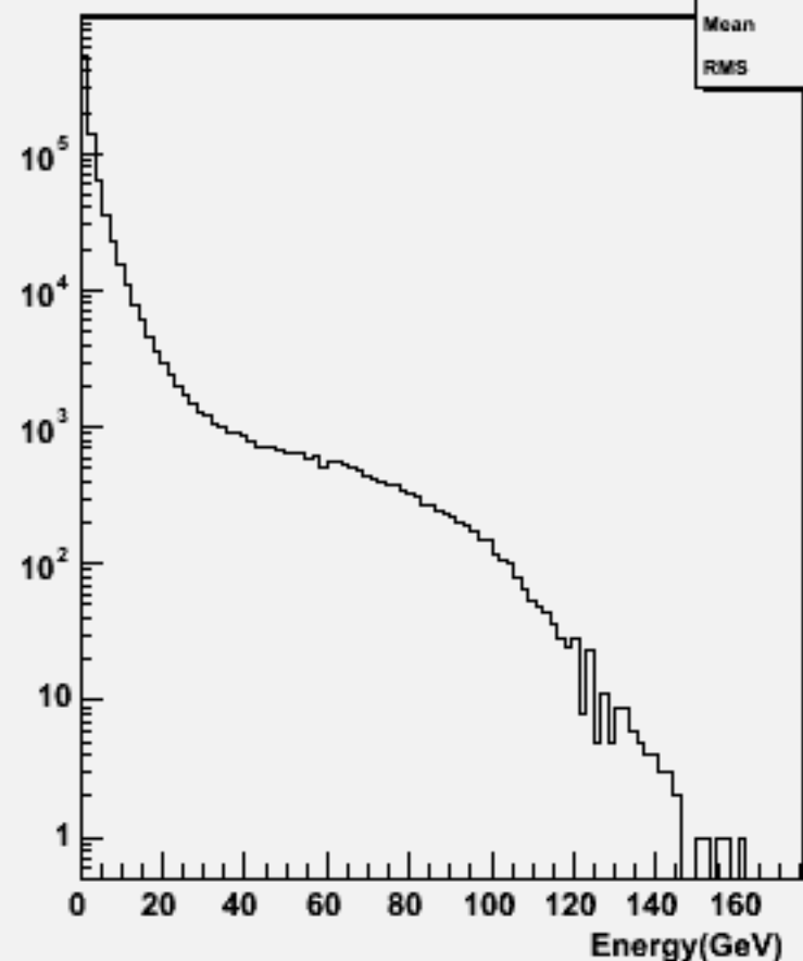
Particle Energy : w101081 ddcse2n2_o
