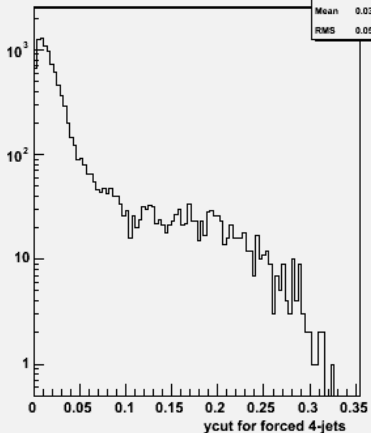
Ycut for 4-jets :w101081 ddcse2n2_o
