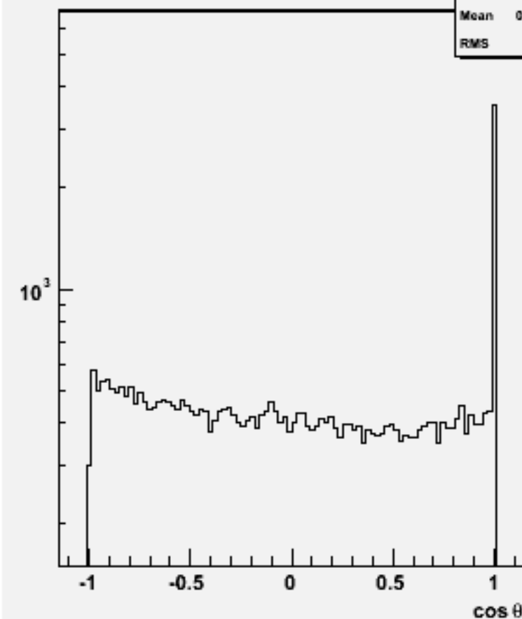
Jet cos \theta (All jets)w101081 ddcse2n2_o
