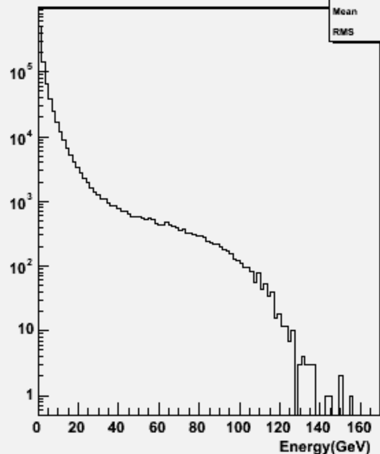
Particle Energy : w101076 ddcse1n1_o
