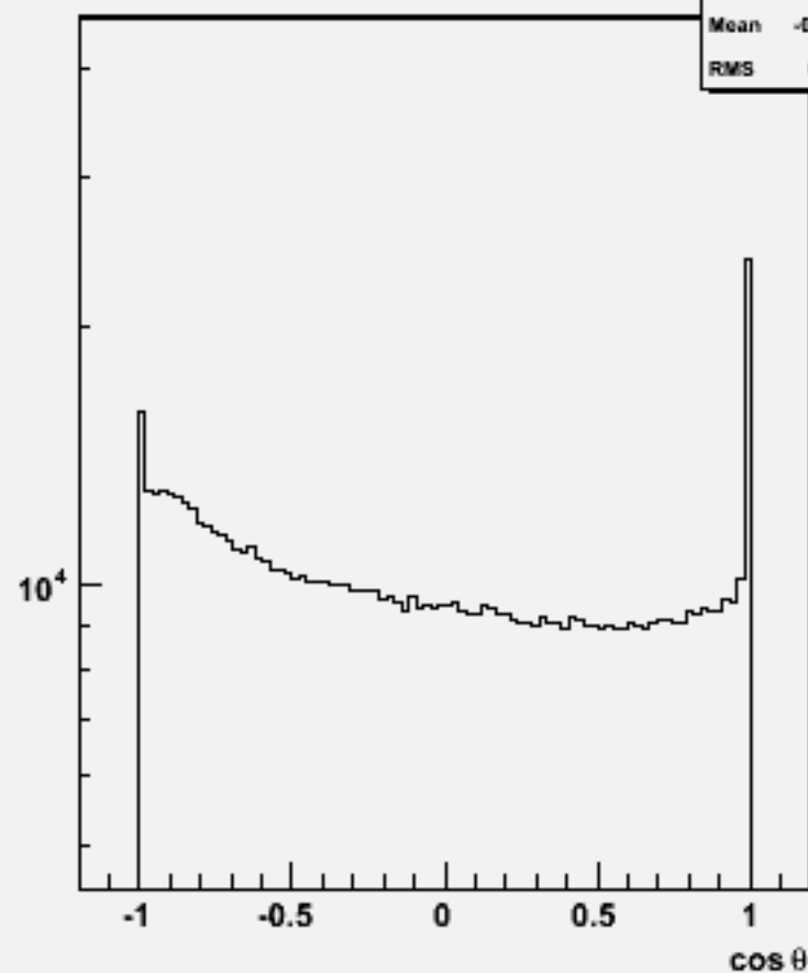
Particle cos \theta : w101076 ddcse1n1_o
