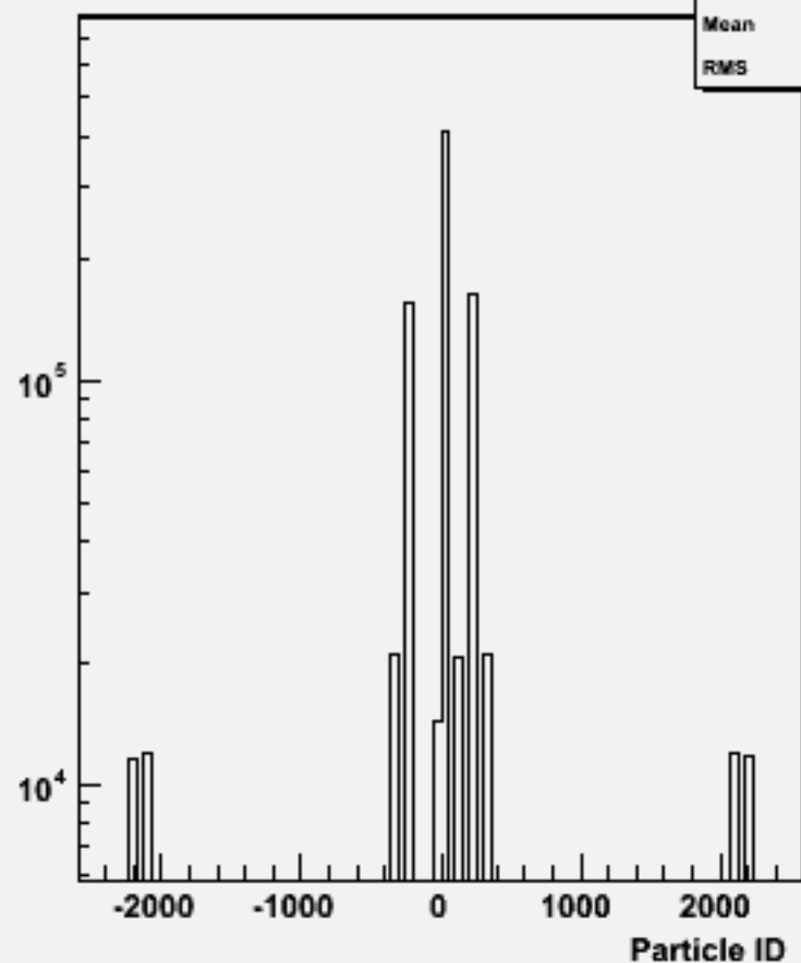
Particle ID : w101076 ddcse1n1_o
