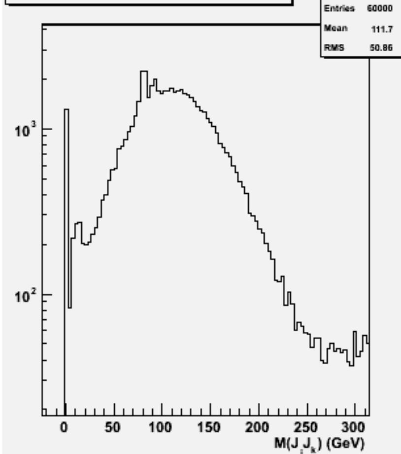
2jets mass(All comb)w101076 ddcse1n1_o
