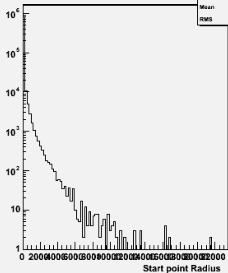
Start point R : w101076 ddcse1n1_o
