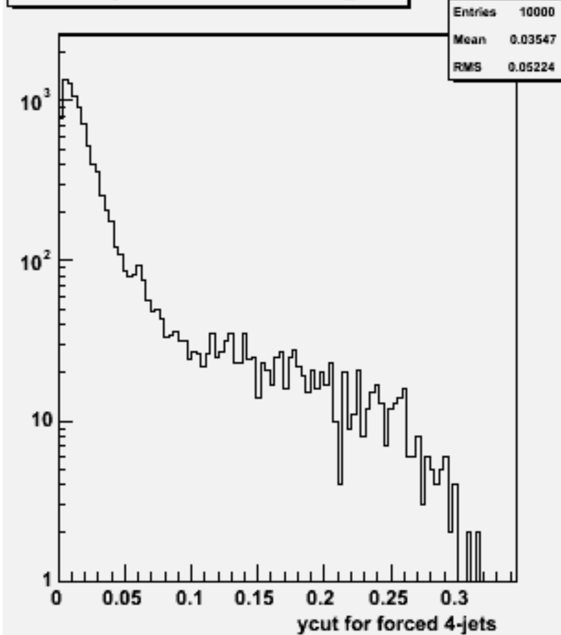
Ycut for 4-jets :w101076 ddcse1n1_o
