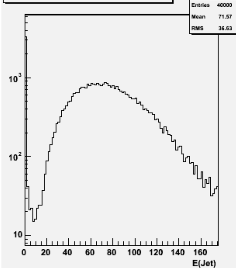
Jet energies(All jets)w101076 ddcse1n1_o
