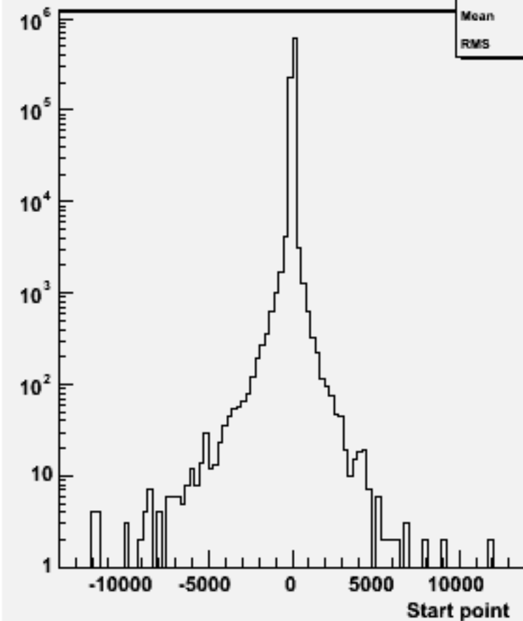
Start point Z : w101076 ddcse1n1_o
