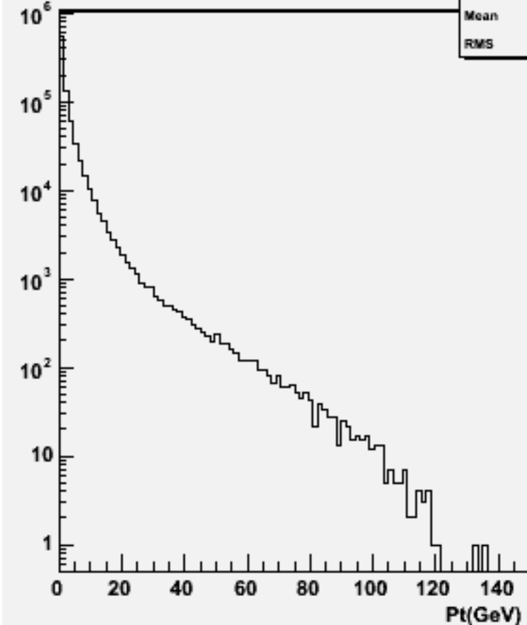
Particle Pt : w101076 ddcse1n1_o
