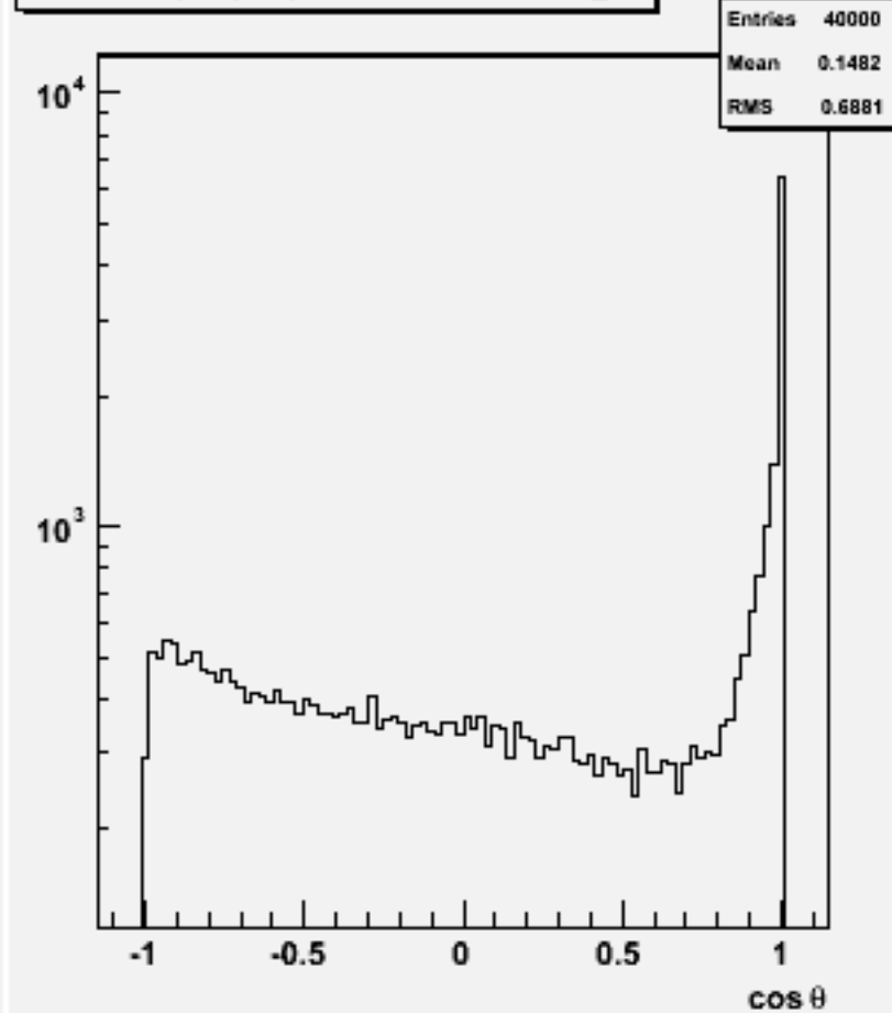
Jet cos \theta (All jets)w101076 ddcse1n1_o
