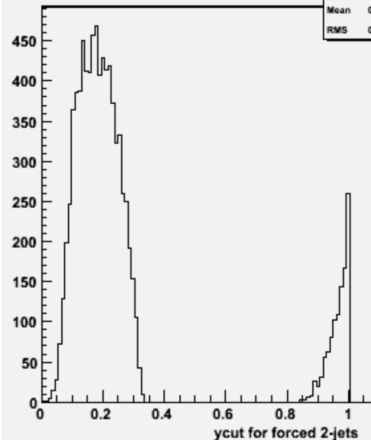
Ycut for 2-jets :w101072 ddudsc_o
