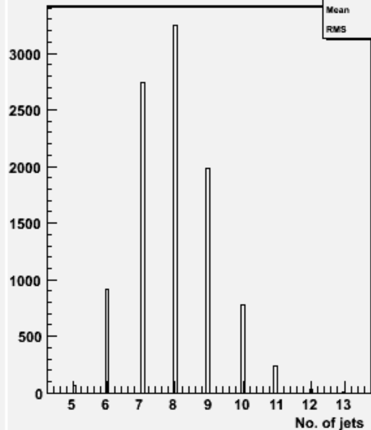
No. jets (ycut=0.001) : w101072 ddudsc_o
