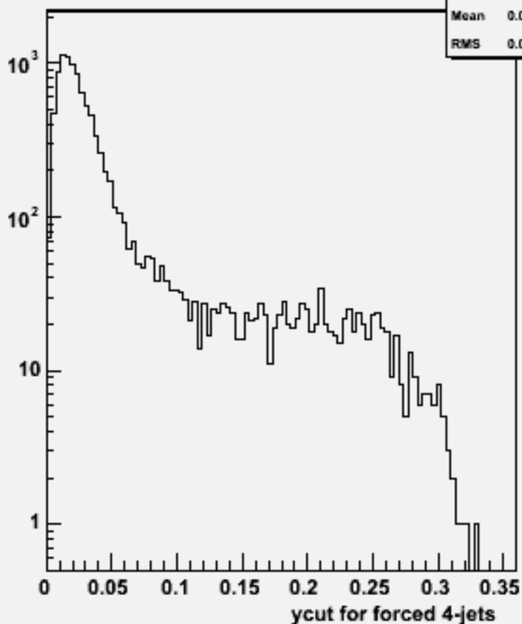
Ycut for 4-jets :w101072 ddudsc_o
