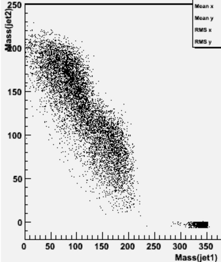
Jet mass for forced 2-jets : w101072 ddudsc_o
