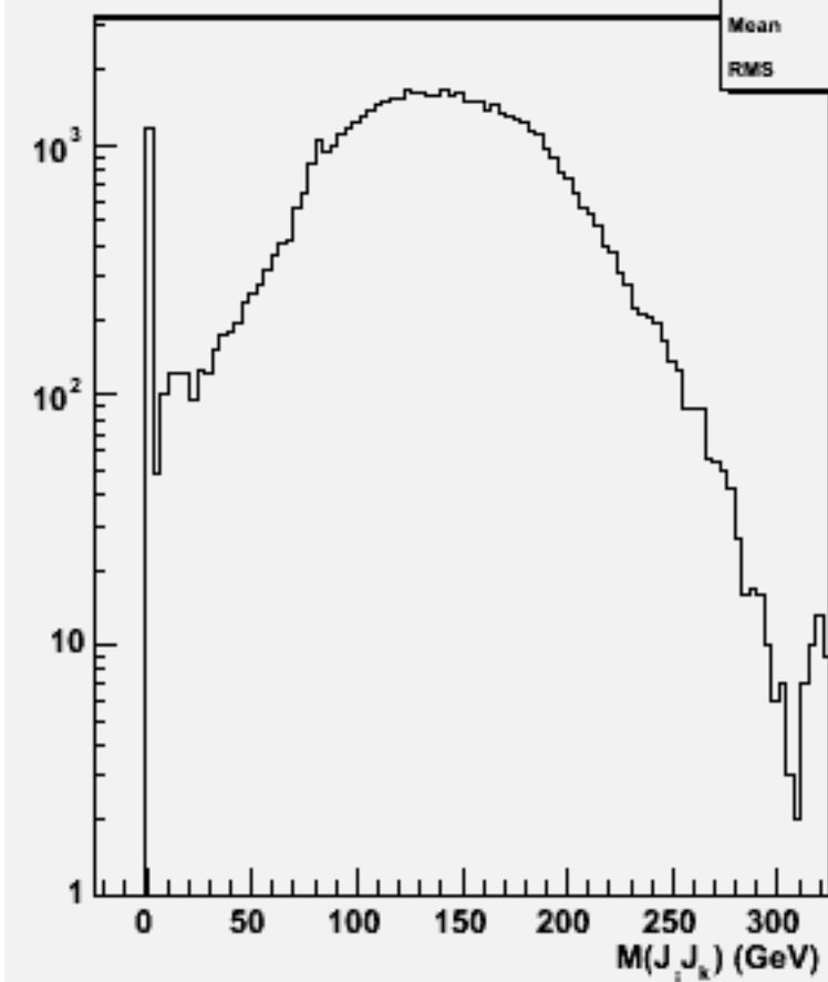
2jets mass(All comb)w101072 ddudsc_o
