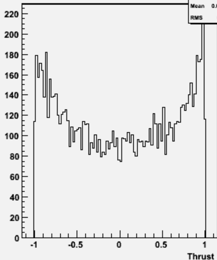
cos \Theta (thrust) w101072 ddudsc_o
