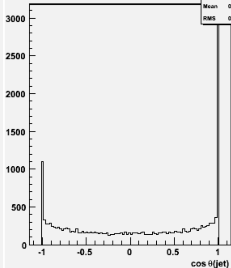
cos \theta for 2-jets :w101072 ddudsc_o
