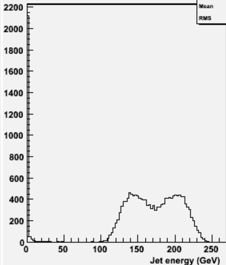
energy for 2-jets :w101072 ddudsc_o
