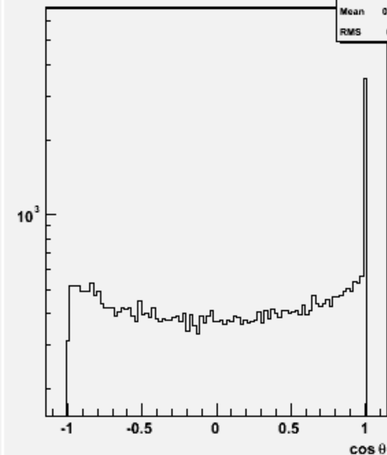
Jet cos \theta (All jets)w101072 ddudsc_o
