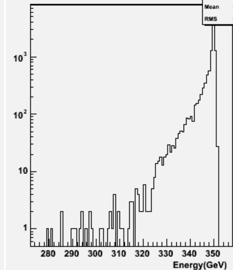
Total Energy (w/o \nu ): w101069 dduddu_o
