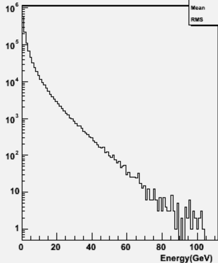
Particle Energy : w101069 dduddu_o
