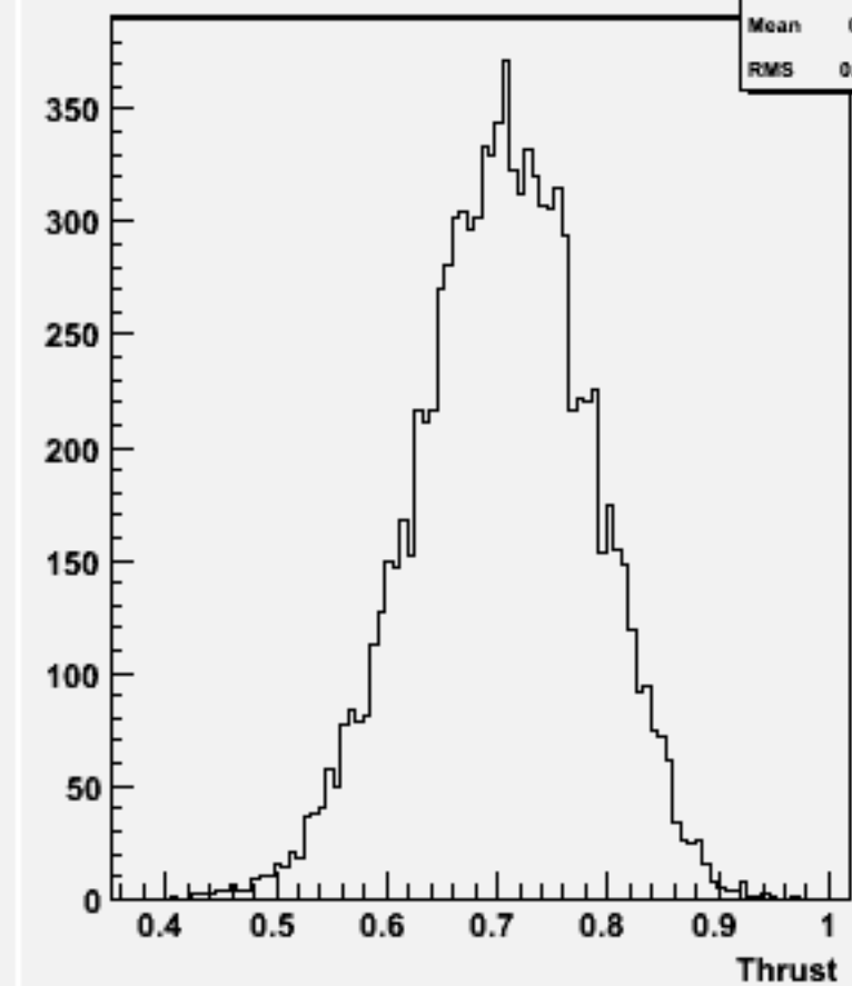
Thrust w101069 dduddu_o
