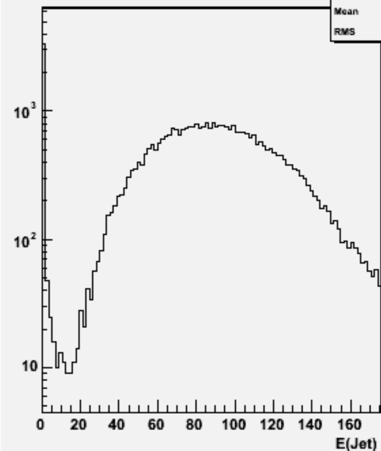
Jet energies(All jets)w101069 dduddu_o
