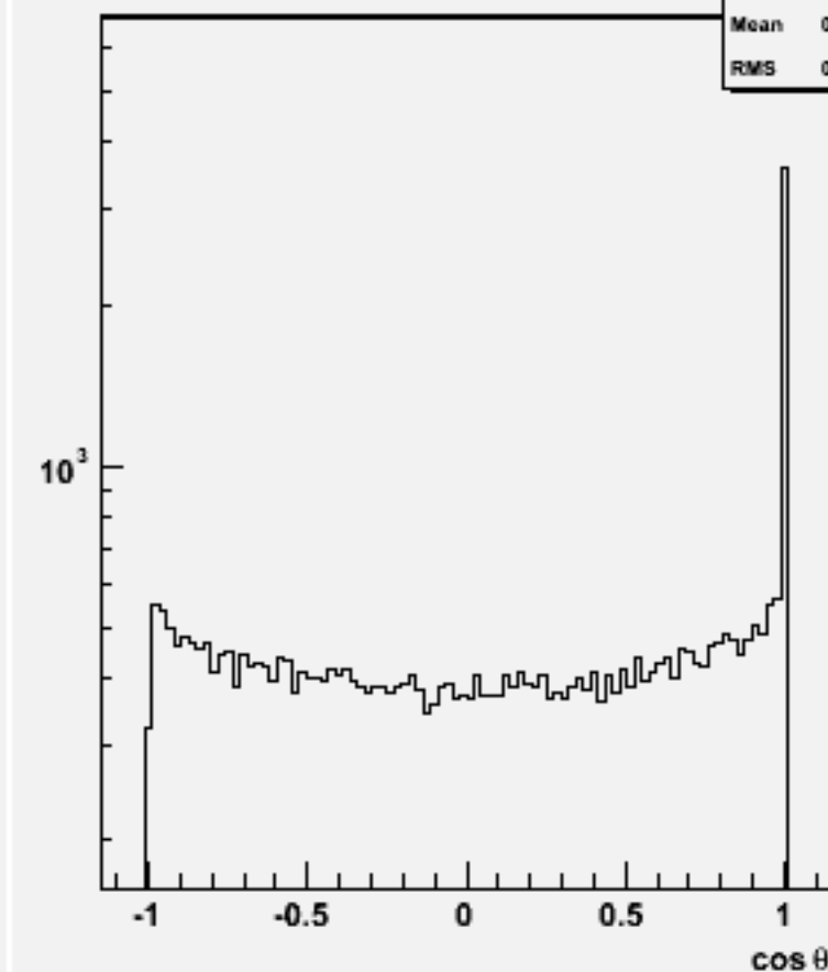
Jet cos \theta (All jets)w101069 dduddu_o
