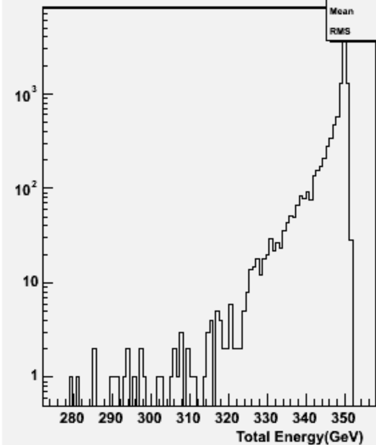
Total Energy (inc. \nu ): w101069 dduddu_o
