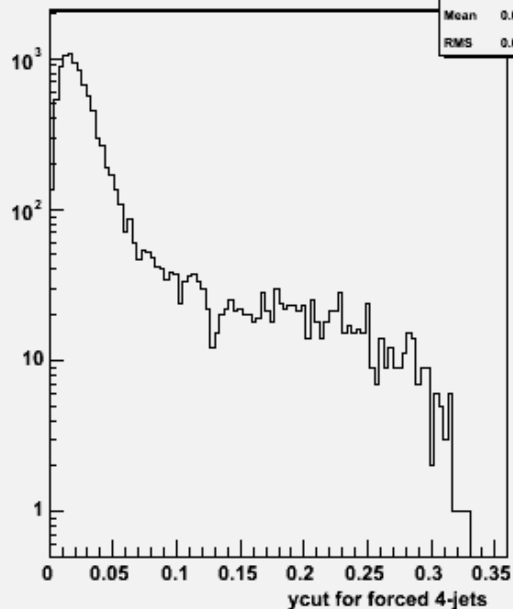
Ycut for 4-jets :w101069 dduddu_o
