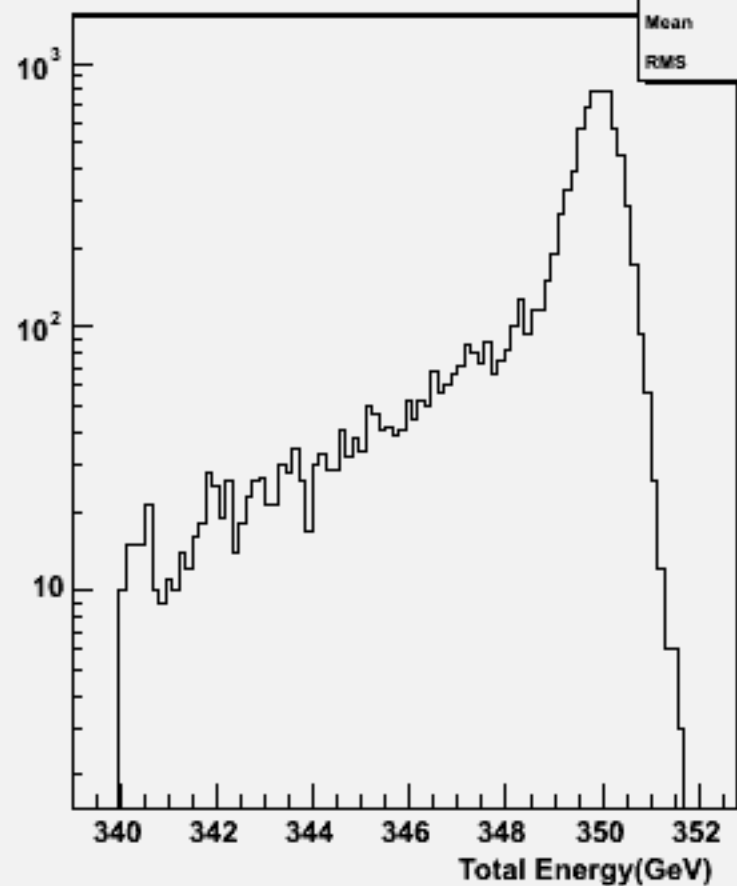
Total Energy (inc. \nu ): w101069 dduddu_o
