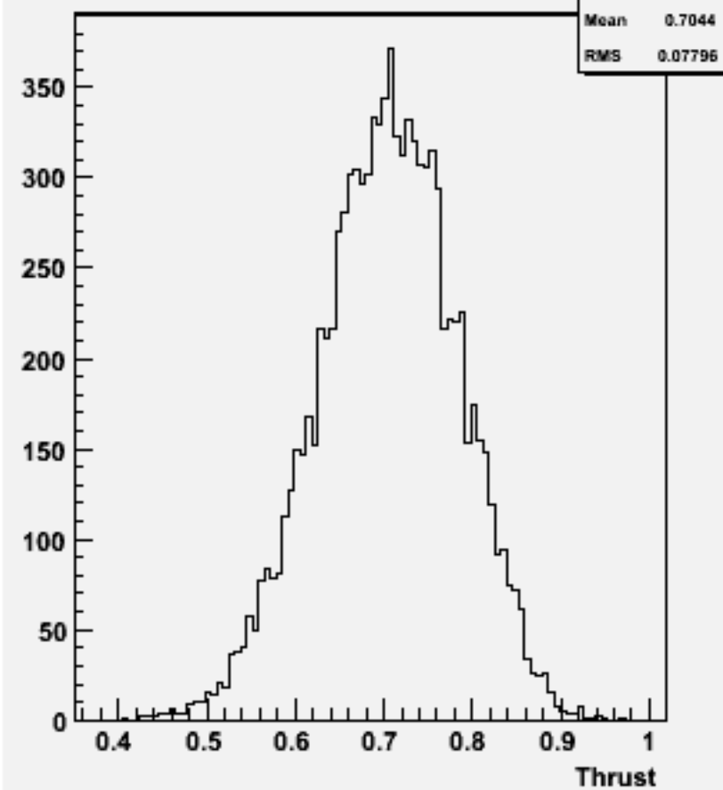
Thrust w101069 dduddu_o
