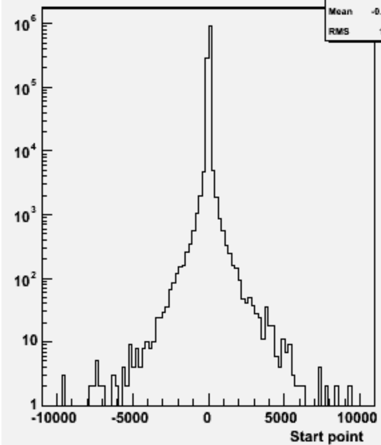
Start point Z : w101069 dduddu_o
