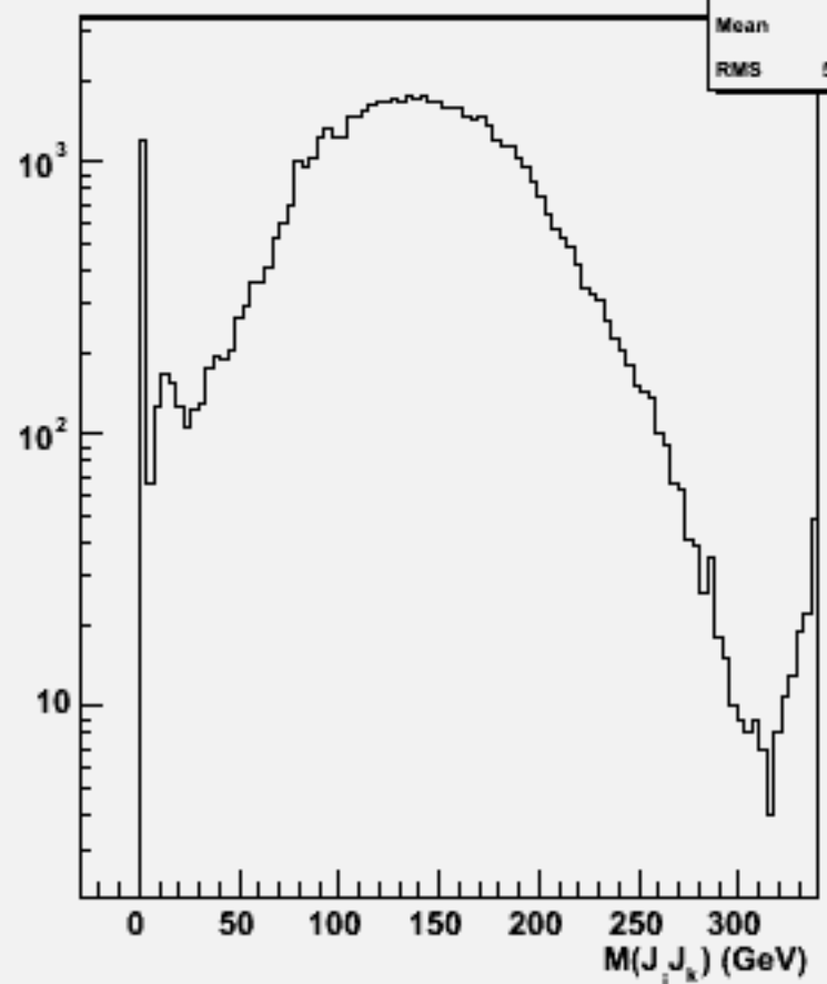
2jets mass(All comb)w101069 dduddu_o
