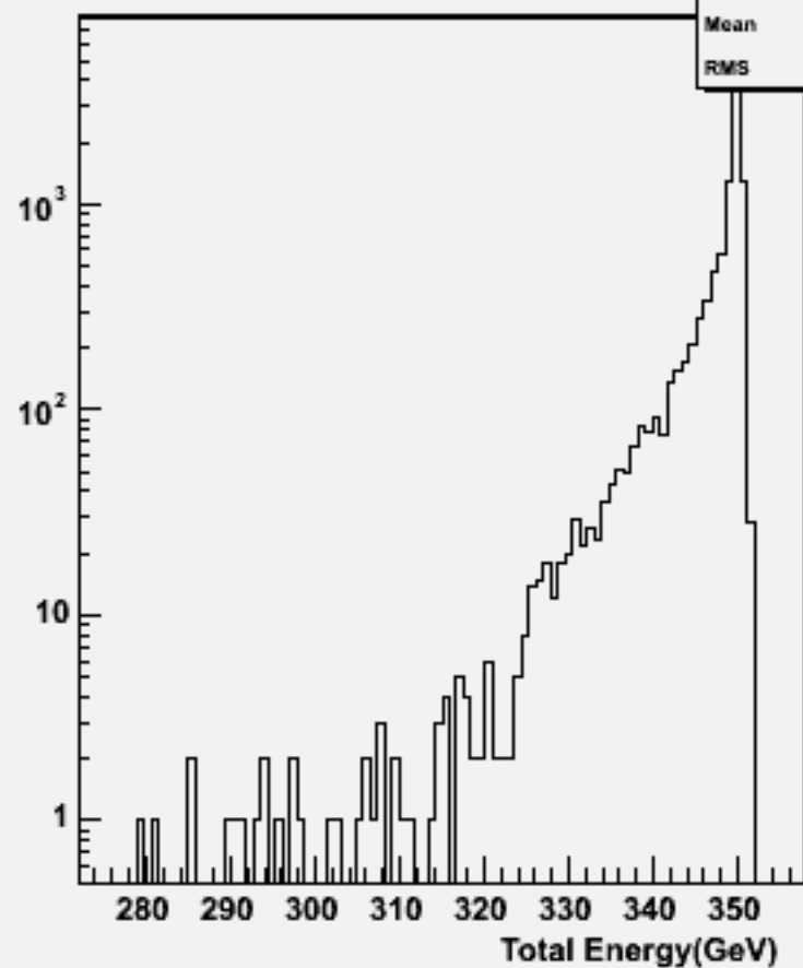
Total Energy (inc. \nu ): w101069 dduddu_o
