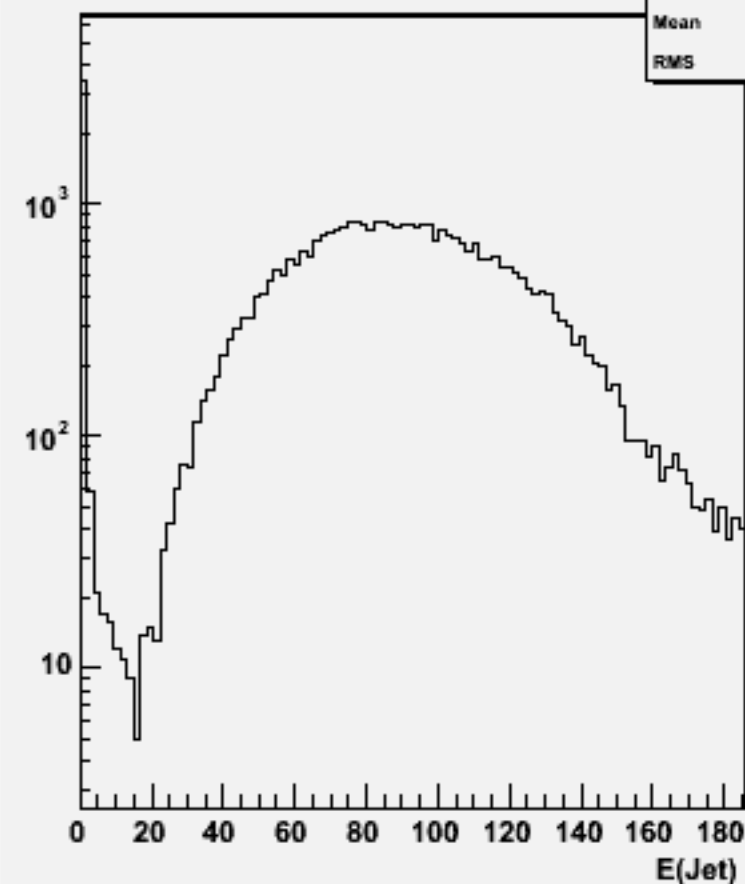
Jet energies(All jets)w101068 dduddu_o
