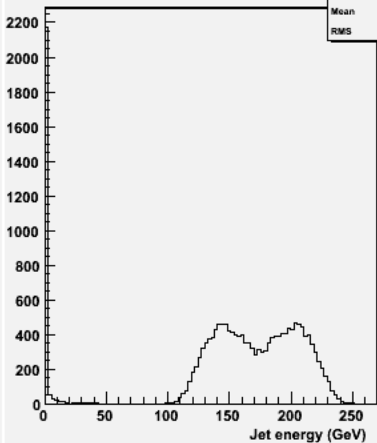
energy for 2-jets :w101068 dduddu_o
