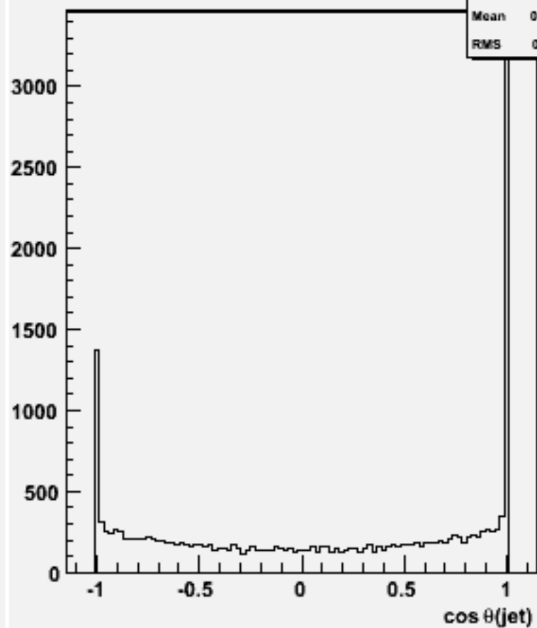
cos \theta for 2-jets :w101068 dduddu_o
