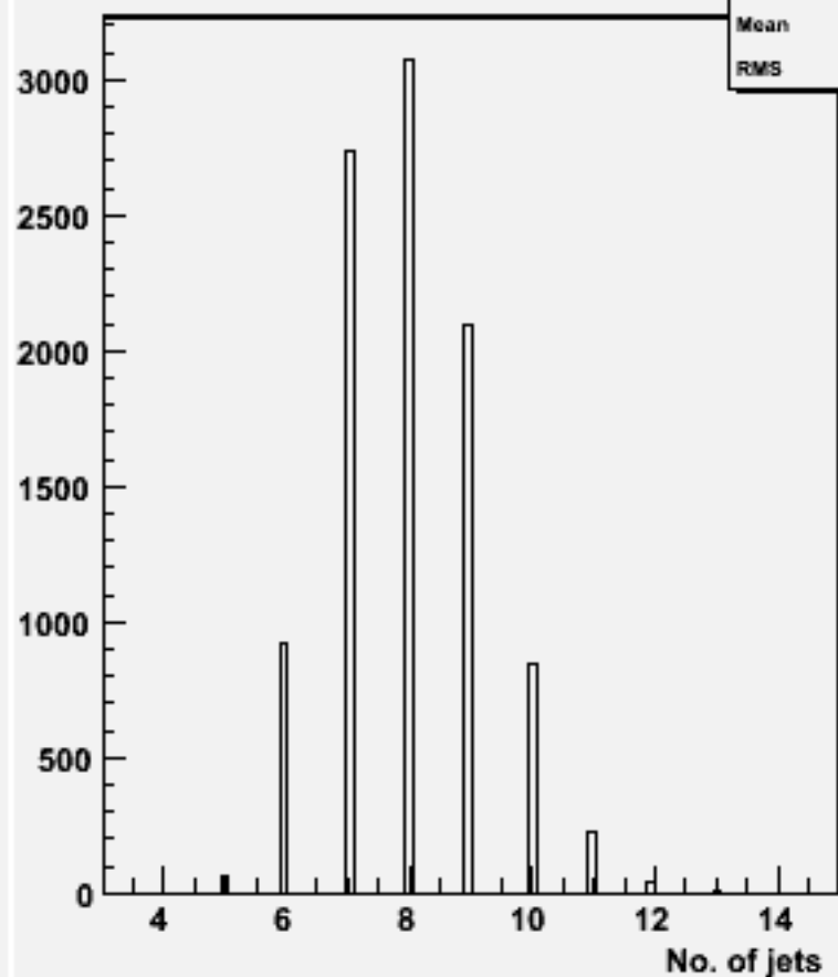
No. jets (ycut=0.001) : w101068 dduddu_o
