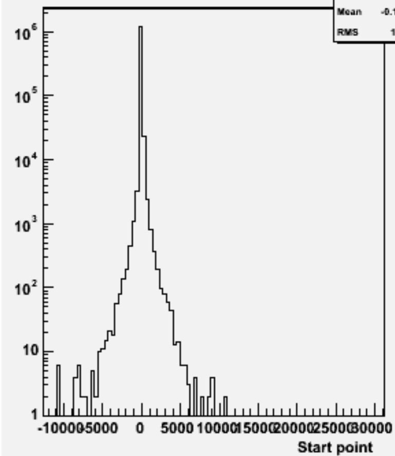
Start point Z : w101068 dduddu_o
