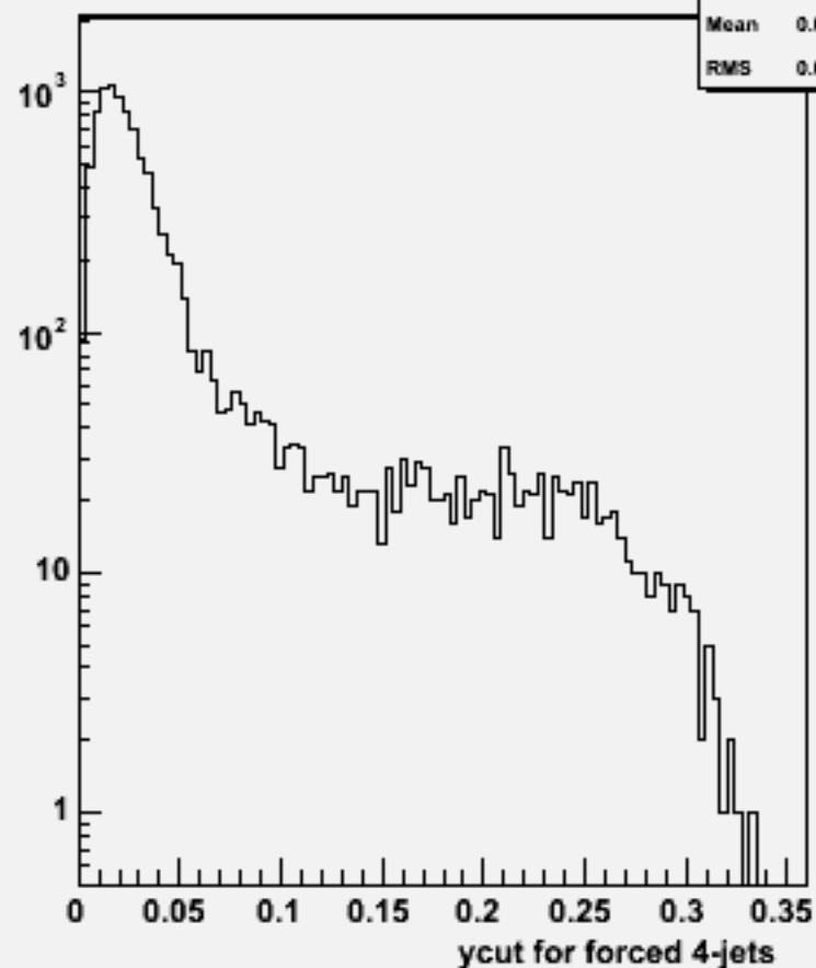
Ycut for 4-jets :w101068 dduddu_o
