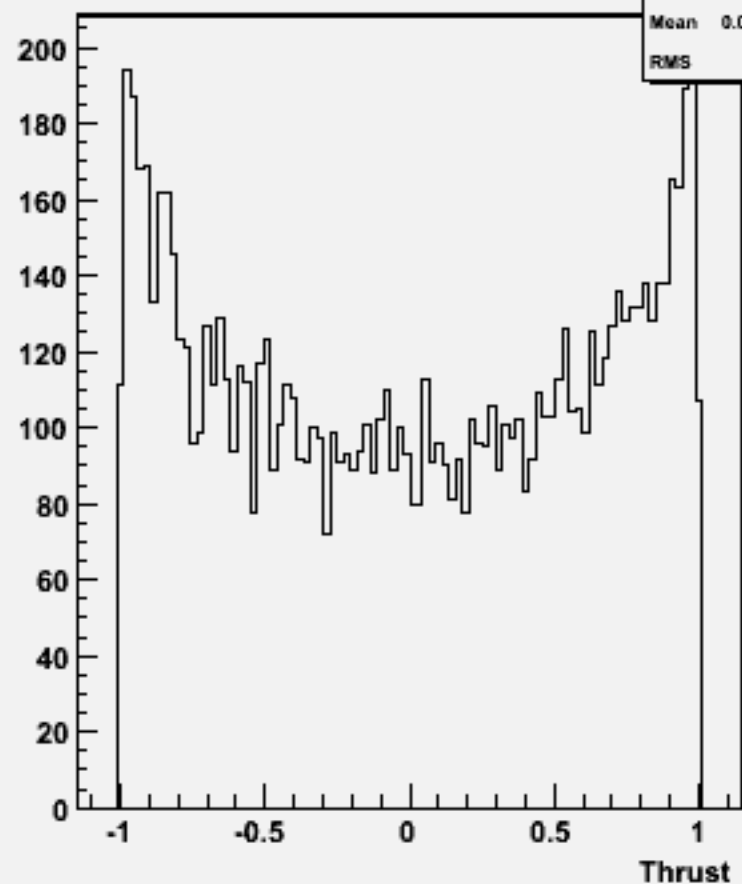
cos \Theta (thrust) w101068 dduddu_o
