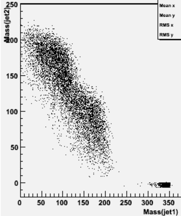
Jet mass for forced 2-jets : w101068 dduddu_o
