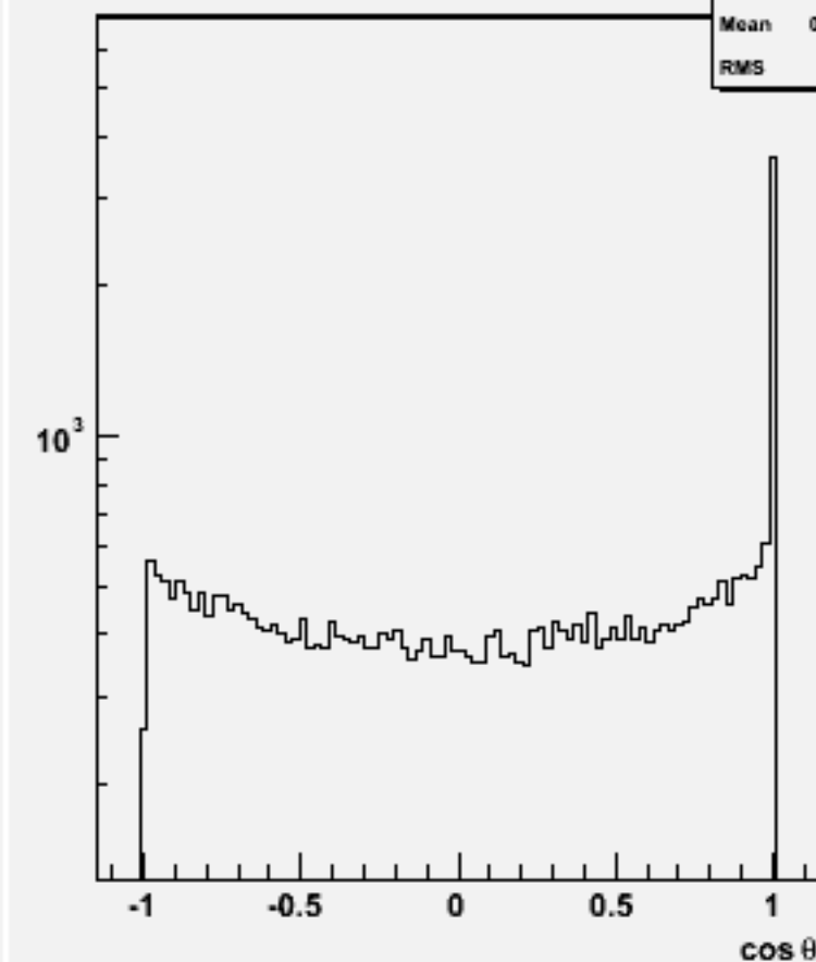
Jet cos \theta (All jets)w101068 dduddu_o
