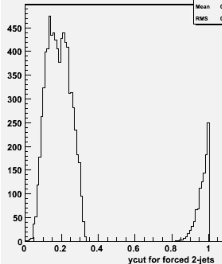
Ycut for 2-jets :w101068 dduddu_o
