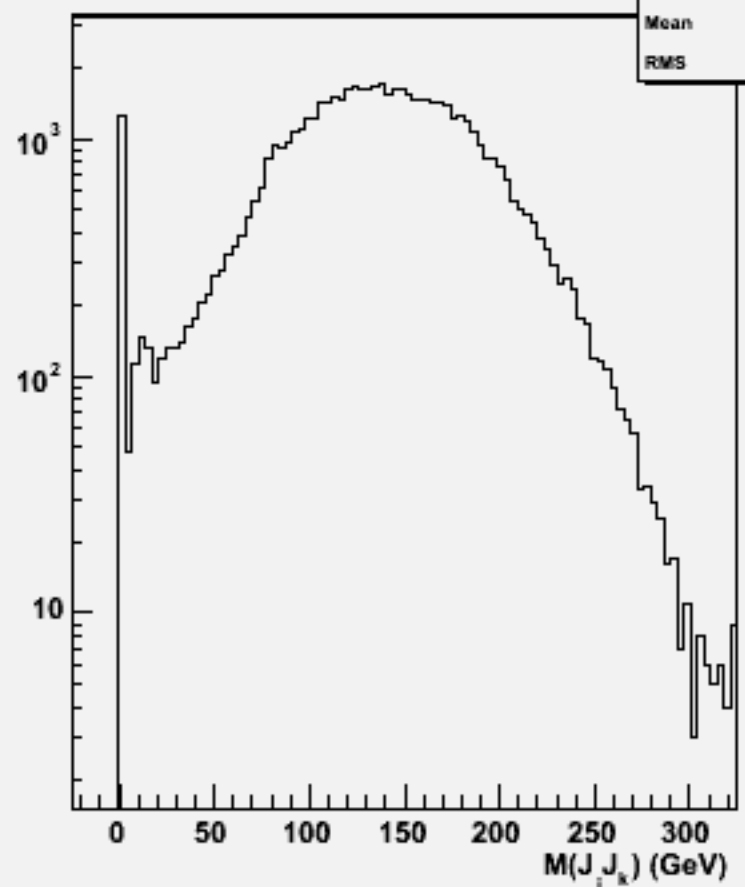
2jets mass(All comb)w101068 dduddu_o
