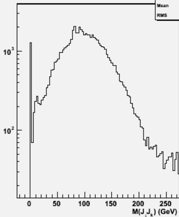
2jets mass(All comb)w101064 ddude3n3_o
