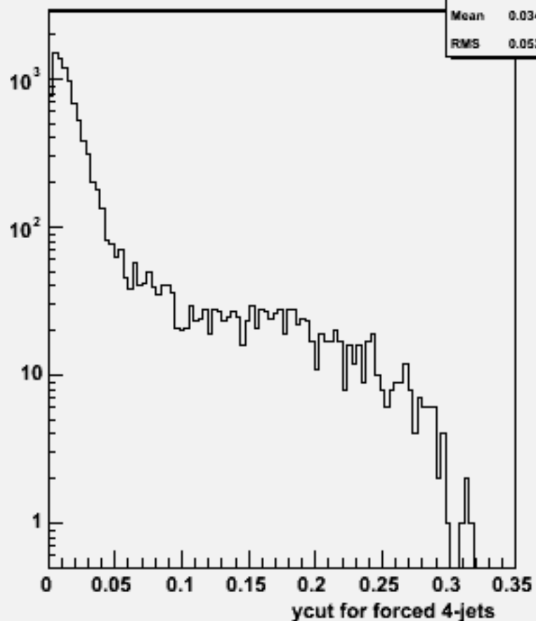
Ycut for 4-jets :w101064 ddude3n3_o
