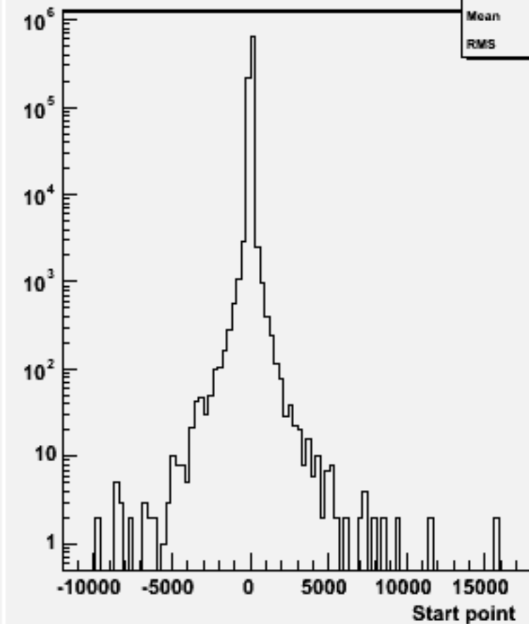
Start point Z : w101064 ddude3n3_o
