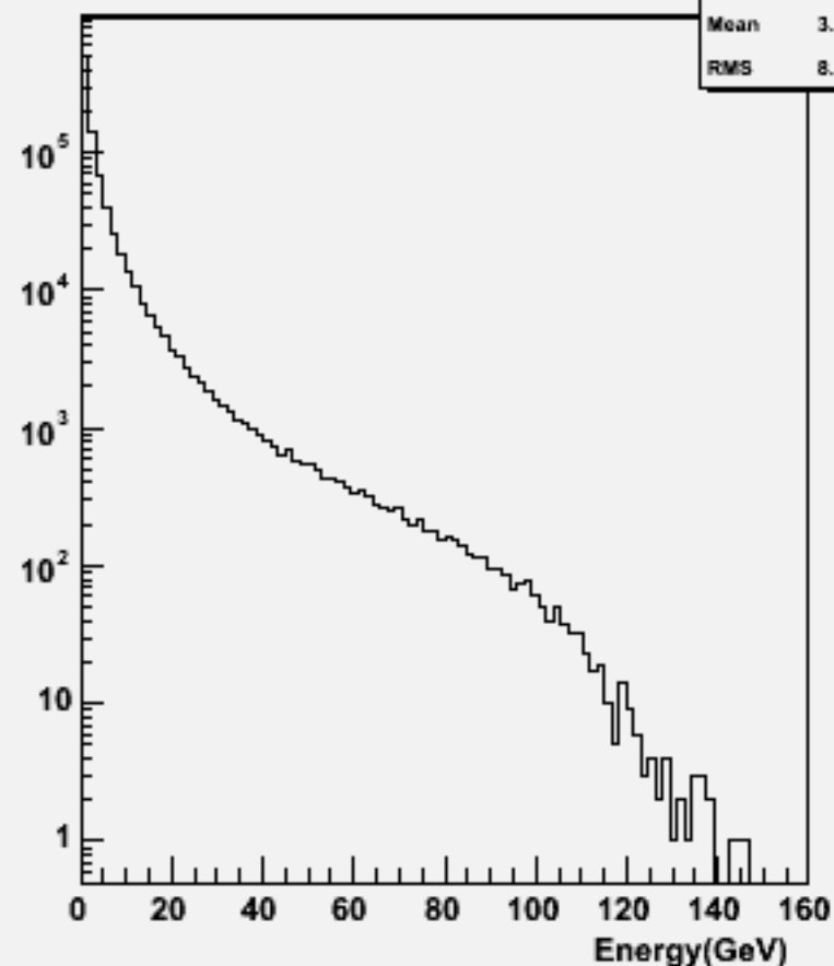
Particle Energy : w101064 ddude3n3_o
