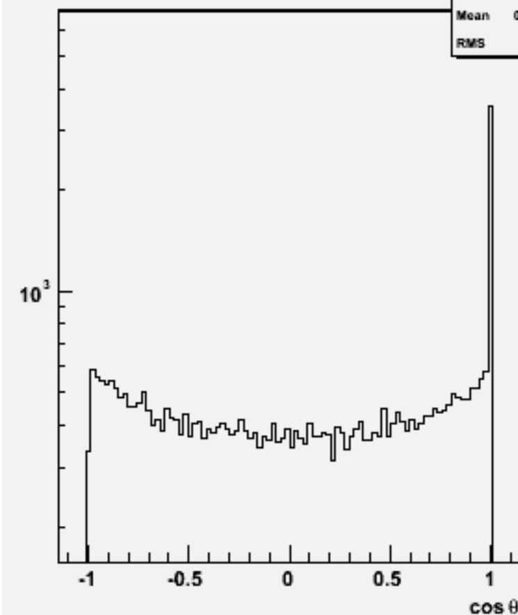
Jet cos \theta (All jets)w101064 ddude3n3_o
