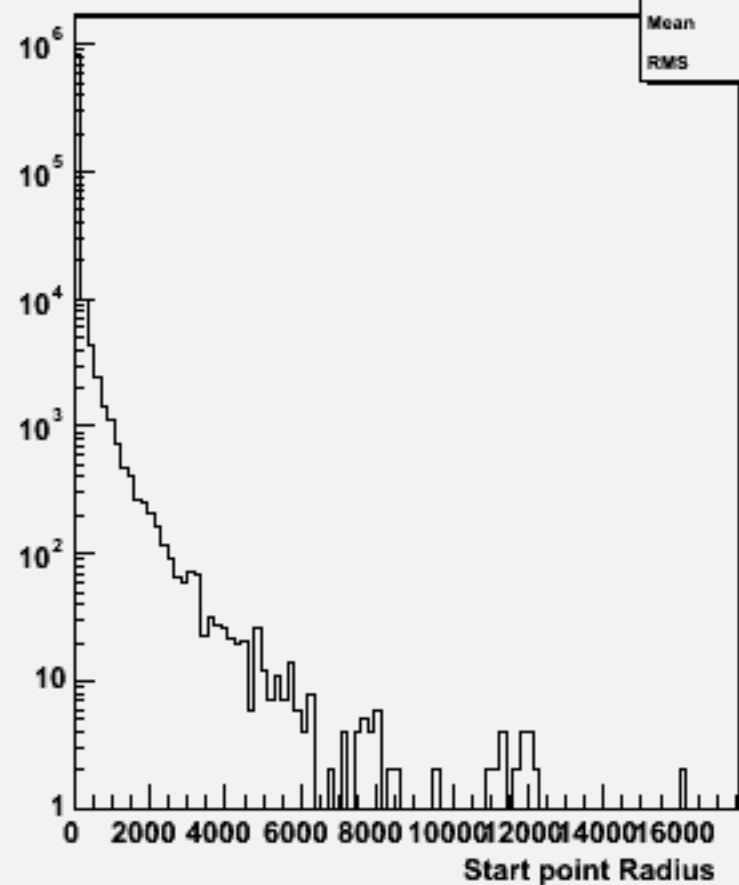
Start point R : w101064 ddude3n3_o
