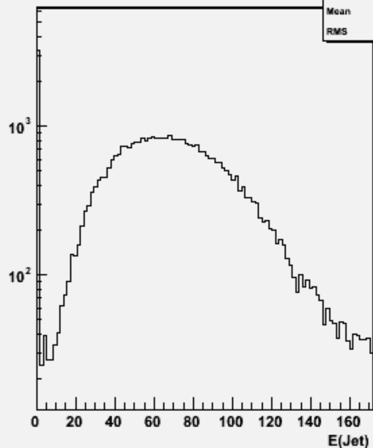
Jet energies(All jets)w101064 ddude3n3_o
