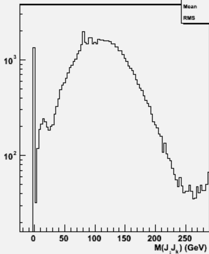
2jets mass(All comb)w101061 ddude2n2_o
