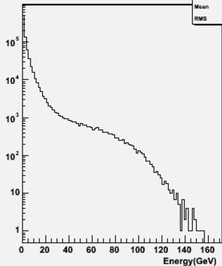
Particle Energy : w101061 ddude2n2_o
