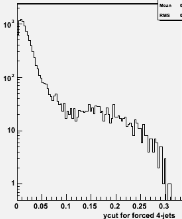
Ycut for 4-jets :w101061 ddude2n2_o
