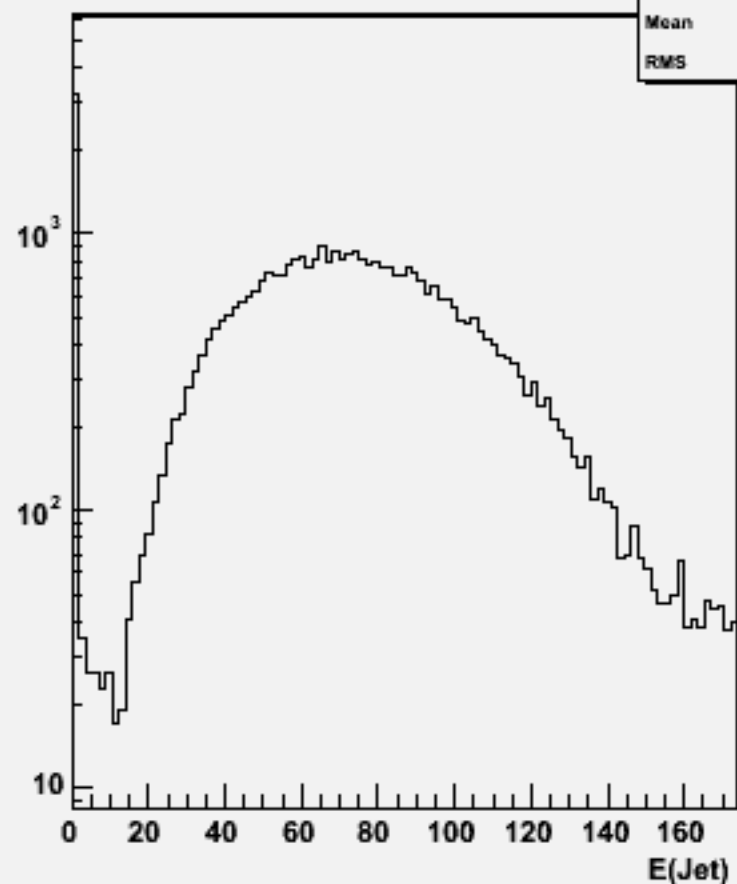
Jet energies(All jets)w101061 ddude2n2_o
