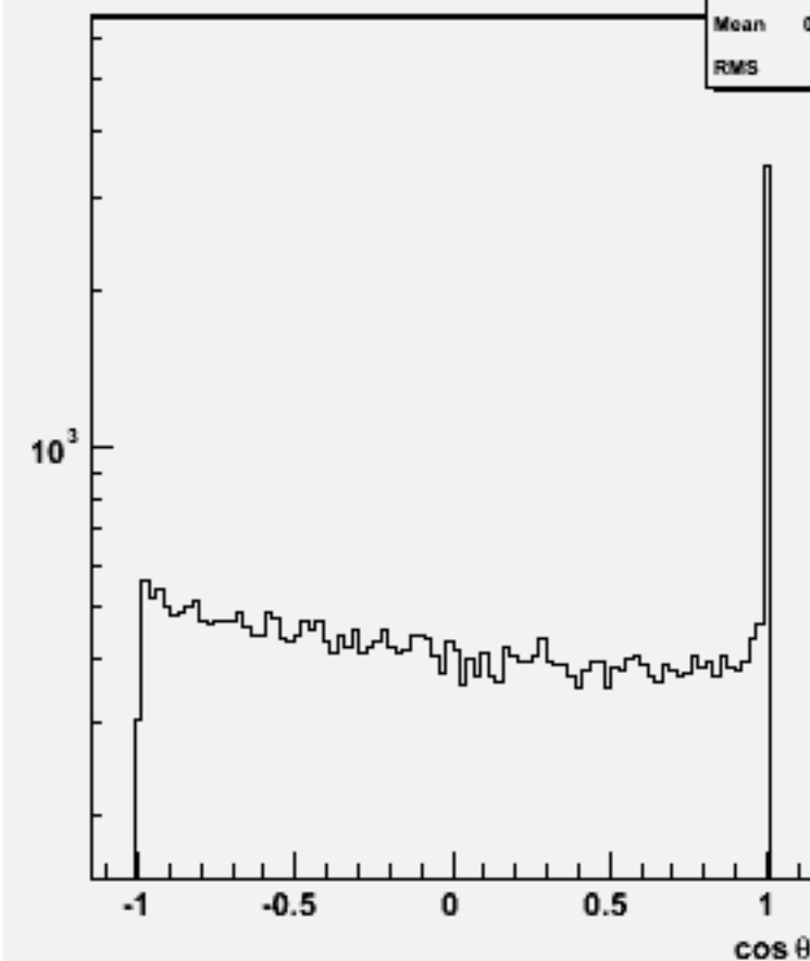
Jet cos \theta (All jets)w101061 ddude2n2_o
