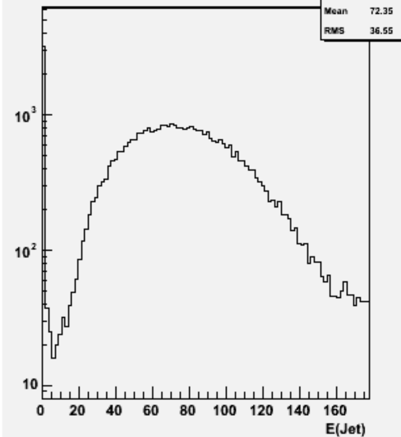
Jet energies(All jets)w101060 ddude2n2_o
