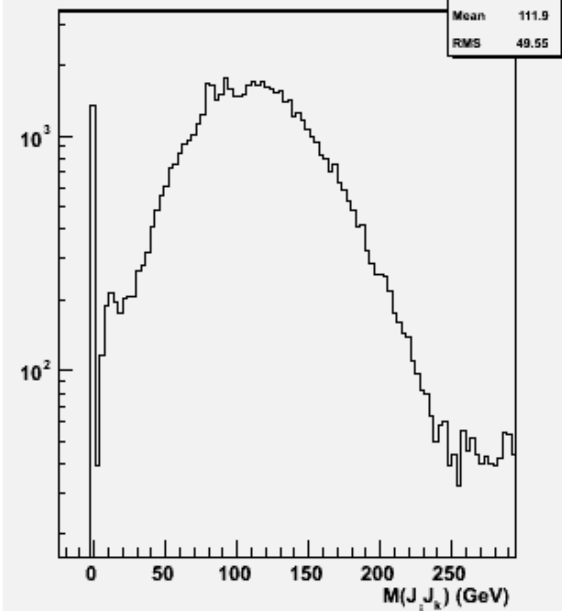
2jets mass(All comb)w101060 ddude2n2_o
