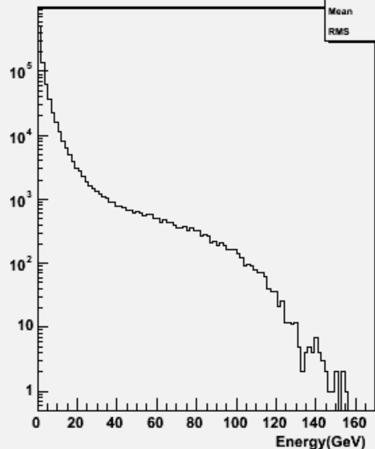
Particle Energy : w101060 ddude2n2_o
