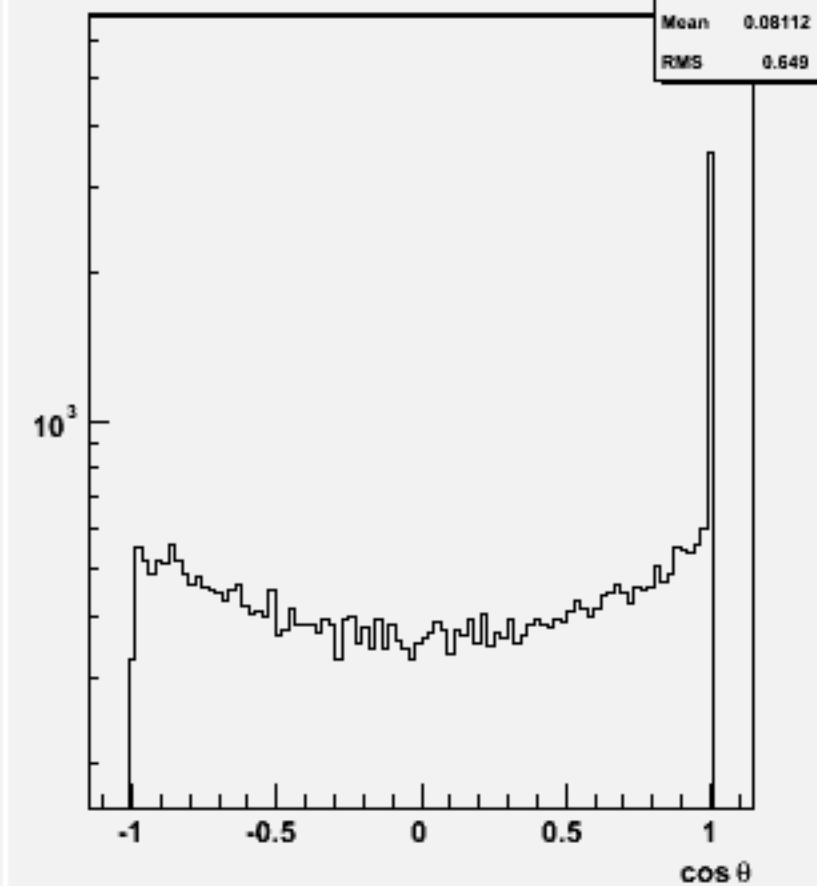
Jet cos \theta (All jets)w101060 ddude2n2_o
