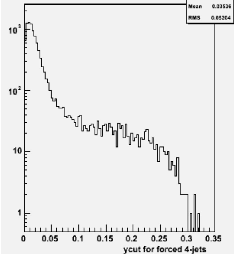
Ycut for 4-jets :w101060 ddude2n2_o
