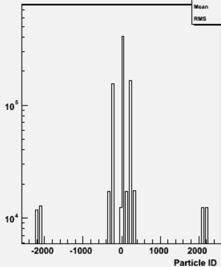
Particle ID : w101058 ddude1n1_o
