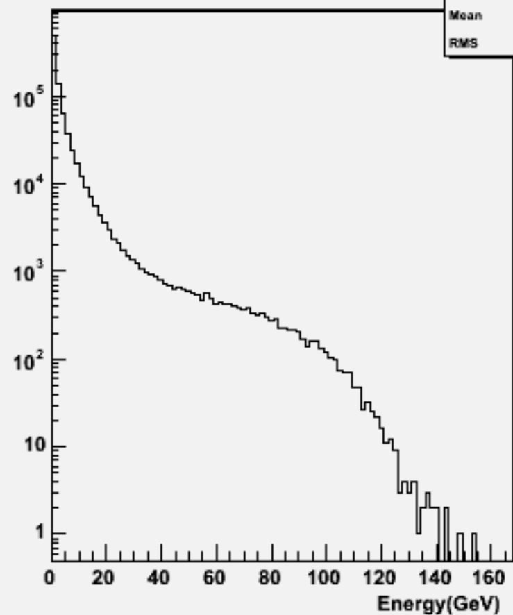
Particle Energy : w101058 ddude1n1_o
