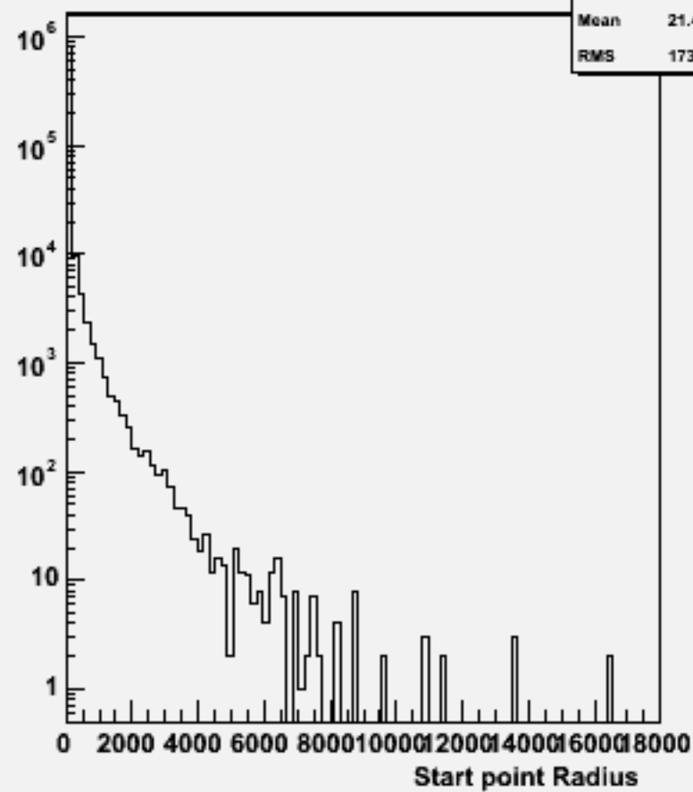
Start point R : w101058 ddude1n1_o
