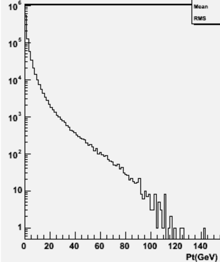
Particle Pt : w101058 ddude1n1_o
