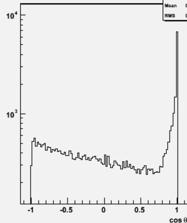
Jet cos \theta (All jets)w101058 ddude1n1_o
