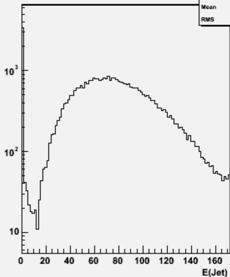
Jet energies(All jets)w101058 ddude1n1_o
