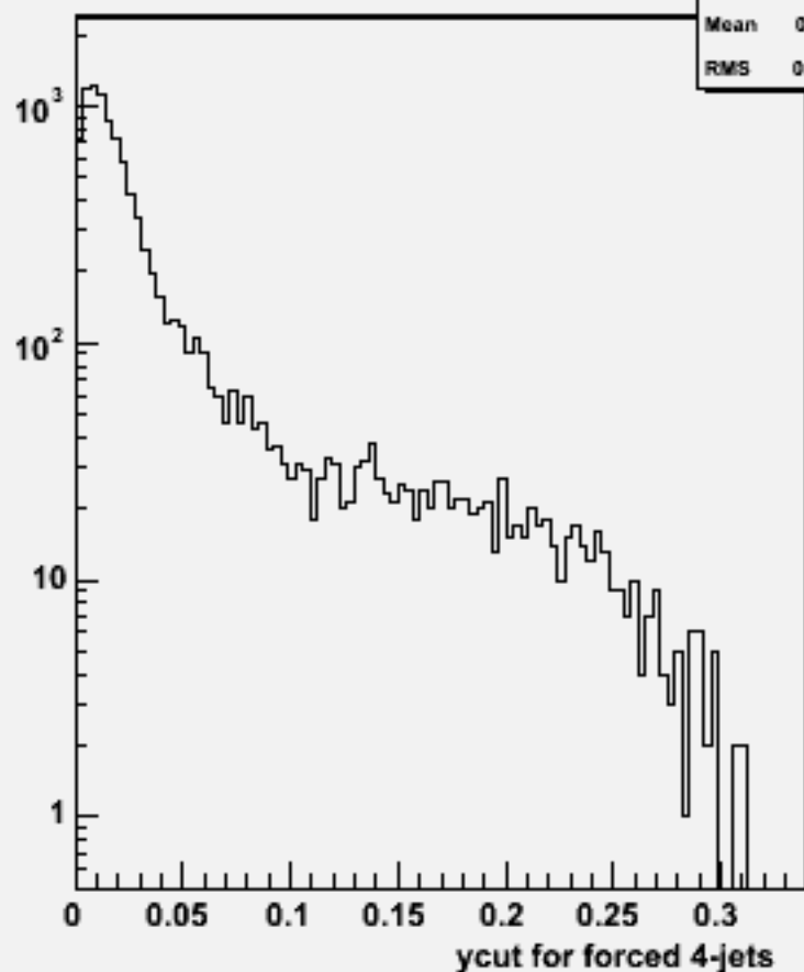
Ycut for 4-jets :w101058 ddude1n1_o
