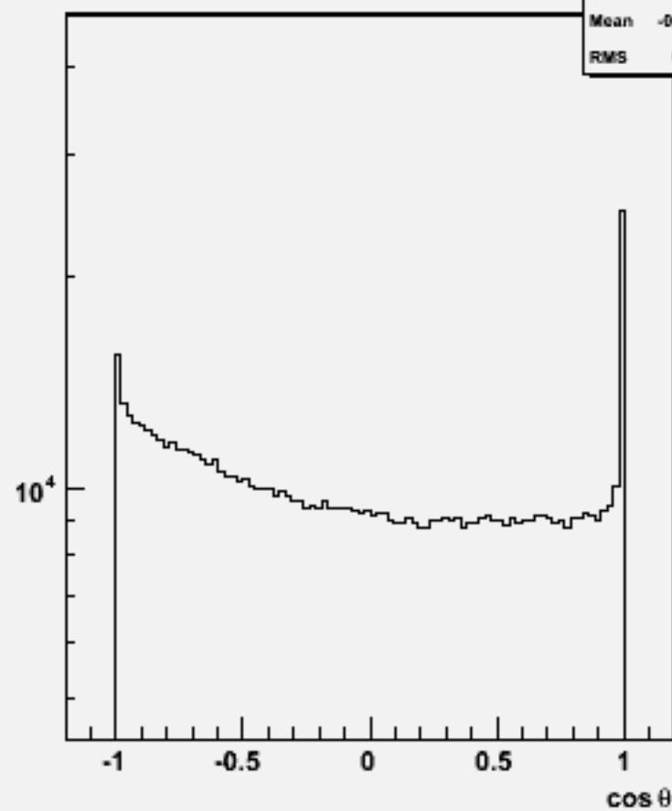
Particle cos \theta : w101058 ddude1n1_o
