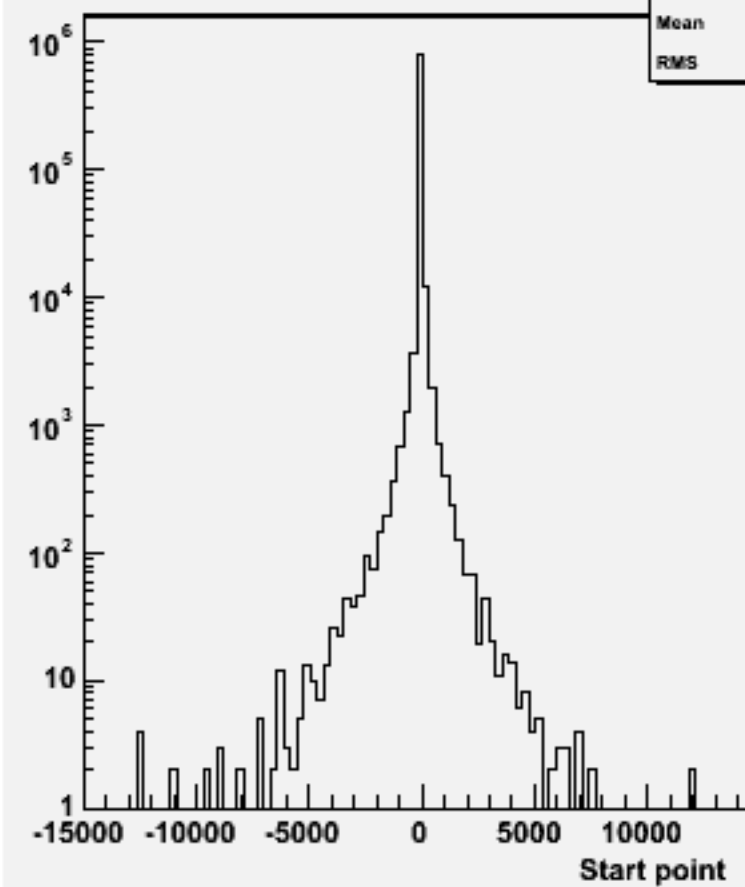
Start point Z : w101058 ddude1n1_o
