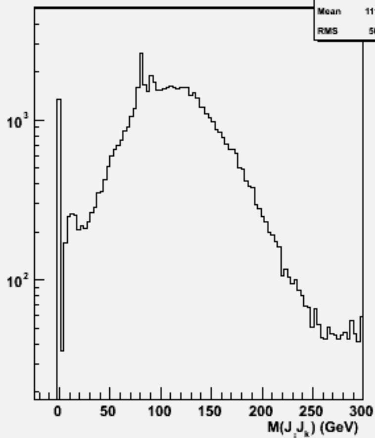
2jets mass(All comb)w101058 ddude1n1_o
