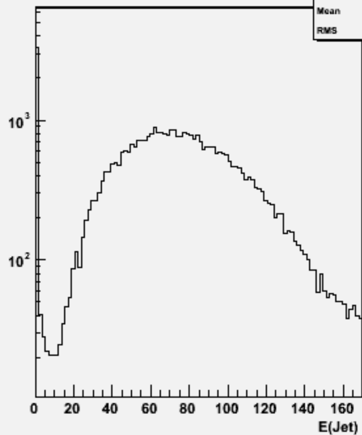
Jet energies(All jets)w101057 ddude1n1_o
