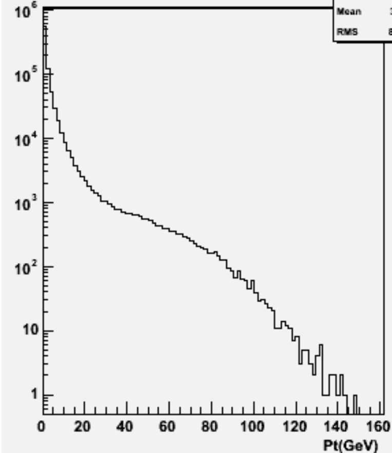
Particle Pt : w101057 ddude1n1_o
