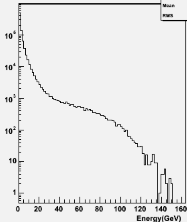
Particle Energy : w101057 ddude1n1_o
