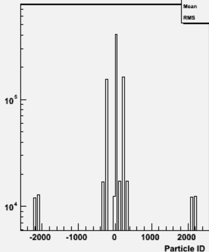
Particle ID : w101057 ddude1n1_o
