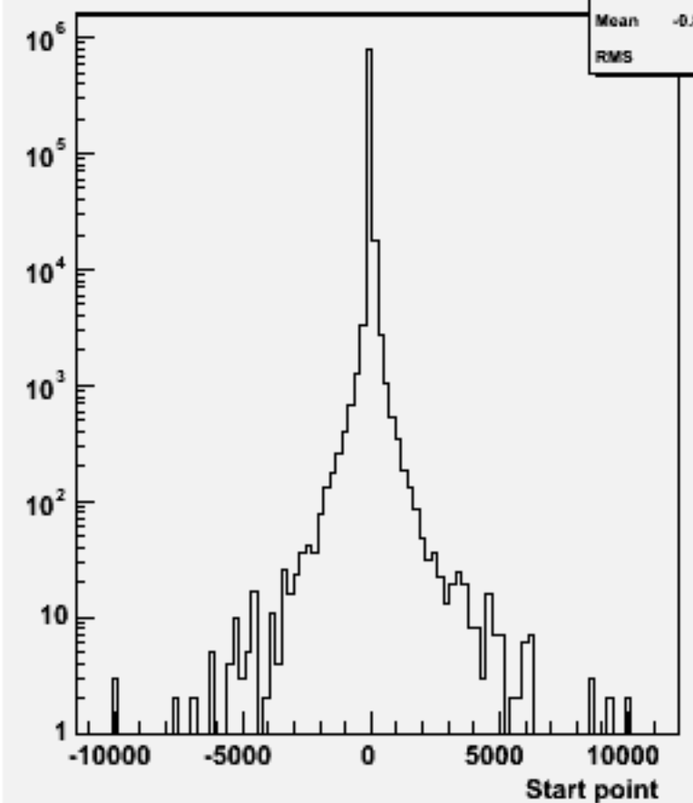
Start point Z : w101057 ddude1n1_o
