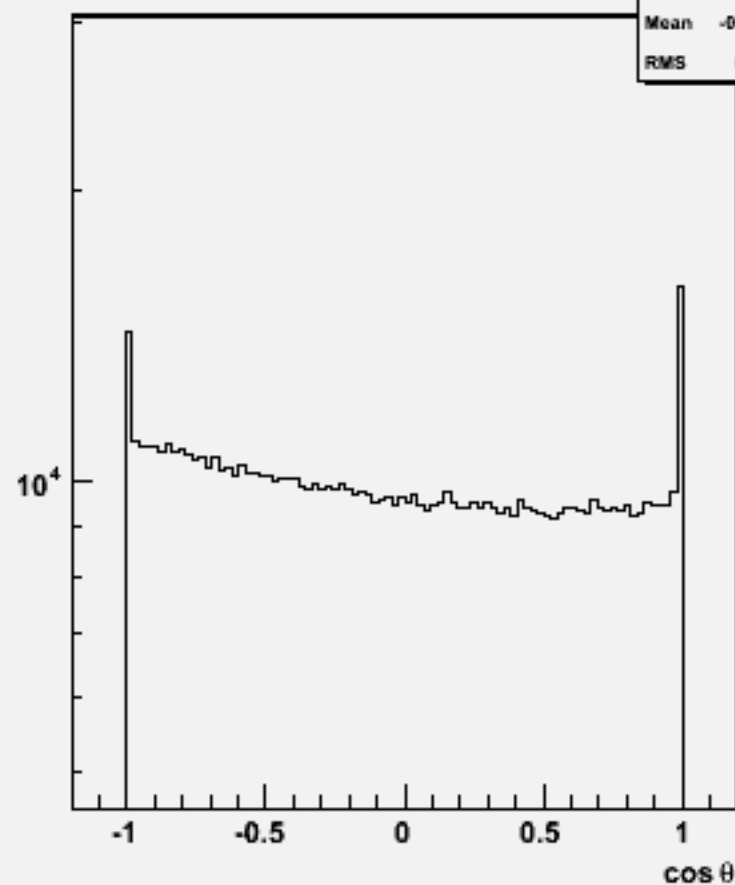
Particle cos \theta : w101057 ddude1n1_o
