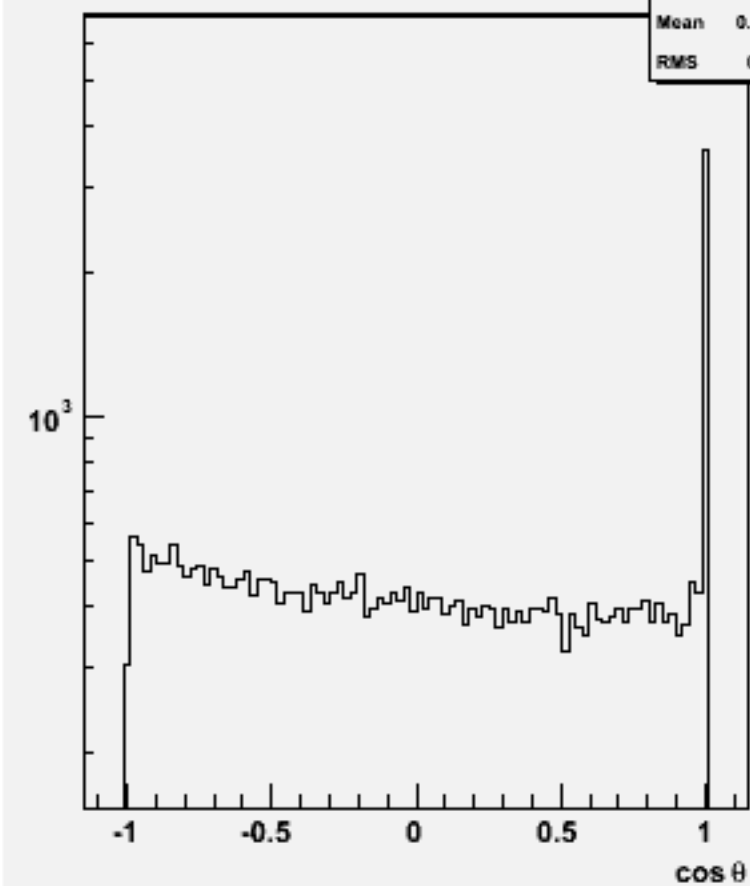
Jet cosθ (All jets)w101057 ddude1n1_o
