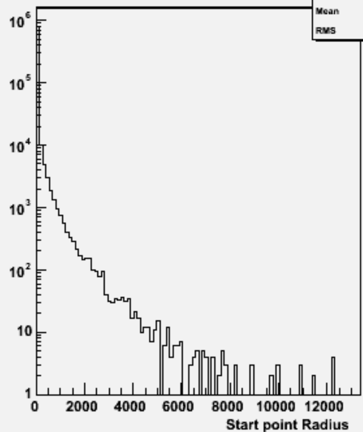
Start point R : w101057 ddude1n1_o
