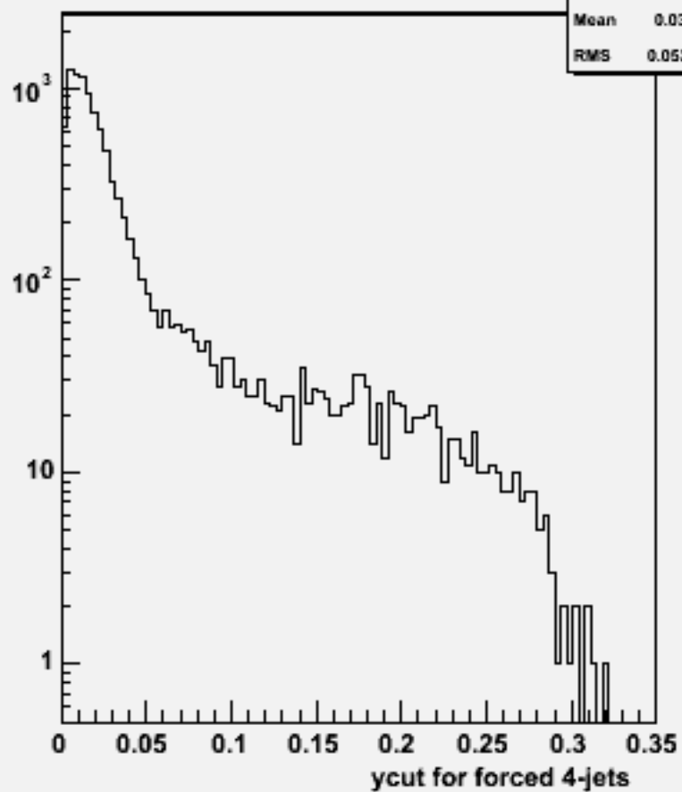
Ycut for 4-jets :w101057 ddude1n1_o
