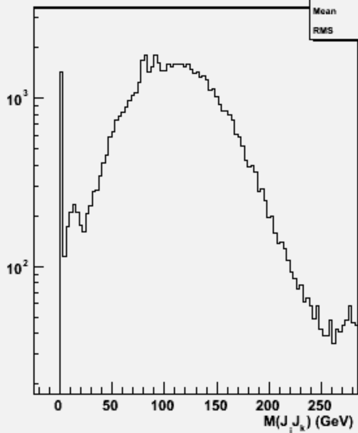
2jets mass(All comb)w101057 ddude1n1_o
