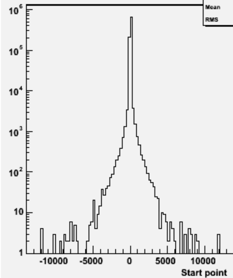
Start point Z : w101053 ddn3e3sc_o
