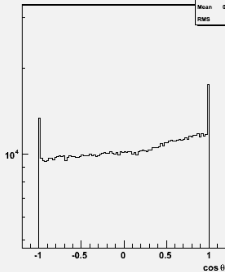
Particle cos \theta : w101053 ddn3e3sc_o
