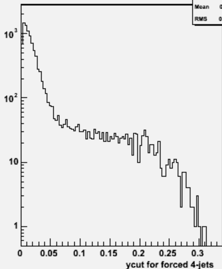
Ycut for 4-jets :w101053 ddn3e3sc_o
