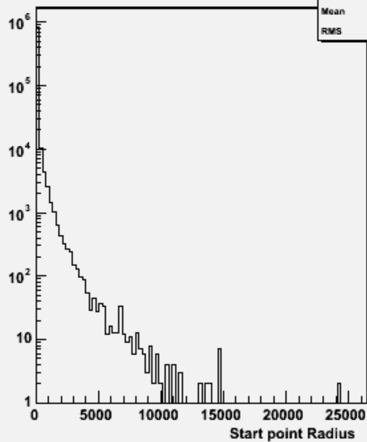
Start point R : w101053 ddn3e3sc_o
