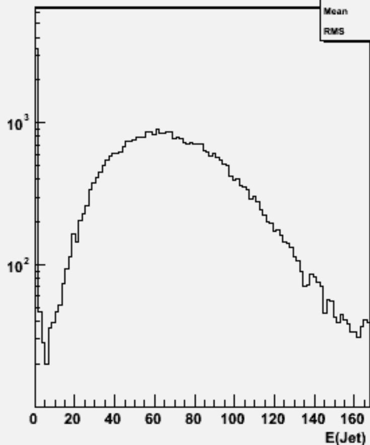
Jet energies(All jets)w101053 ddn3e3sc_o
