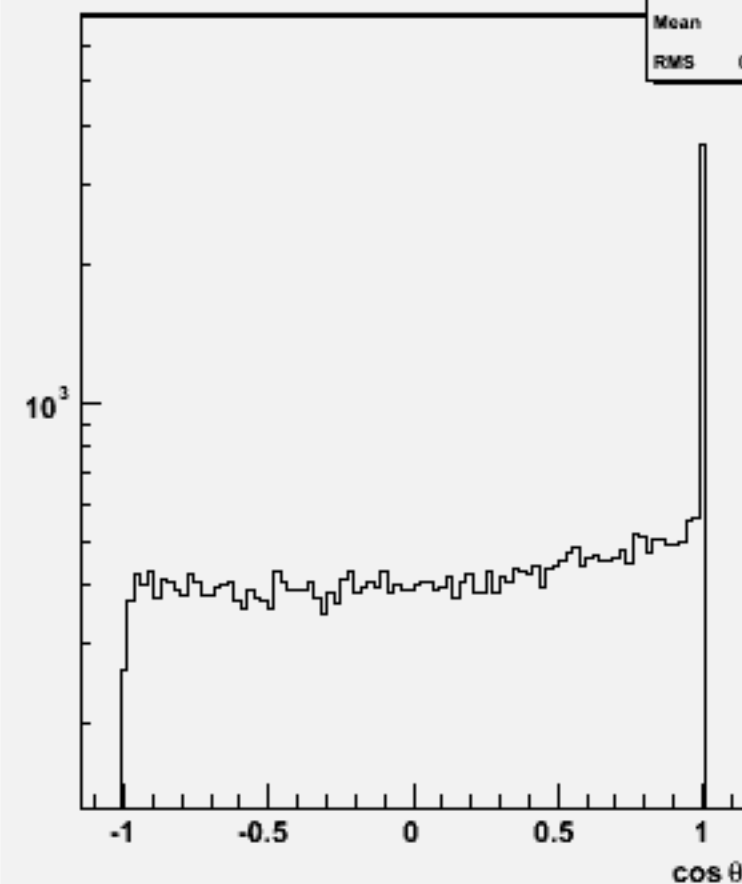
Jet cos \theta (All jets)w101053 ddn3e3sc_o
