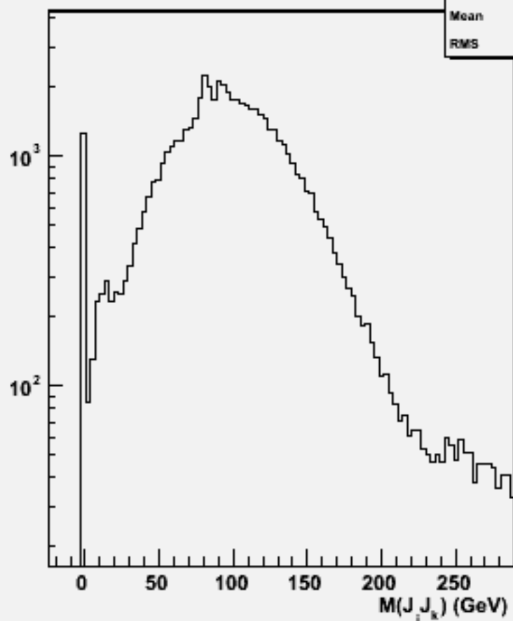
2jets mass(All comb)w101053 ddn3e3sc_o
