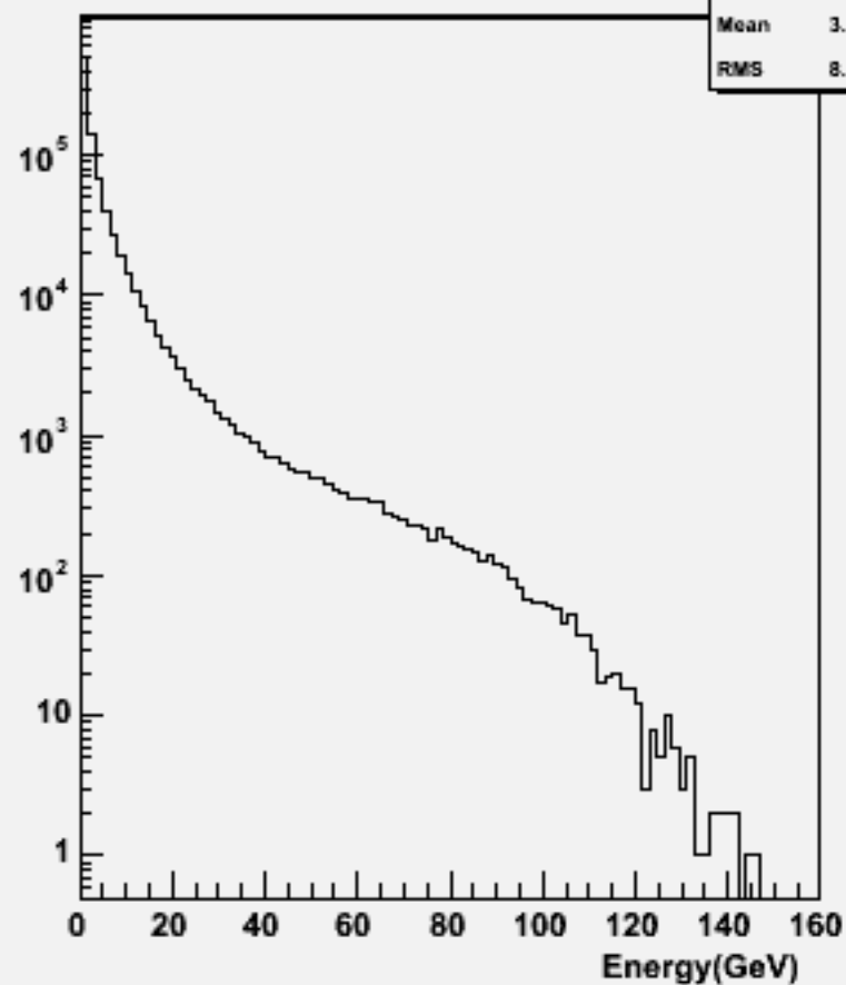
Particle Energy : w101053 ddn3e3sc_o
