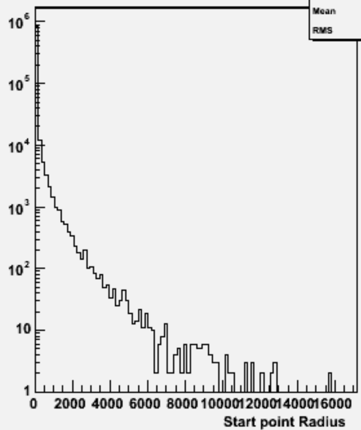
Start point R : w101052 ddn3e3sc_o
