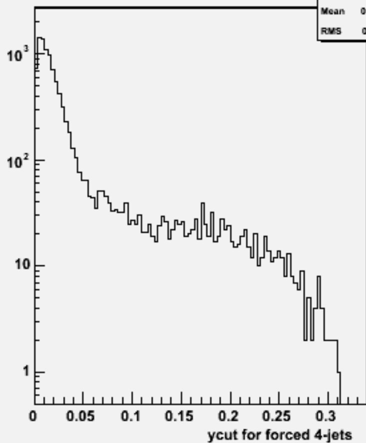
Ycut for 4-jets :w101052 ddn3e3sc_o
