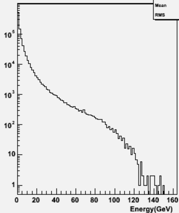
Particle Energy : w101052 ddn3e3sc_o
