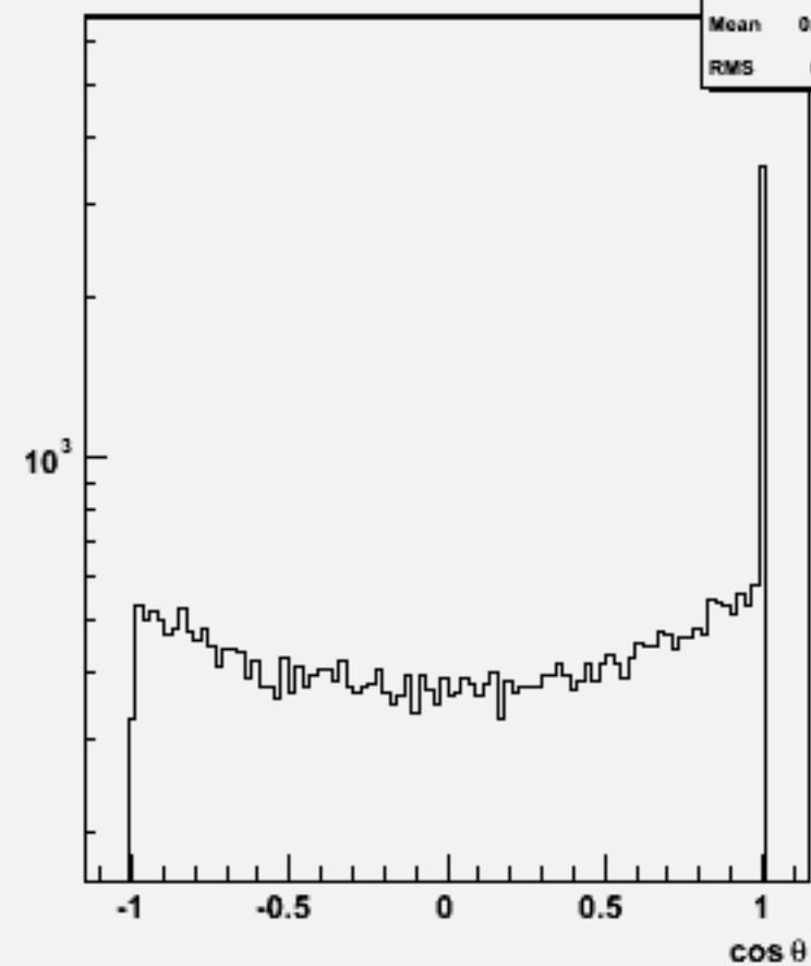
Jet cos \theta (All jets)w101052 ddn3e3sc_o
