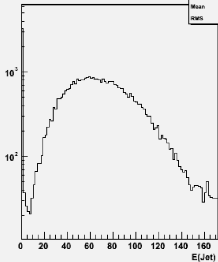
Jet energies(All jets)w101052 ddn3e3sc_o
