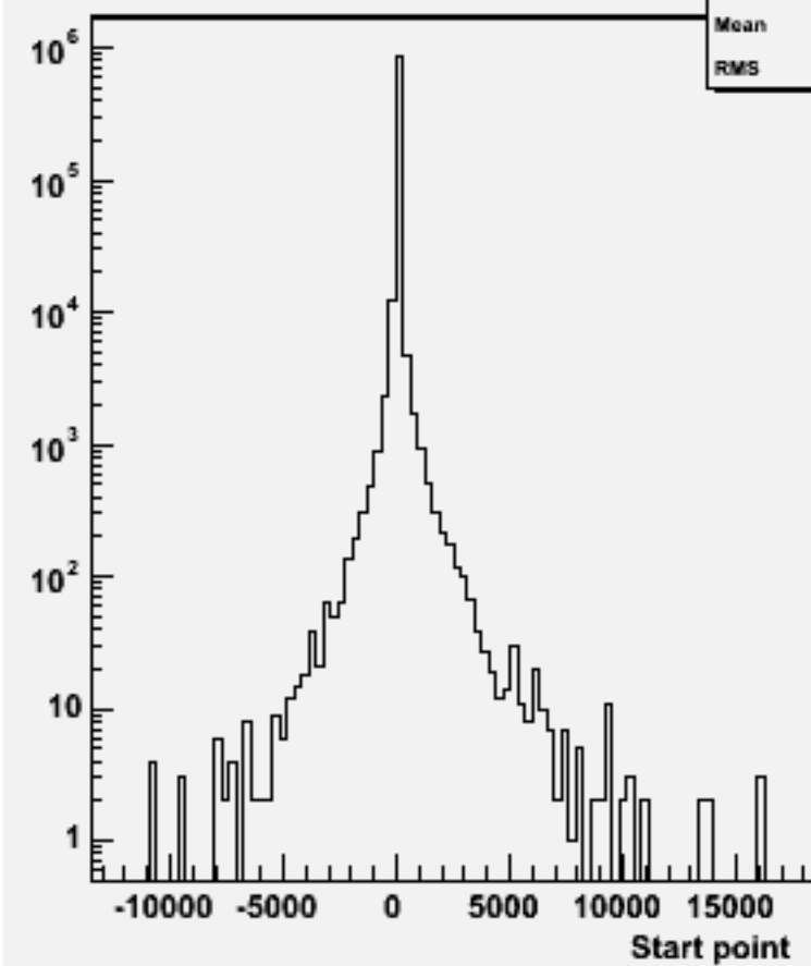
Start point Z : w101052 ddn3e3sc_o
