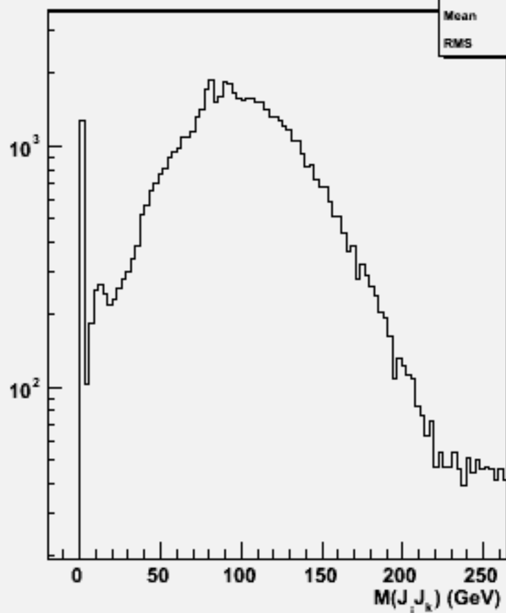
2jets mass(All comb)w101052 ddn3e3sc_o
