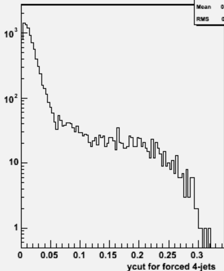
Ycut for 4-jets :w101048 ddn3e3du_o
