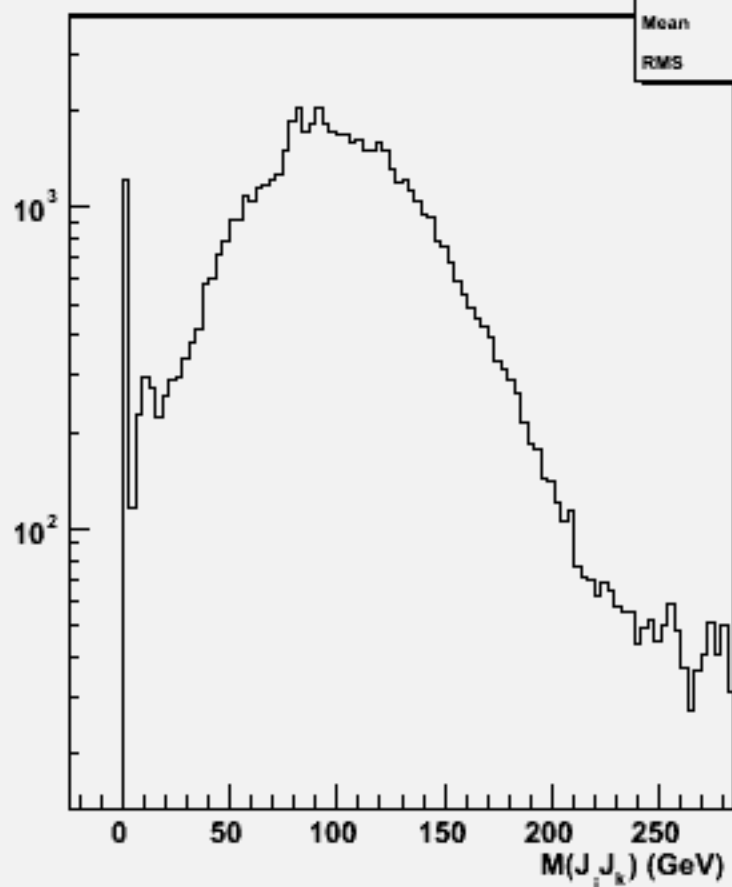
2jets mass(All comb)w101048 ddn3e3du_o
