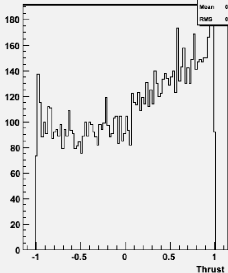
cos \Theta (thrust) w101041 ddn3e3e2n2_o
