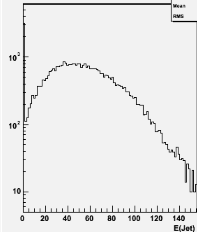
Jet energies(All jets)w101041 ddn3e3e2n2_o
