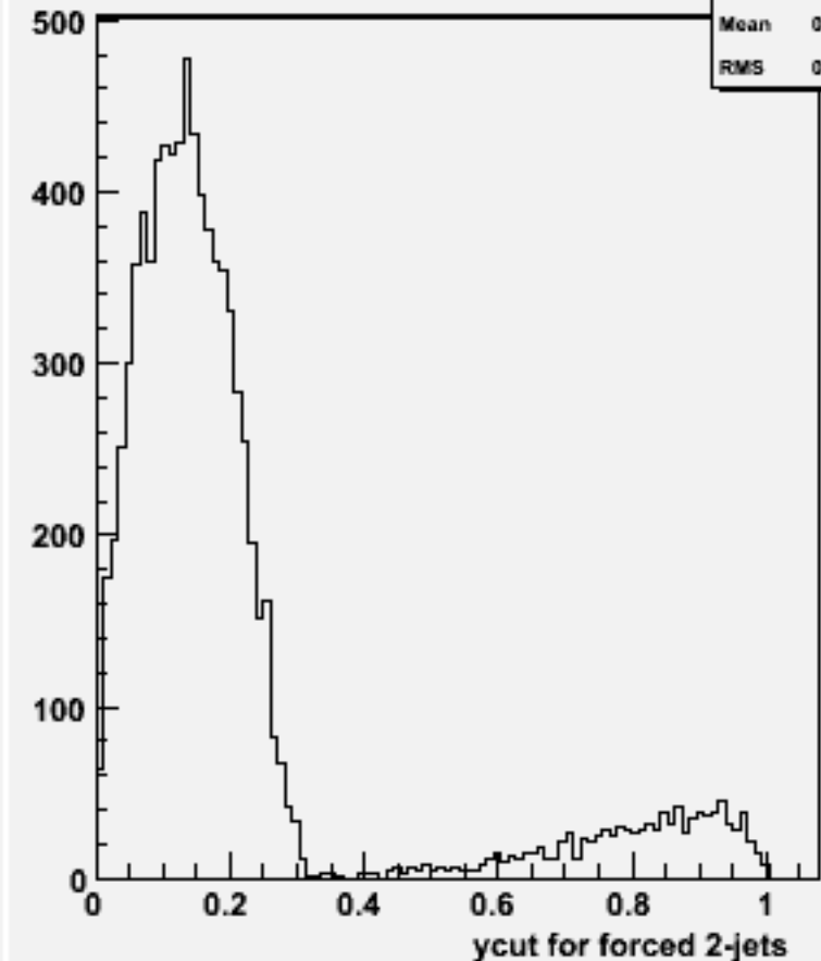
Ycut for 2-jets :w101041 ddn3e3e2n2_o
