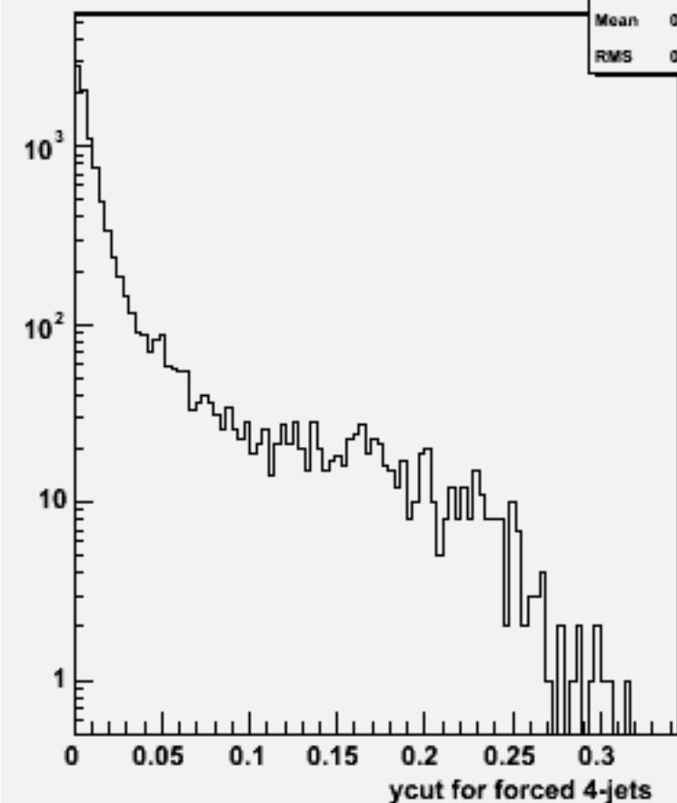
Ycut for 4-jets :w101041 ddn3e3e2n2_o
