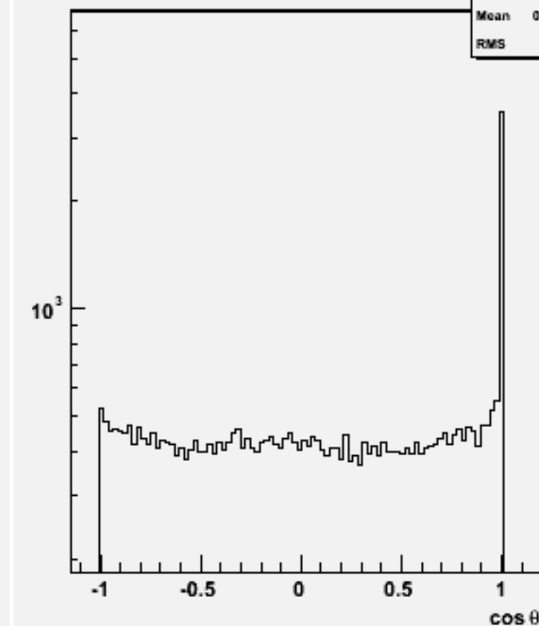
Jet cos \theta (All jets)w101041 ddn3e3e2n2_o
