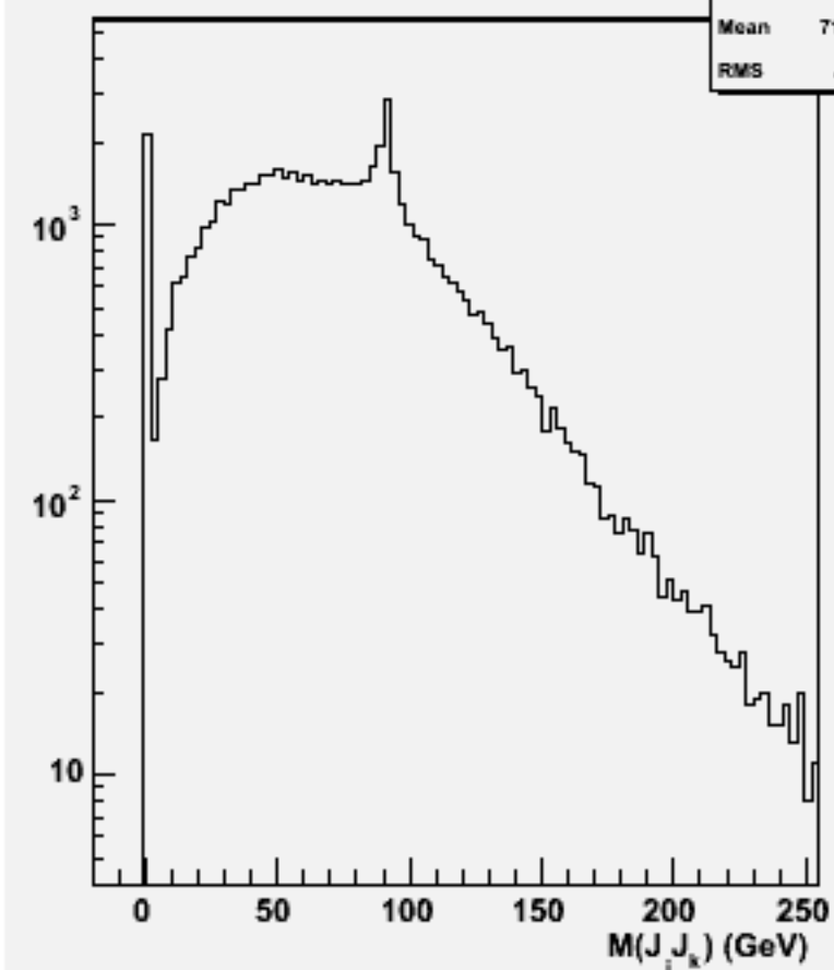
2jets mass(All comb)w101041 ddn3e3e2n2_o
