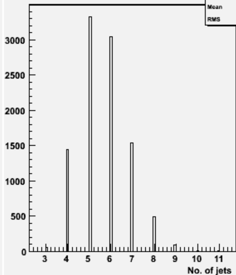
No. jets (ycut=0.001) : w101041 ddn3e3e2n2_o
