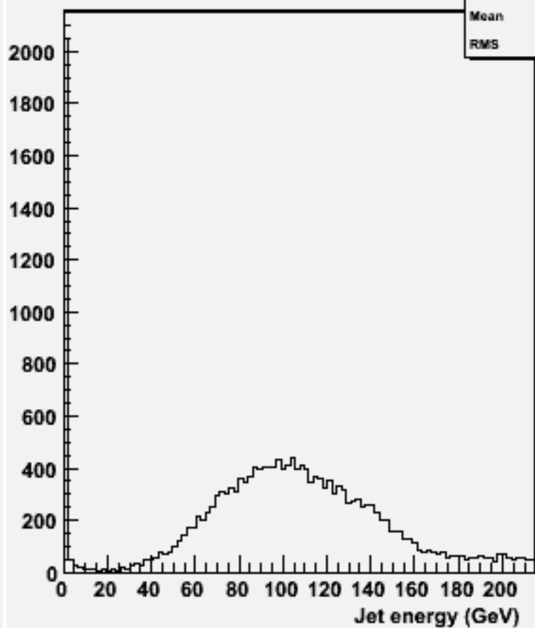
energy for 2-jets :w101041 ddn3e3e2n2_o
