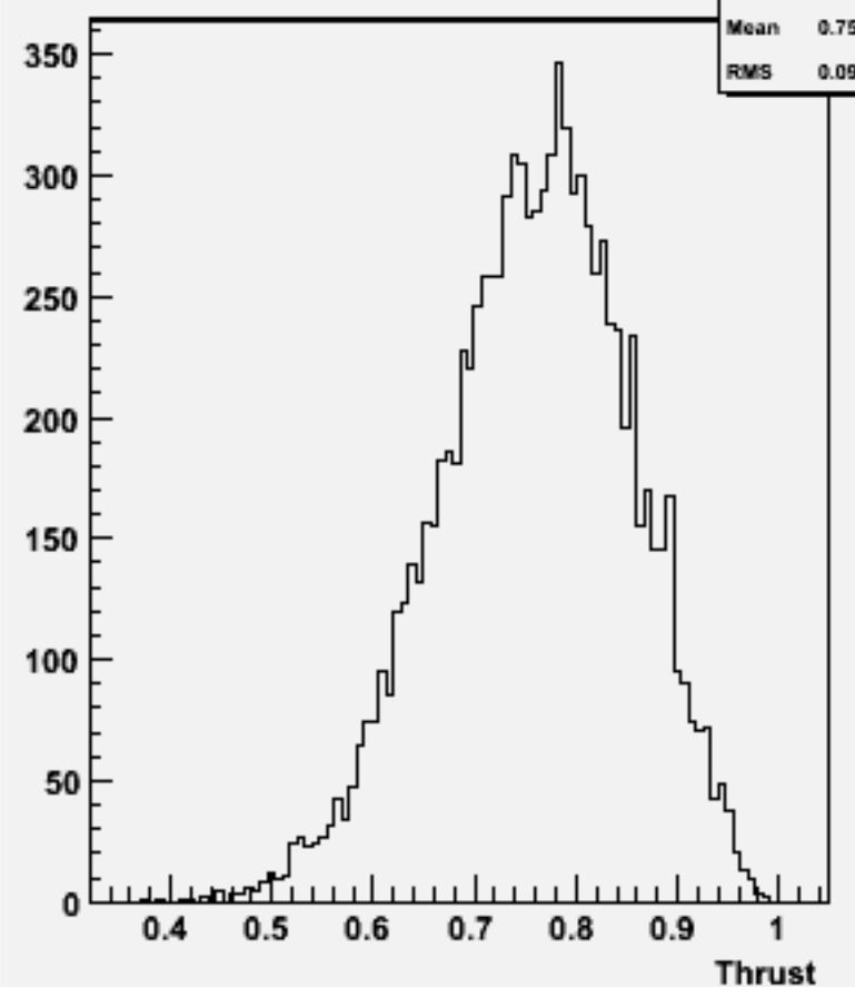
Thrust w101041 ddn3e3e2n2_o
