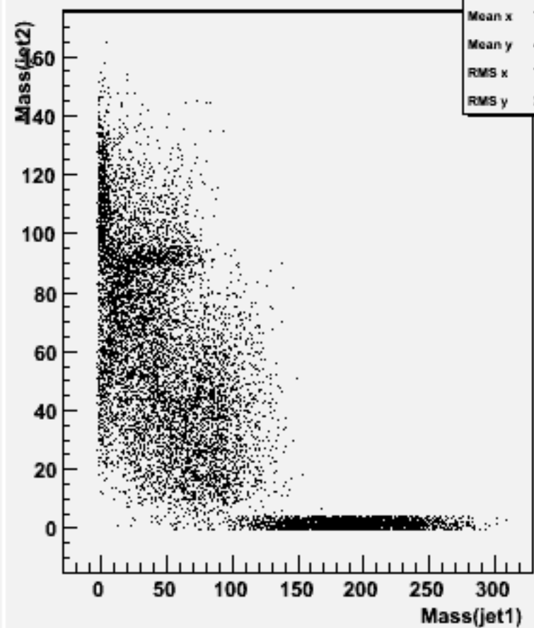
Jet mass for forced 2-jets : w101041 ddn3e3e2n2_o
