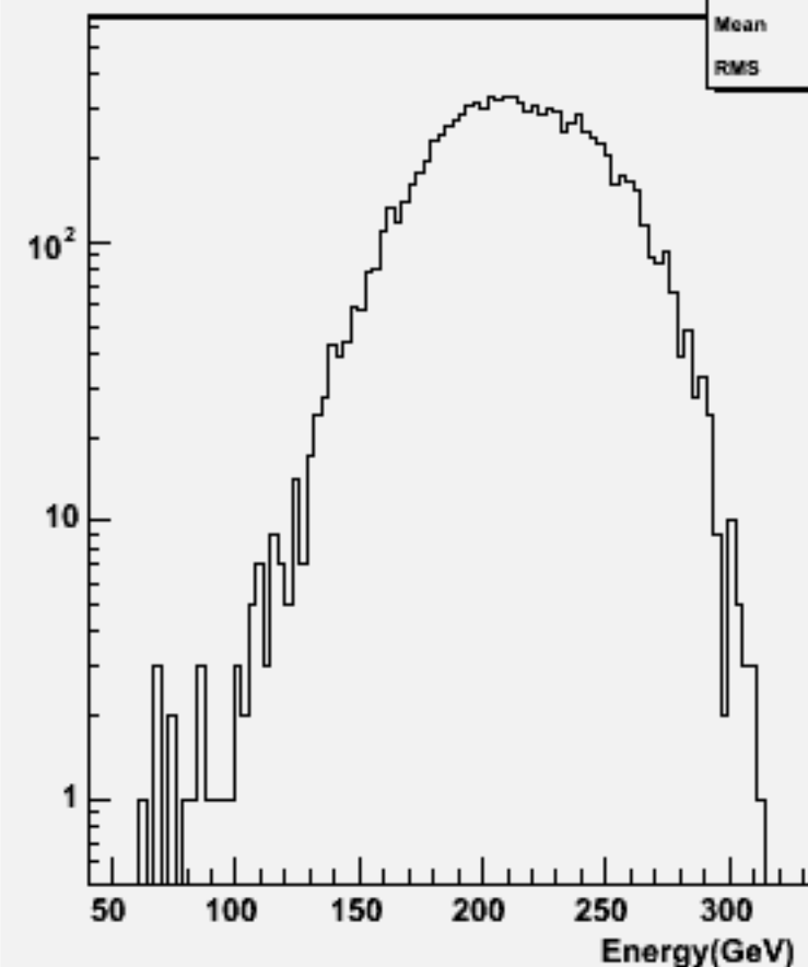
Thrust w101040 ddn3e3e2n2_o
