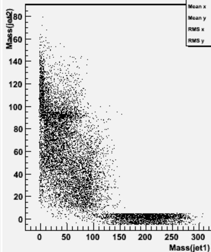
Jet mass for forced 2-jets : w101040 ddn3e3e2n2_o
