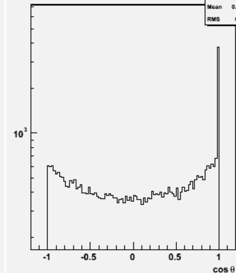
Jet cos \theta (All jets)w101040 ddn3e3e2n2_o
