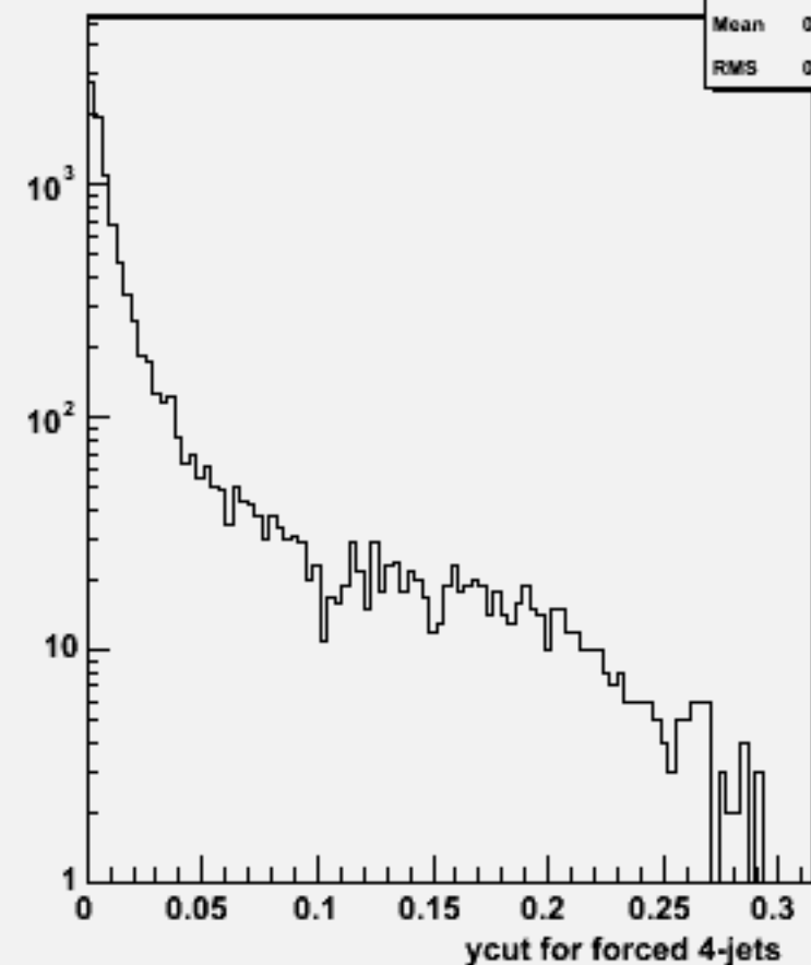
Ycut for 4-jets :w101040 ddn3e3e2n2_o
