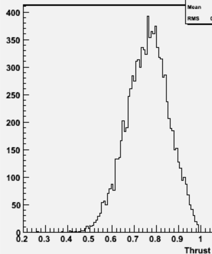
Thrust w101040 ddn3e3e2n2_o
