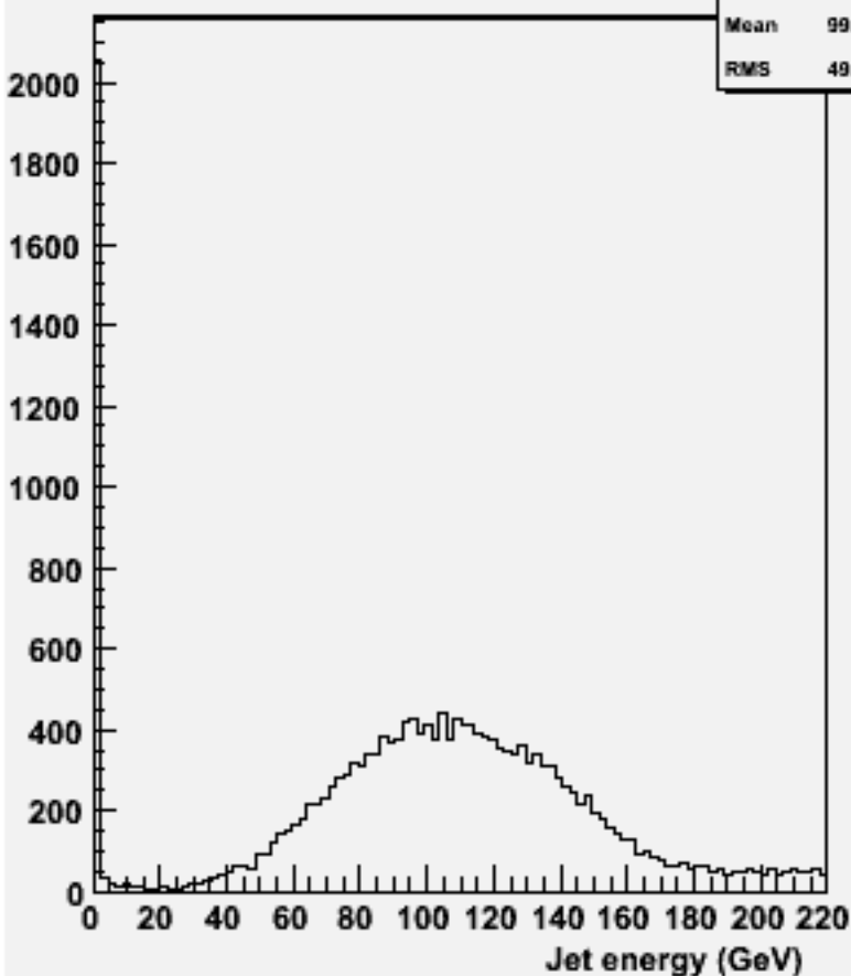
energy for 2-jets :w101040 ddn3e3e2n2_o
