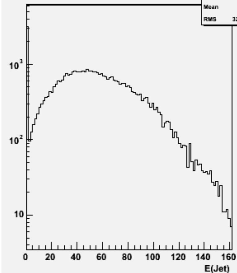
Jet energies(All jets)w101040 ddn3e3e2n2_o
