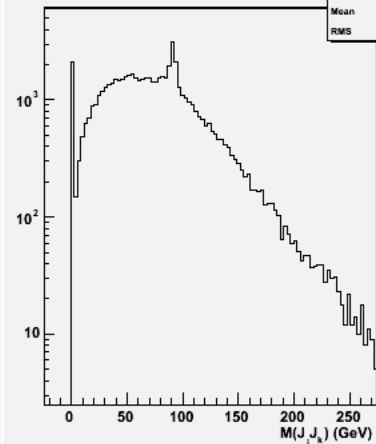
2jets mass(All comb)w101040 ddn3e3e2n2_o
