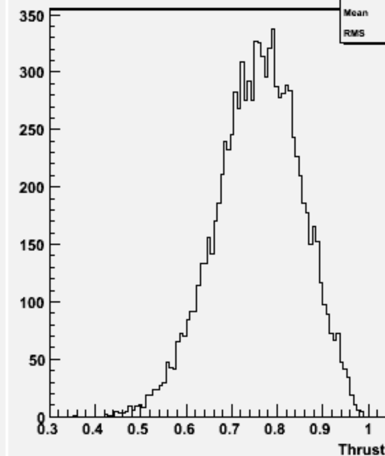
Thrust w101037 ddn3e3e1n1_o
