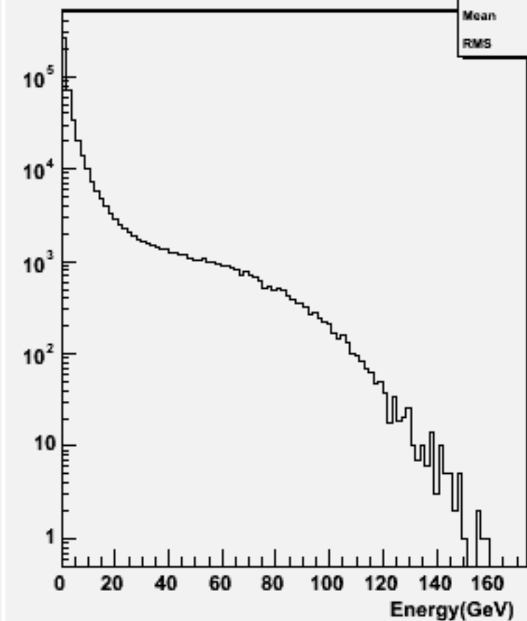
Particle Energy : w101037 ddn3e3e1n1_o
