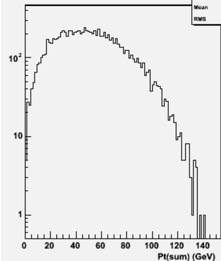
Pt Sum: w101037 ddn3e3e1n1_o
