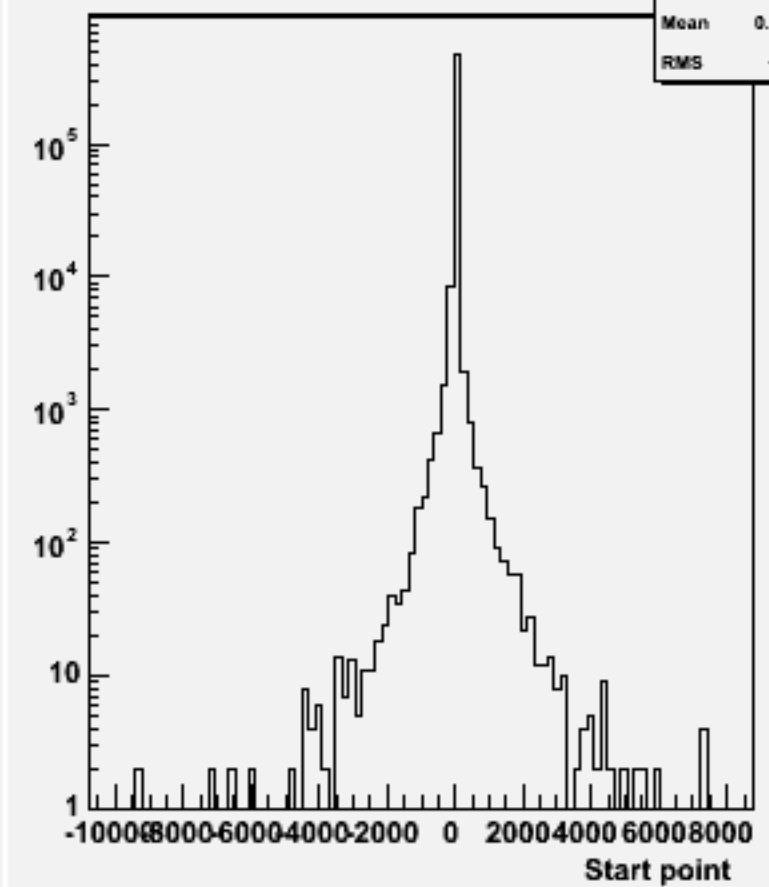
Start point Z : w101037 ddn3e3e1n1_o
