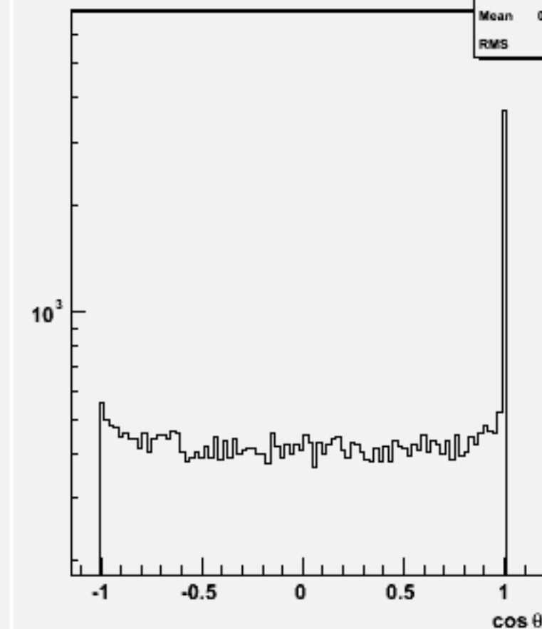
Jet cos \theta (All jets)w101037 ddn3e3e1n1_o
