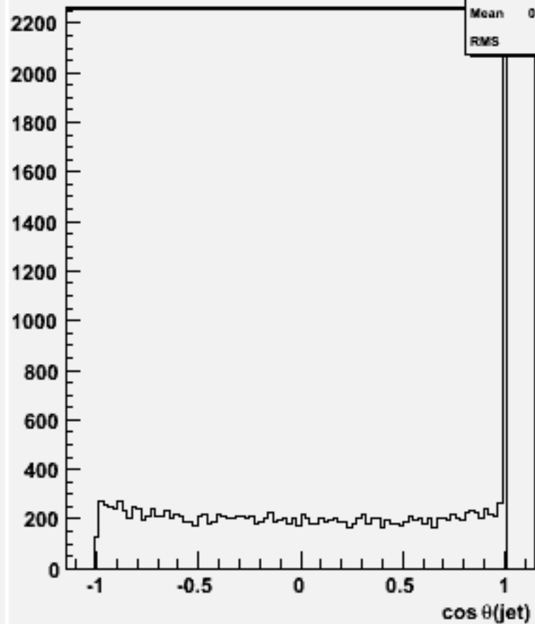
cos \theta for 2-jets :w101037 ddn3e3e1n1_o
