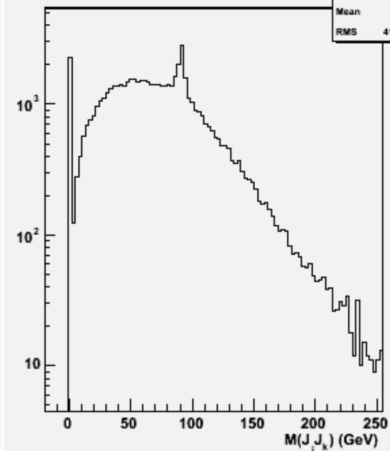
2jets mass(All comb)w101037 ddn3e3e1n1_o
