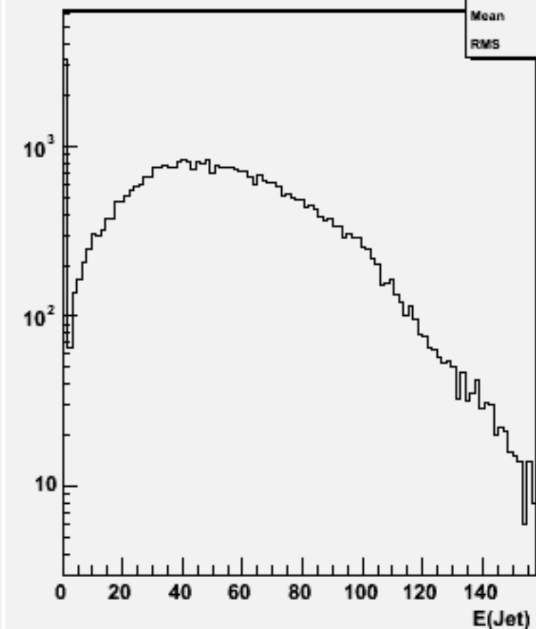
Jet energies(All jets)w101037 ddn3e3e1n1_o
