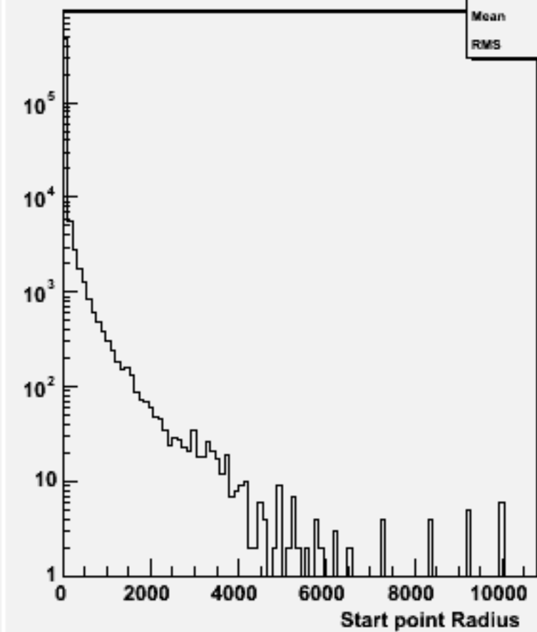
Start point R : w101037 ddn3e3e1n1_o
