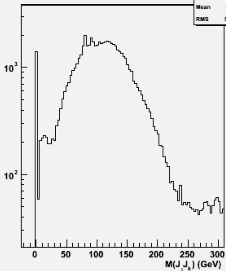
2jets mass(All comb)w101033 ddn2e2sc_o
