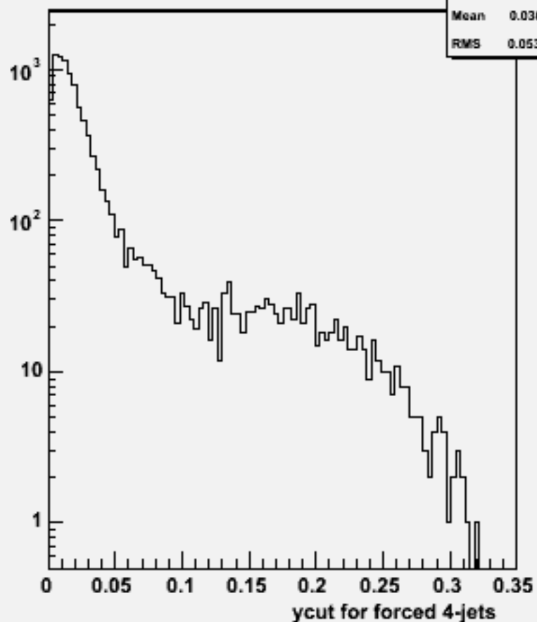
Ycut for 4-jets :w101033 ddn2e2sc_o
