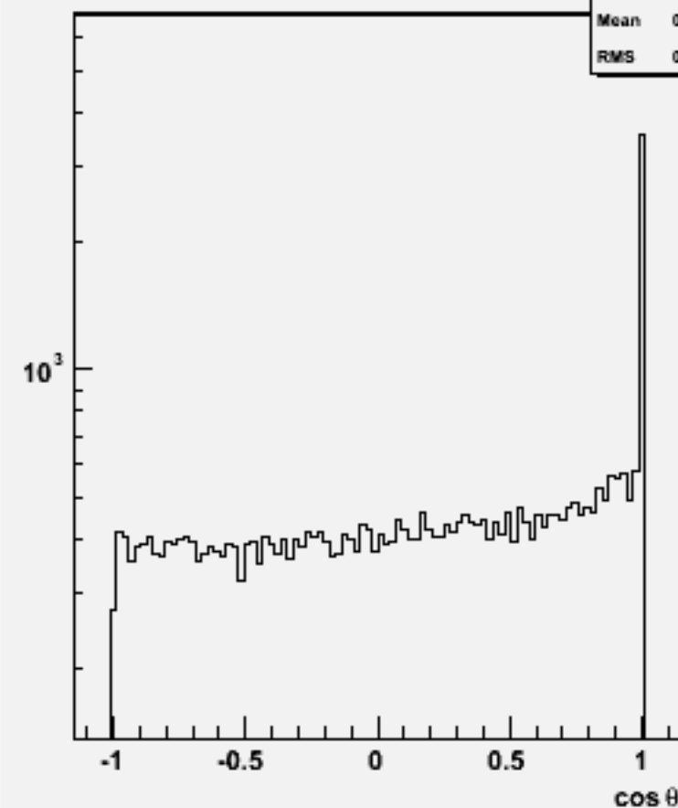
Jet cos \theta (All jets)w101033 ddn2e2sc_o
