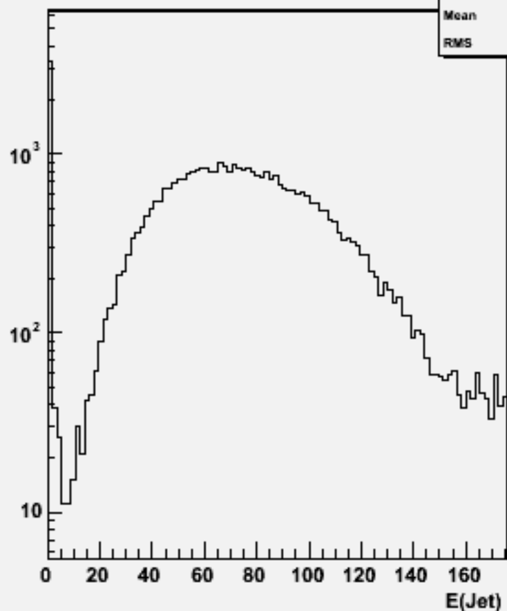
Jet energies(All jets)w101033 ddn2e2sc_o
