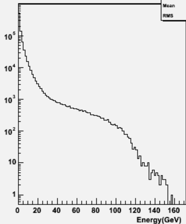
Particle Energy : w101032 ddn2e2sc_o
