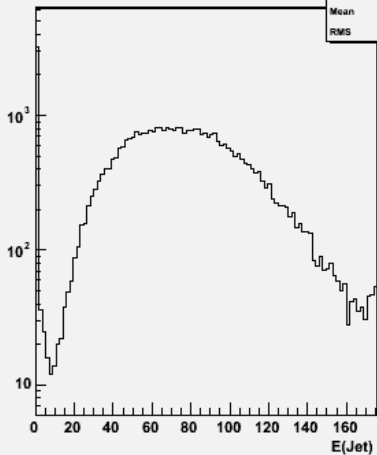
Jet energies(All jets)w101032 ddn2e2sc_o
