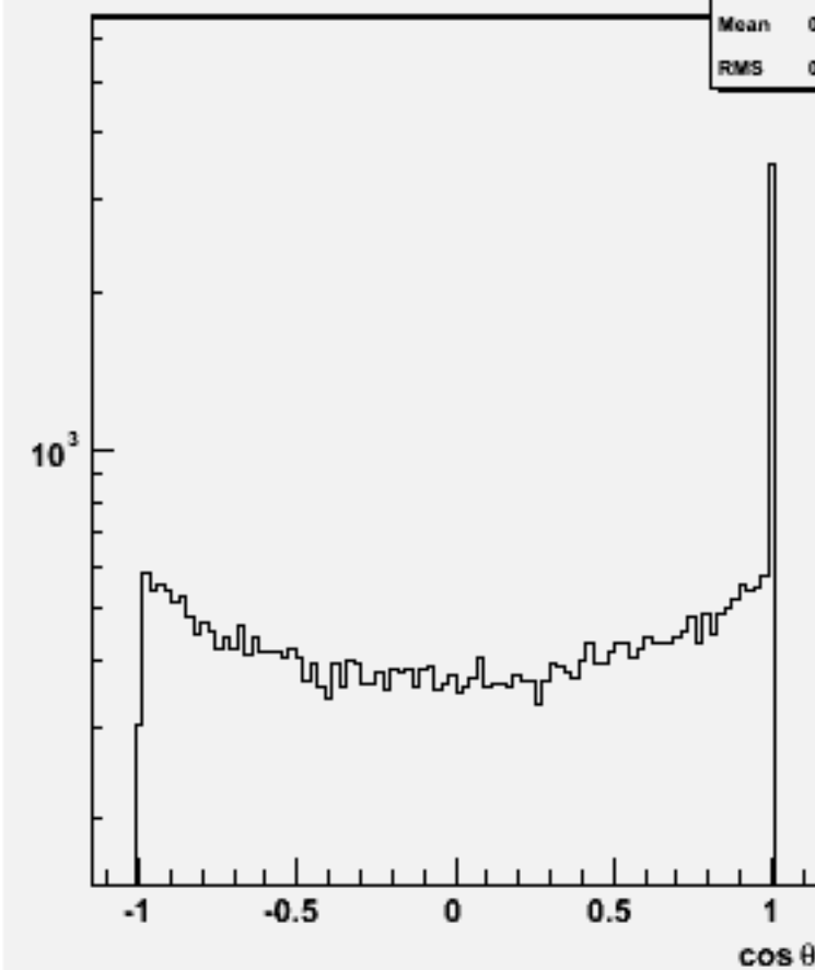
Jet cos \theta (All jets)w101032 ddn2e2sc_o
