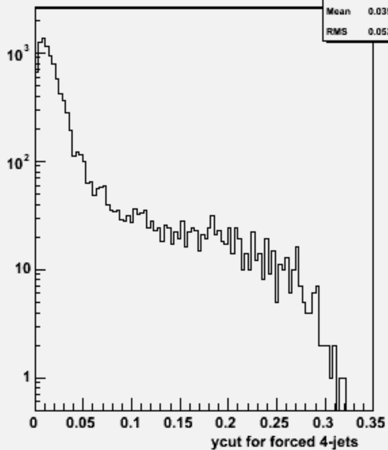
Ycut for 4-jets :w101032 ddn2e2sc_o
