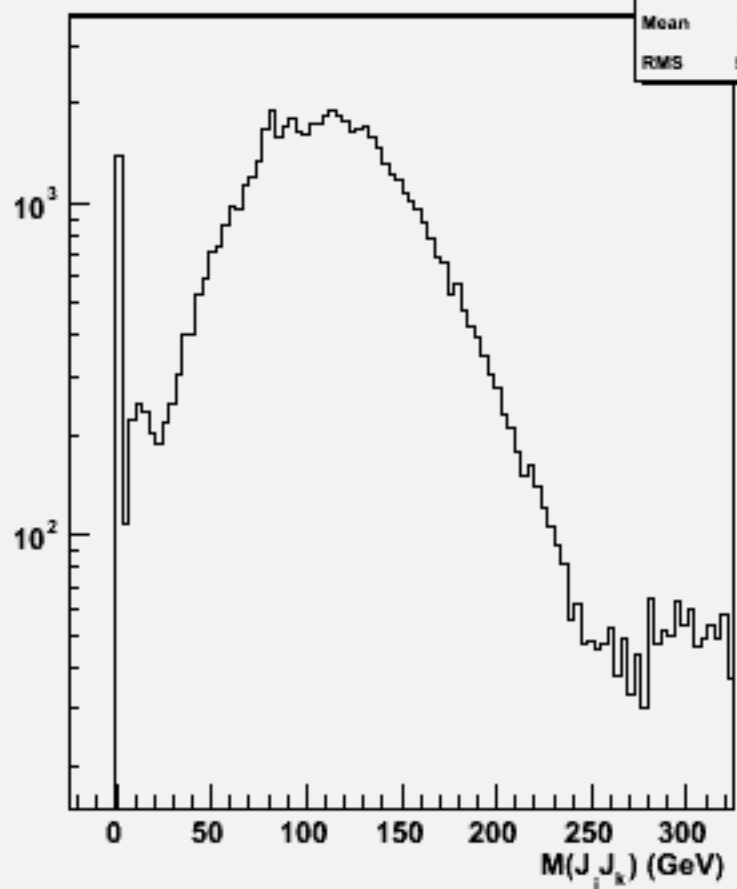
2jets mass(All comb)w101032 ddn2e2sc_o
