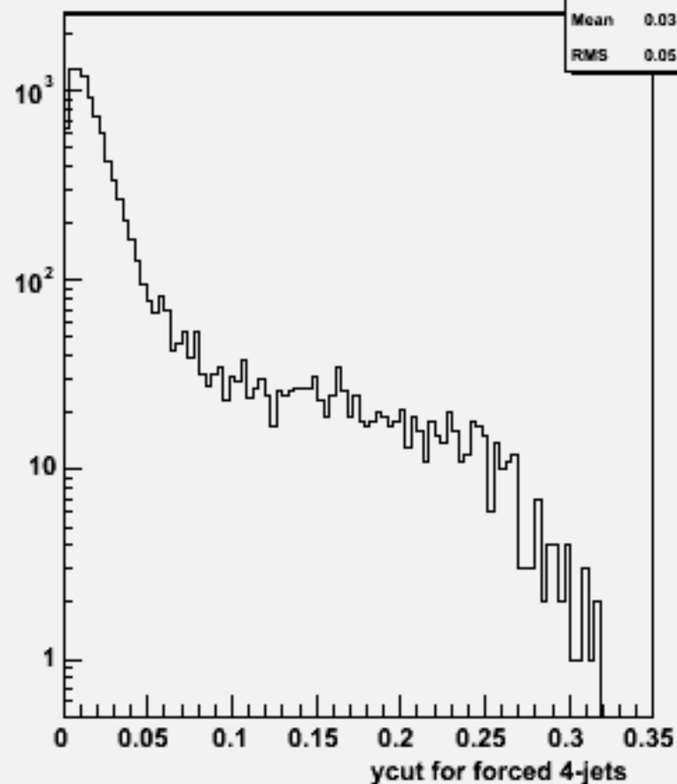
Ycut for 4-jets :w101028 ddn2e2du_o
