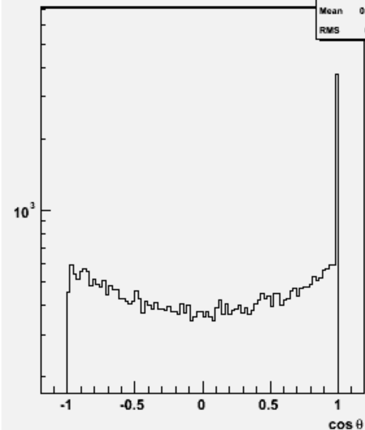
Jet cos \theta (All jets)w101028 ddn2e2du_o
