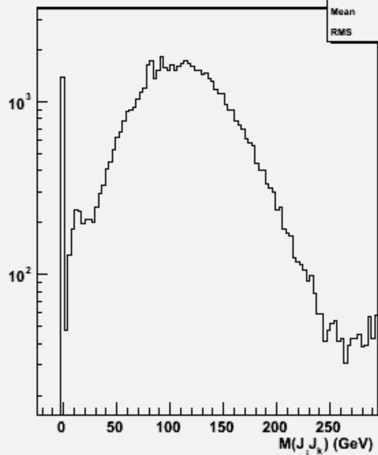
2jets mass(All comb)w101028 ddn2e2du_o
