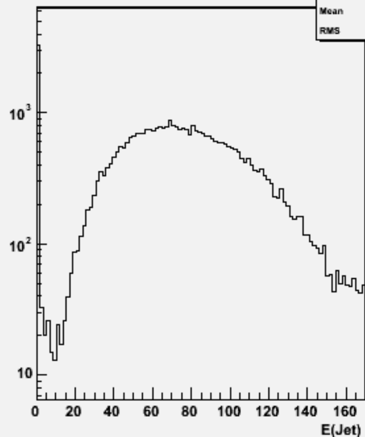
Jet energies(All jets)w101028 ddn2e2du_o
