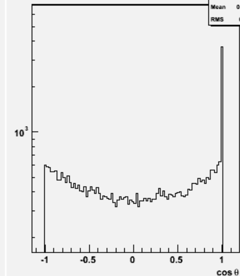
Jet cos \theta (All jets)w101024 ddn2e2e3n3_o
