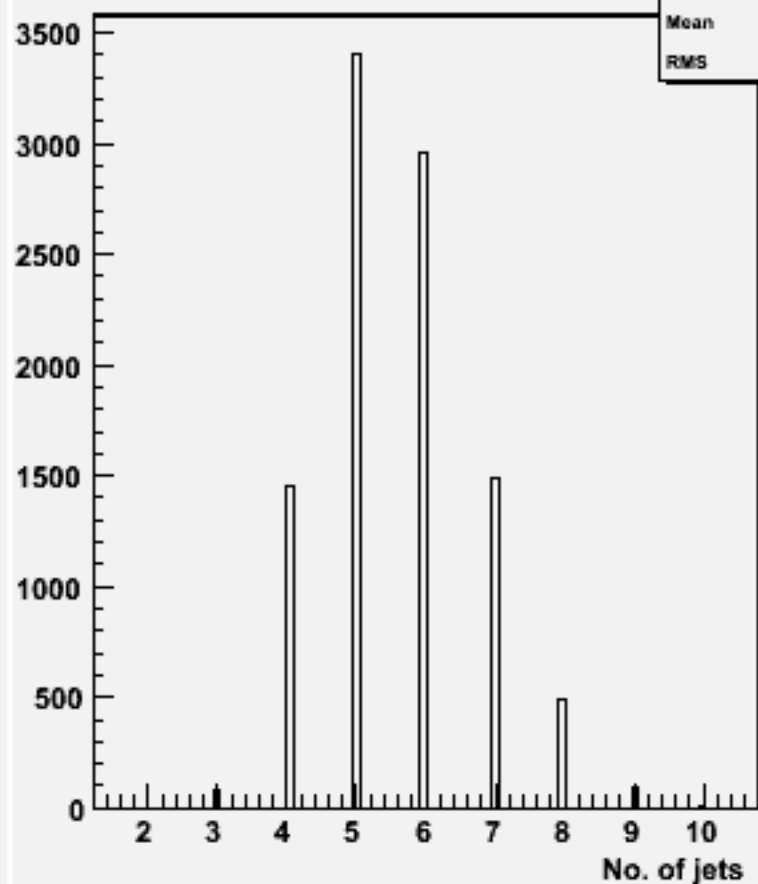
No. jets (ycut=0.001) : w101024 ddn2e2e3n3_o
