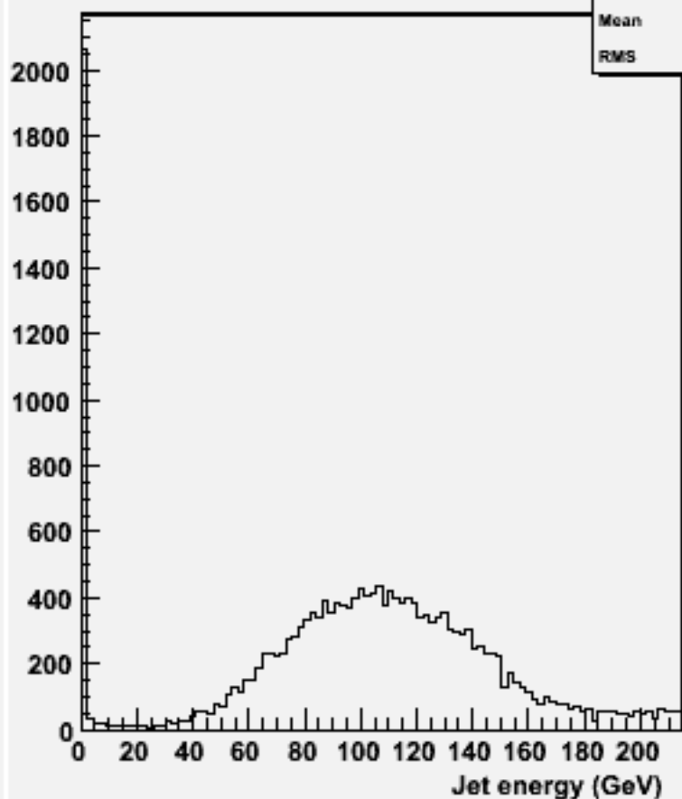
energy for 2-jets :w101024 ddn2e2e3n3_o
