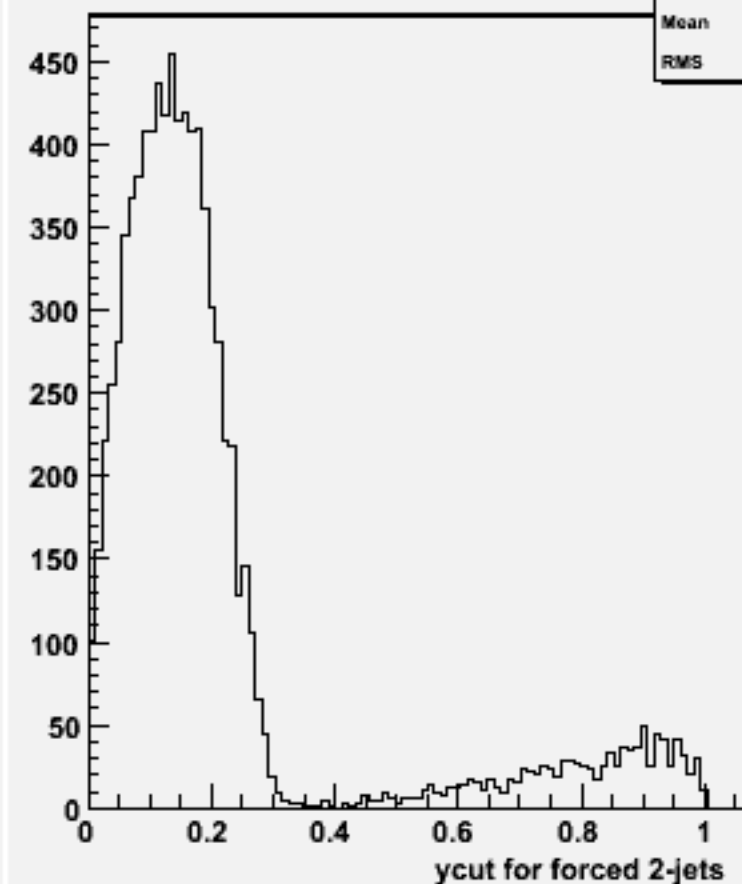
Ycut for 2-jets :w101024 ddn2e2e3n3_o
