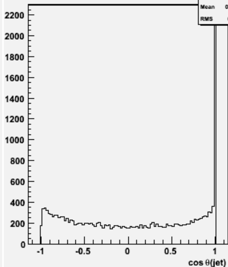
cos \theta for 2-jets :w101024 ddn2e2e3n3_o
