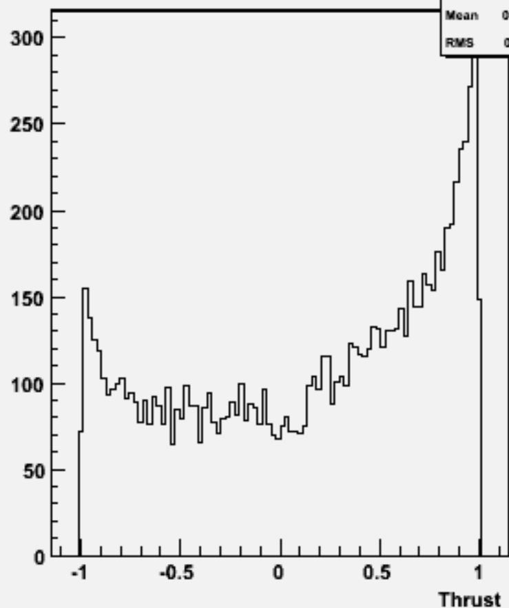
cos \Theta (thrust) w101024 ddn2e2e3n3_o
