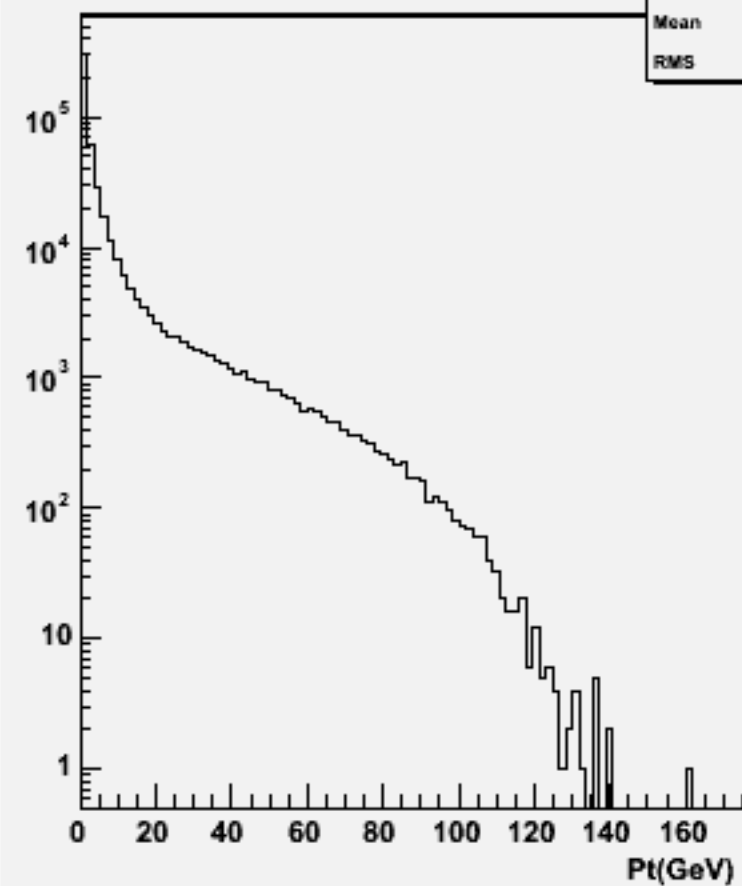
Start point Z : w101024 ddn2e2e3n3_o
