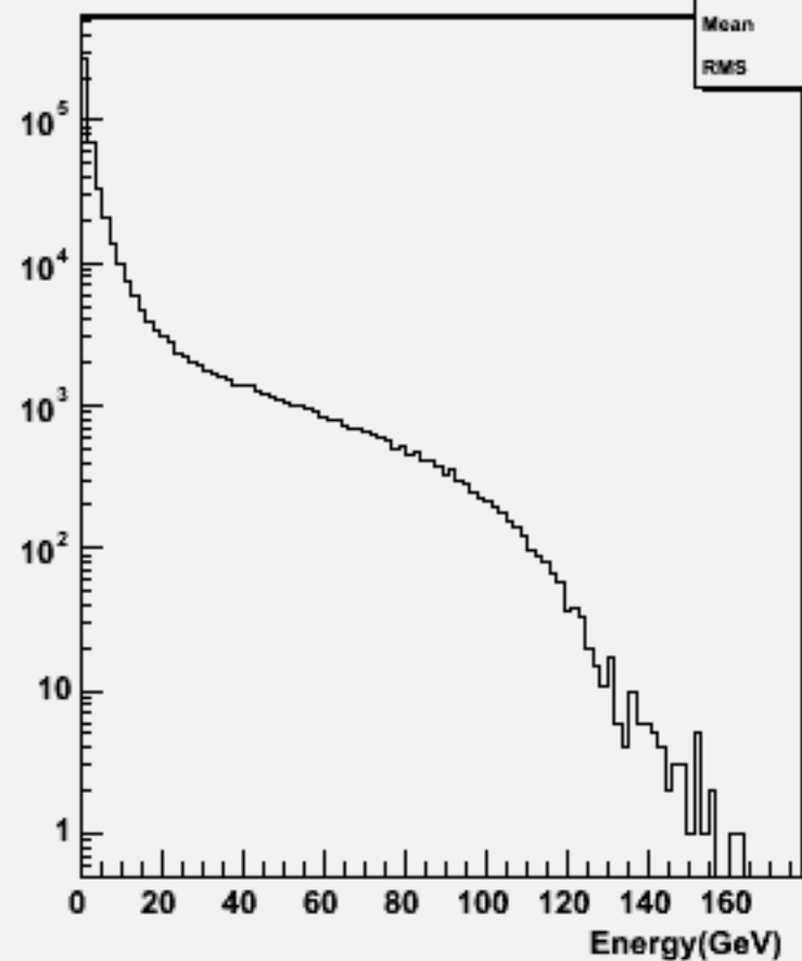
Start point R : w101024 ddn2e2e3n3_o
