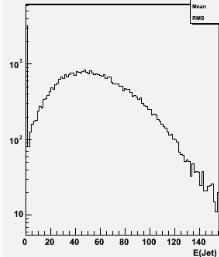
Jet energies(All jets)w101024 ddn2e2e3n3_o
