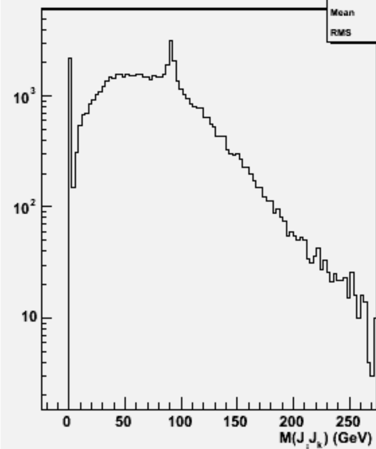
2jets mass(All comb)w101024 ddn2e2e3n3_o
