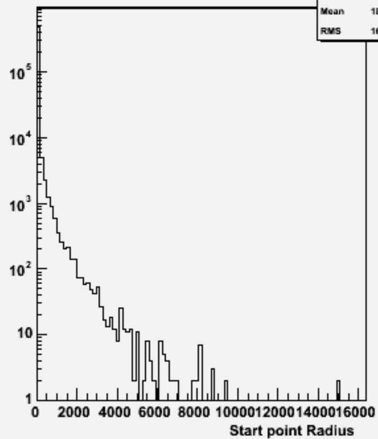
Start point R : w101024 ddn2e2e3n3_o
