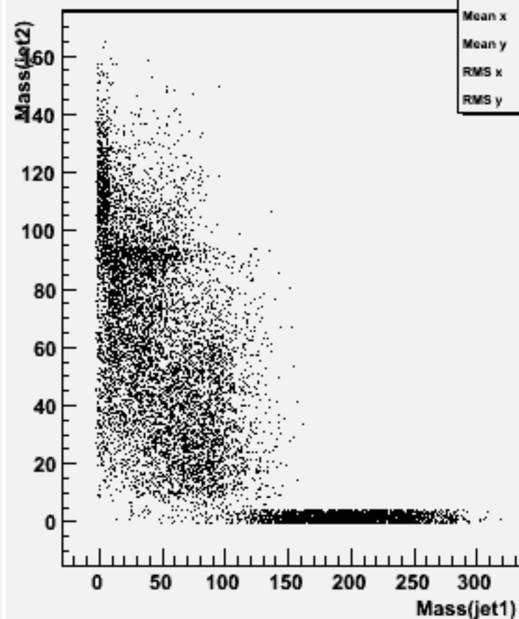
Jet mass for forced 2-jets : w101024 ddn2e2e3n3_o
