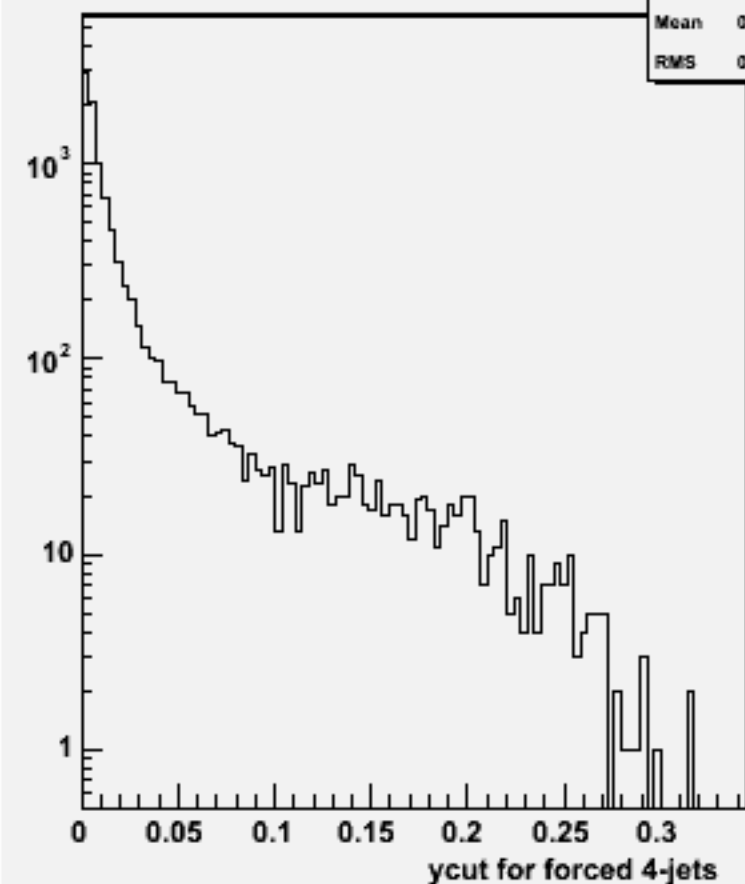
Ycut for 4-jets :w101024 ddn2e2e3n3_o
