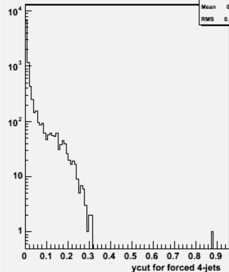
Ycut for 4-jets :w101021 ddn2e2e2n2_o
