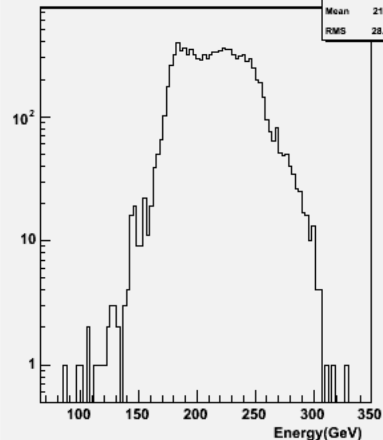
Thrust w101021 ddn2e2e2n2_o
