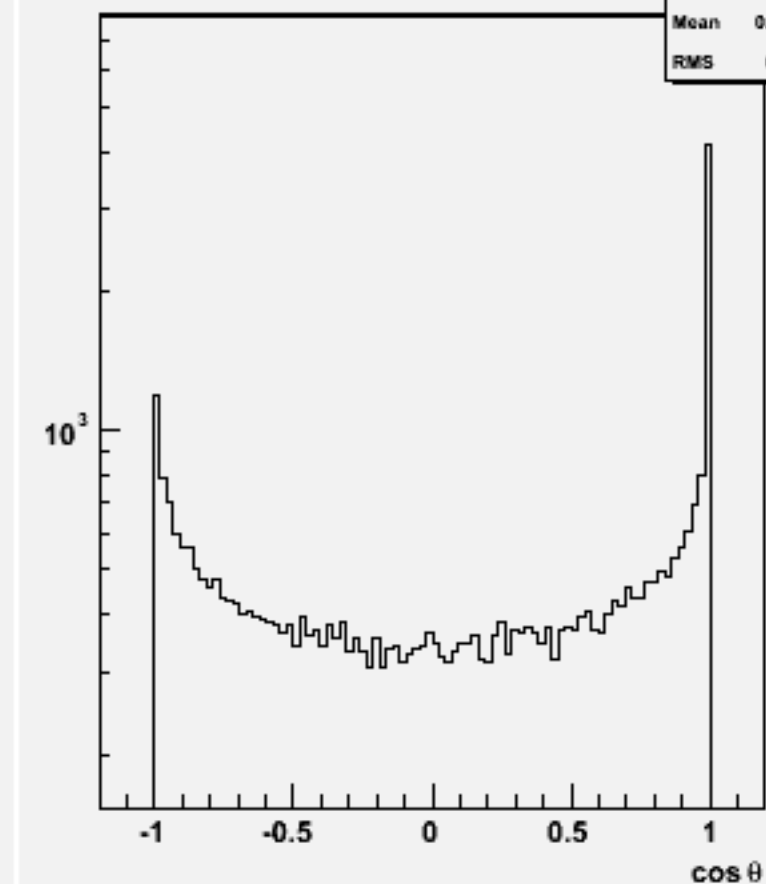
Jet cos \theta (All jets)w101021 ddn2e2e2n2_o
