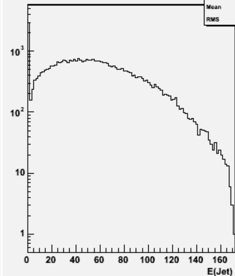
Jet energies(All jets)w101021 ddn2e2e2n2_o
