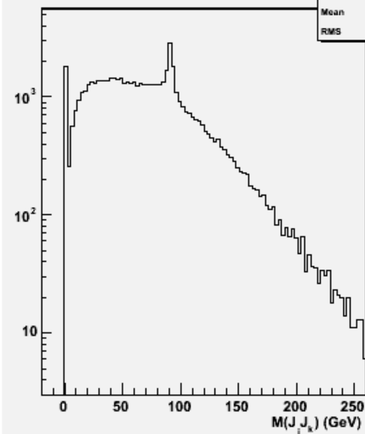
2jets mass(All comb)w101021 ddn2e2e2n2_o
