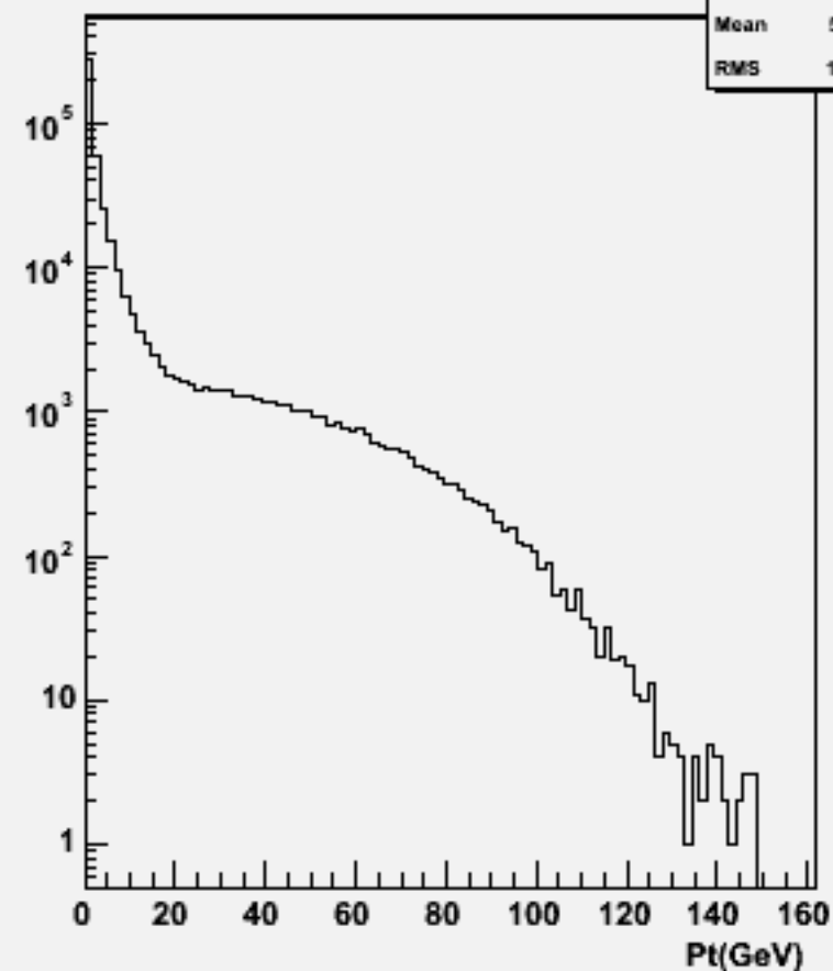
Start point Z : w101017 ddn2e2e1n1_o
