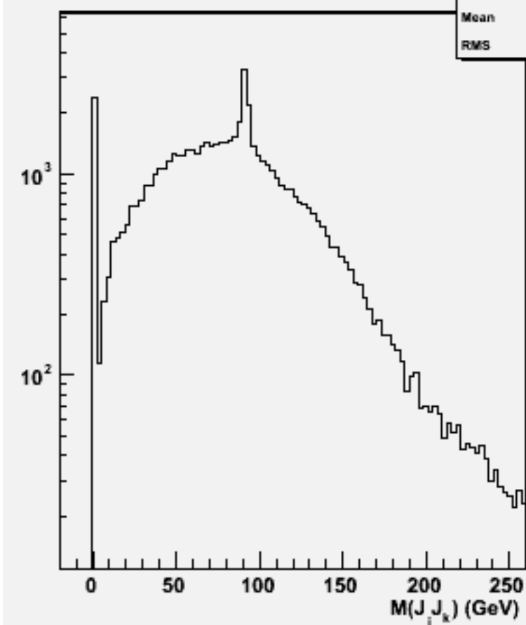
2jets mass(All comb)w101017 ddn2e2e1n1_o
