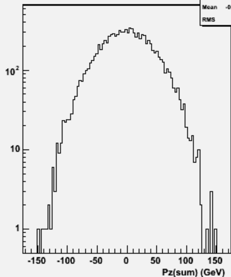
Pz Sum: w101017 ddn2e2e1n1_o
