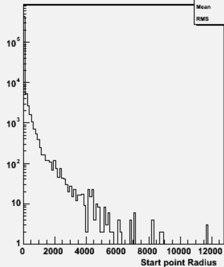
Start point R : w101017 ddn2e2e1n1_o
