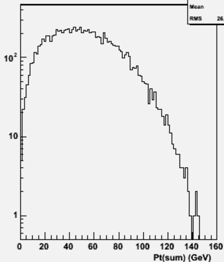
Pt Sum: w101017 ddn2e2e1n1_o
