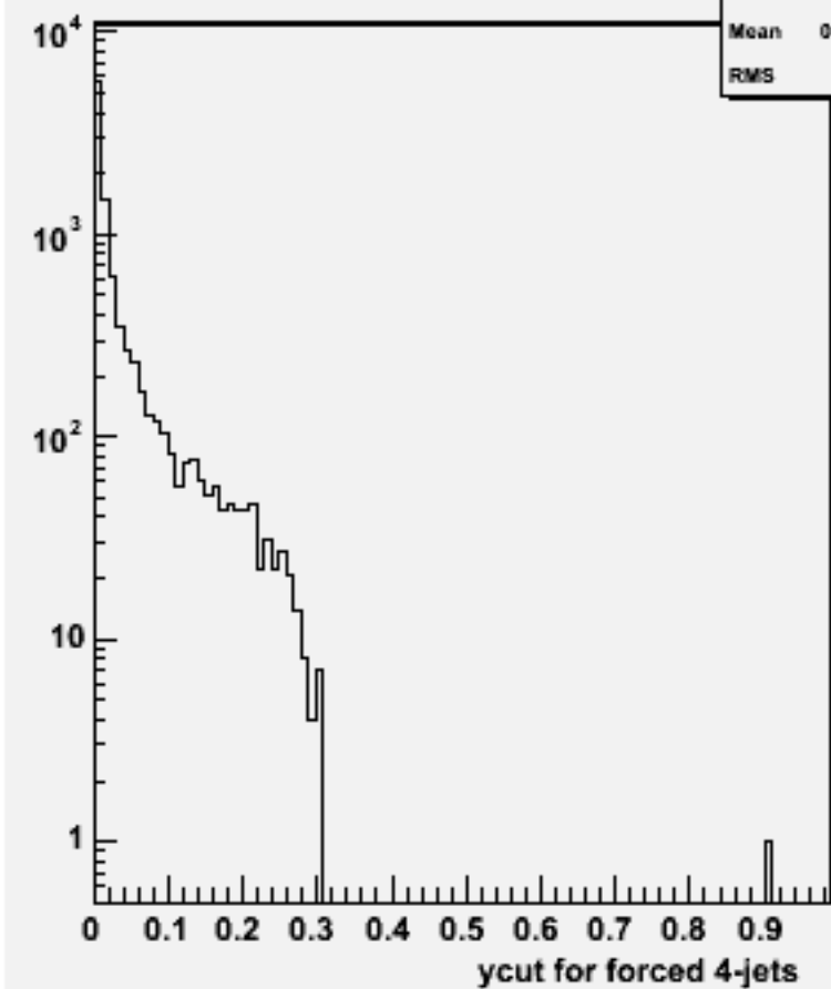
Ycut for 4-jets :w101017 ddn2e2e1n1_o
