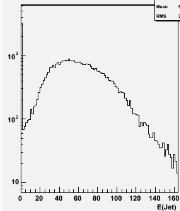
Jet energies(All jets)w101017 ddn2e2e1n1_o
