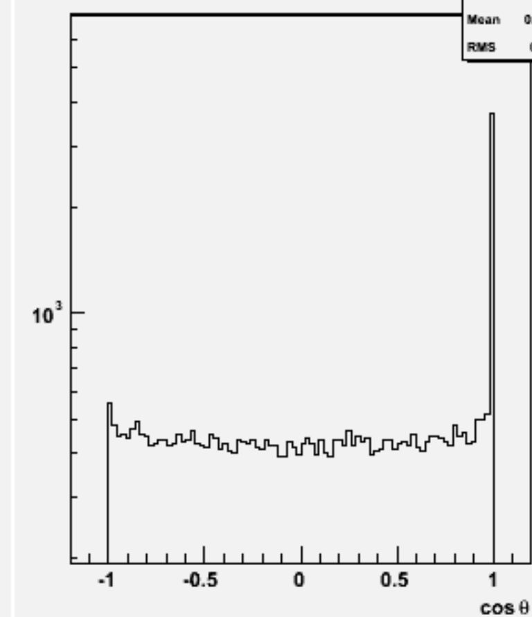
Jet cos \theta (All jets)w101017 ddn2e2e1n1_o
