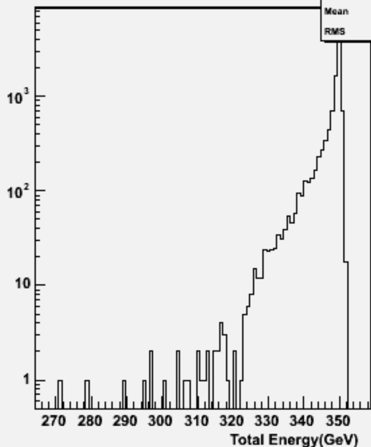
Pt Sum: w101017 ddn2e2e1n1_o
