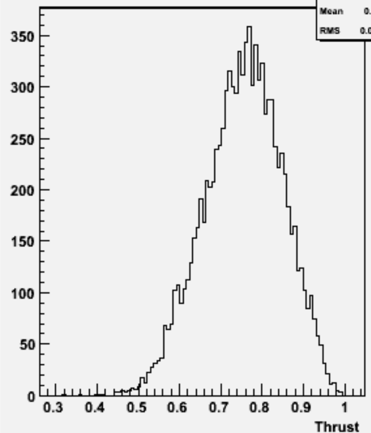
Thrust w101017 ddn2e2e1n1_o
